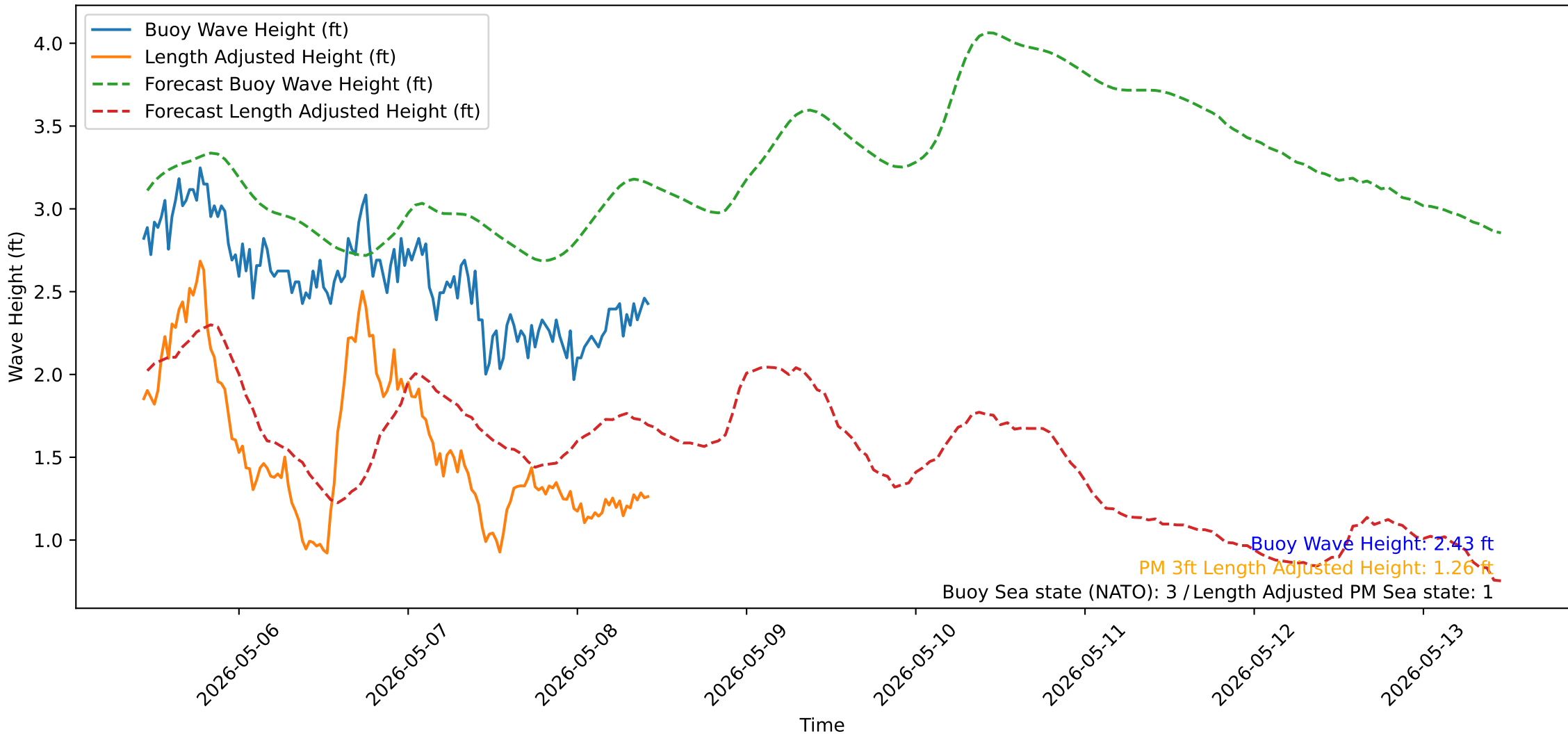
Wave Heights over Time for Oceanside Harbor at 2026-05-08 10:40:31
