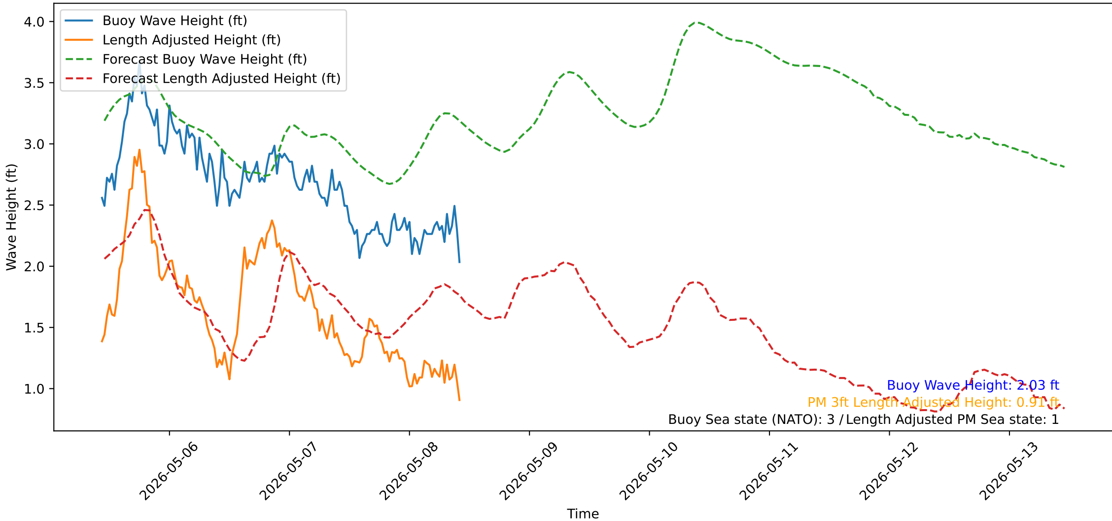
Wave Heights over Time for Green Beach at 2026-05-08 10:41:13
