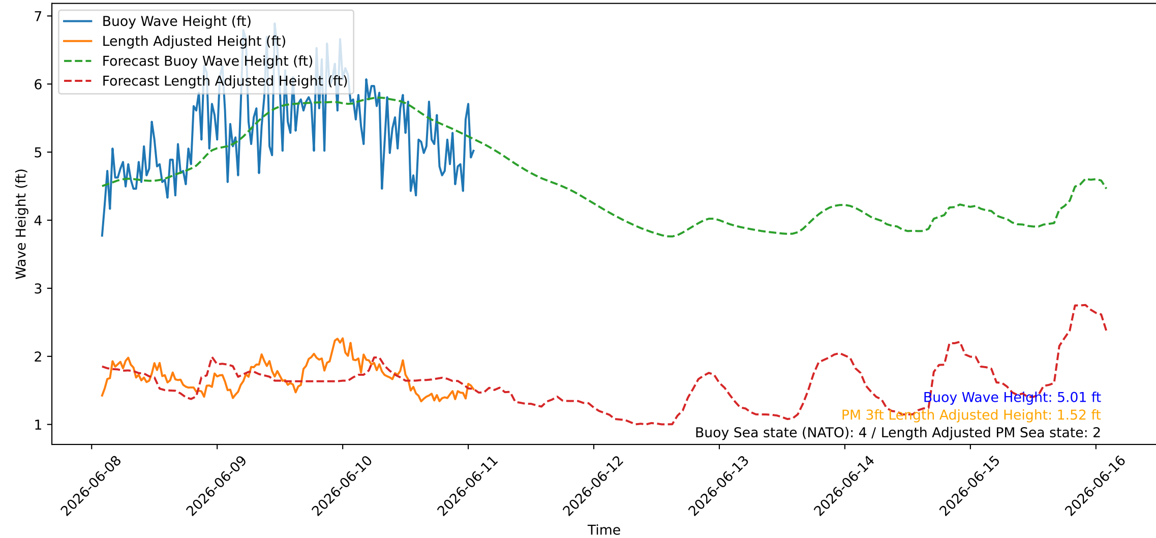
Wave Heights over Time for Green Beach at 2026-06-11 02:01:10
