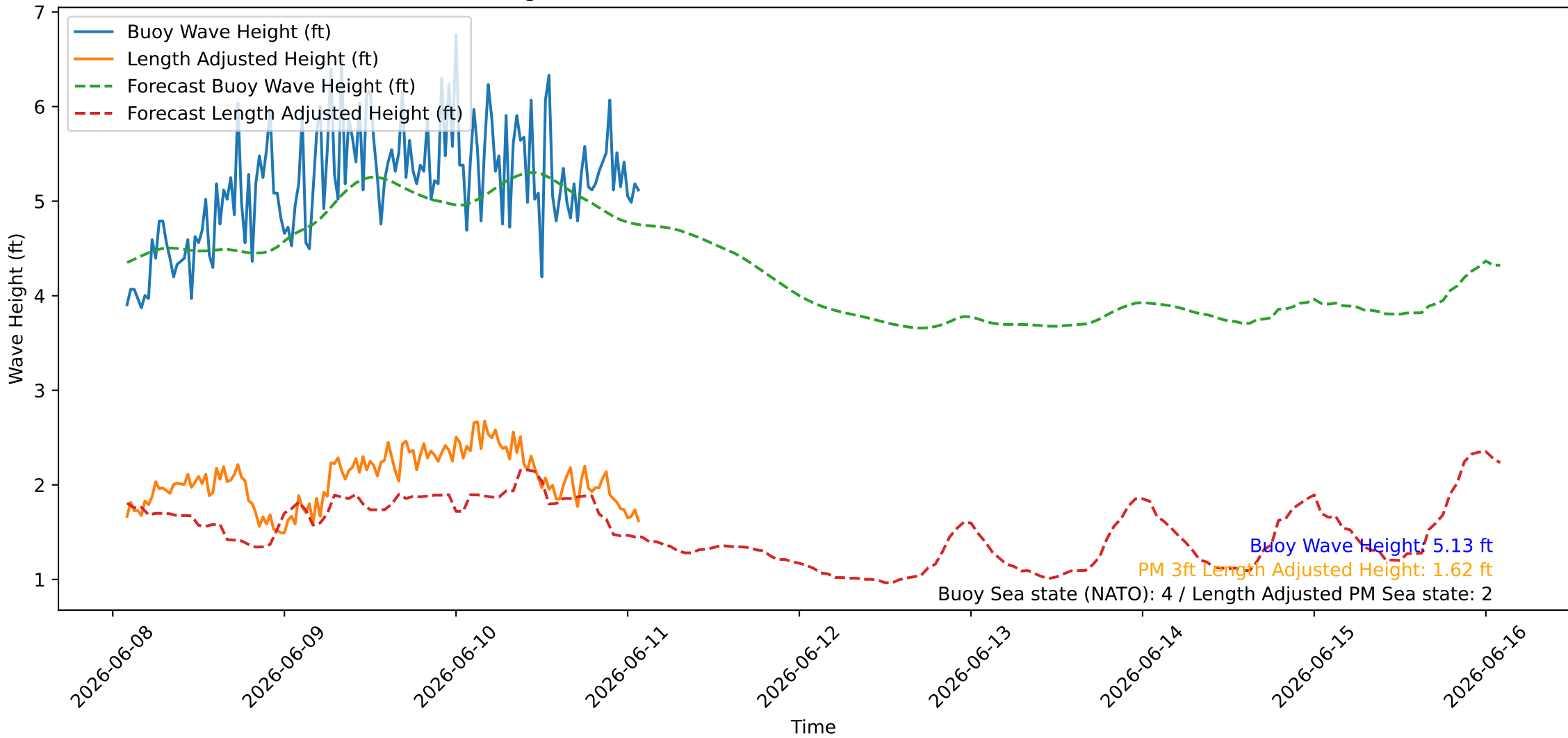
Wave Heights over Time for Oceanside Harbor at 2026-06-11 02:00:26
