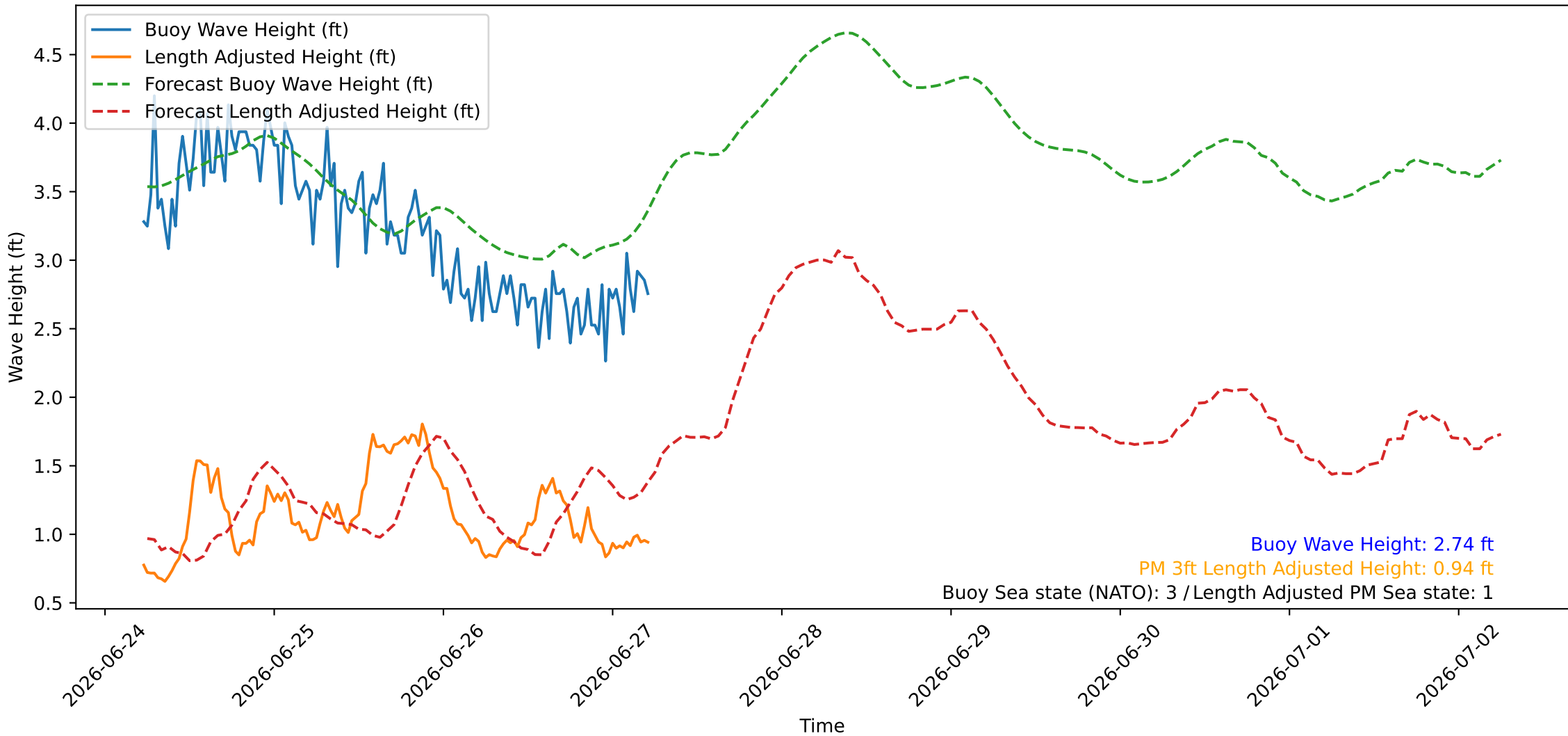
Wave Heights over Time for Green Beach at 2026-06-27 05:41:08
