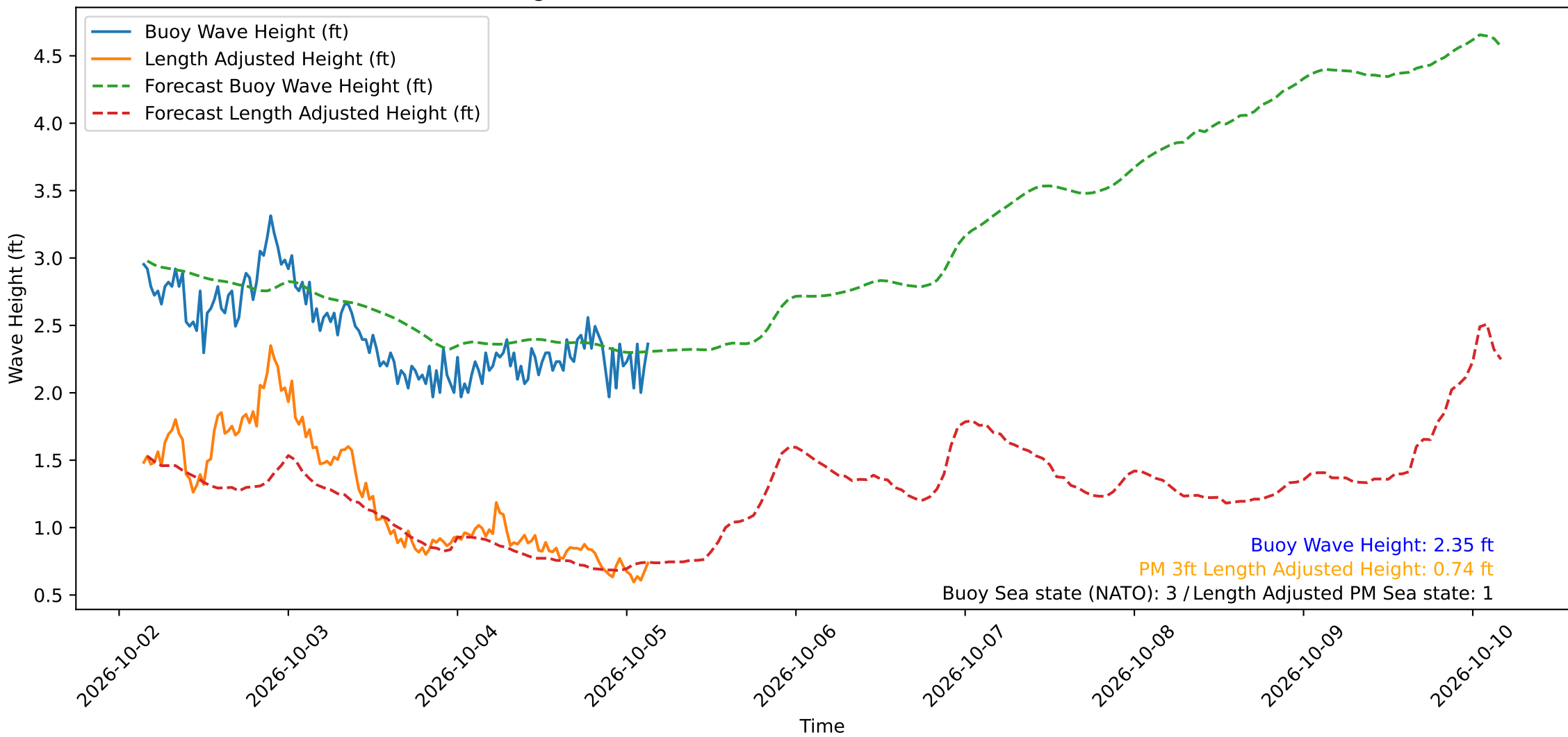
Wave Heights over Time for Oceanside Harbor at 2026-10-05 03:40:30
