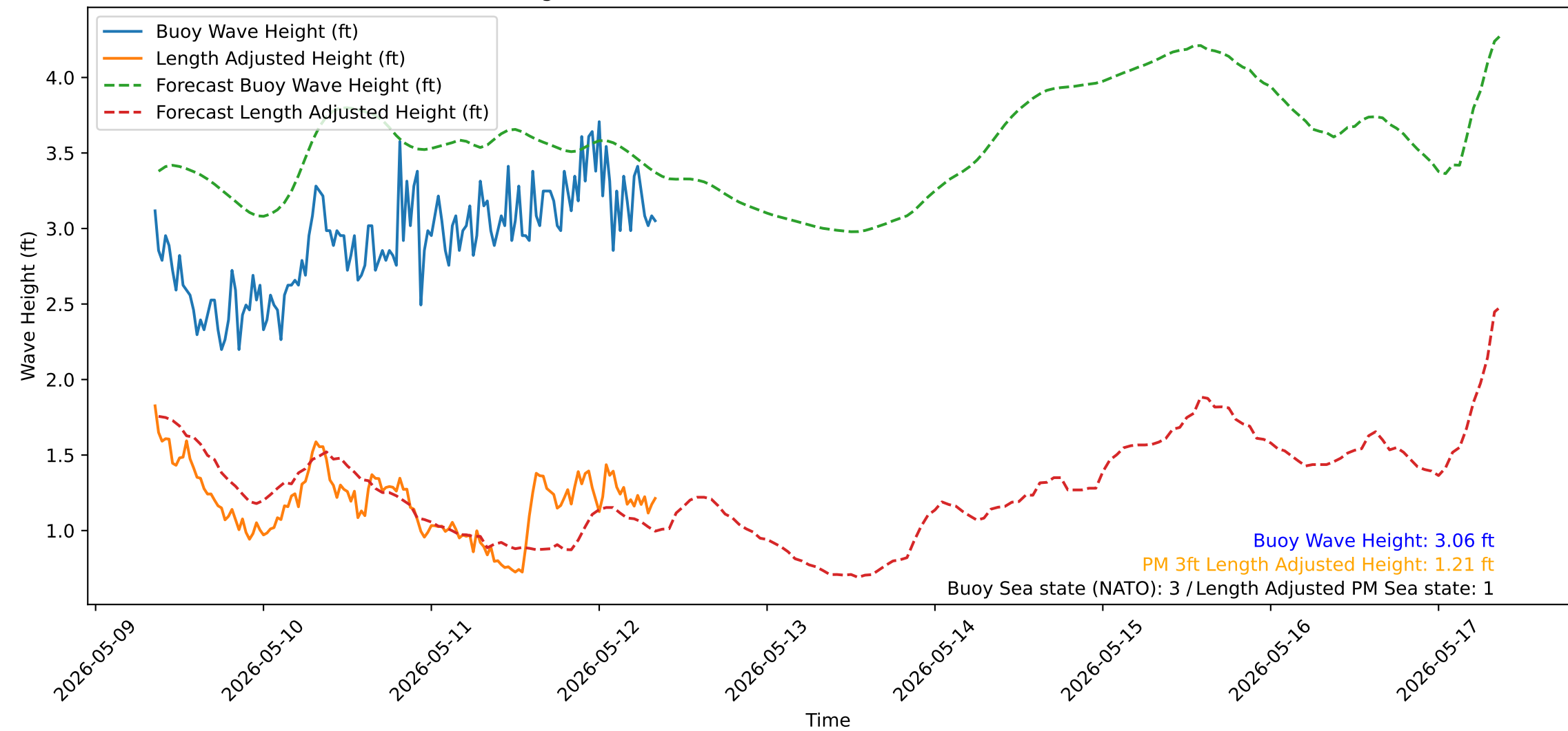
Wave Heights over Time for Oceanside Harbor at 2026-05-12 08:40:32
