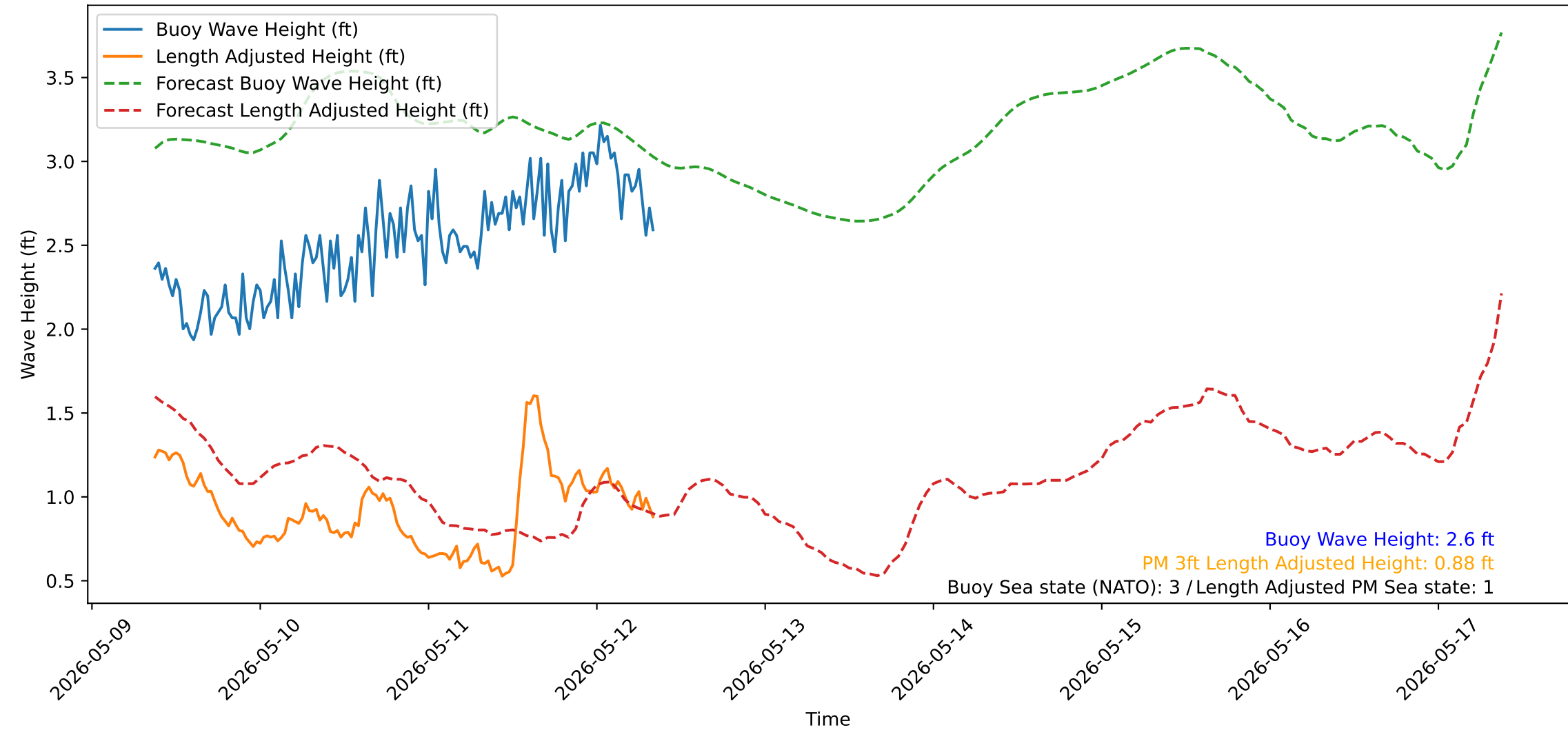
Wave Heights over Time for Red Beach at 2026-05-12 08:40:52
