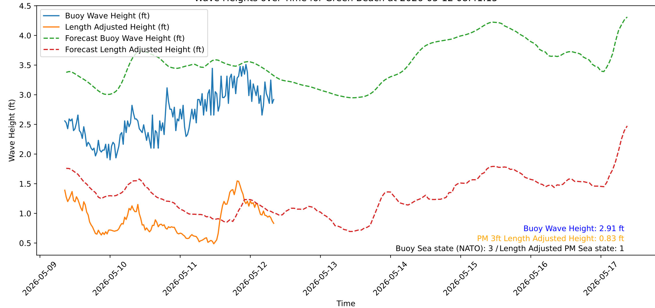
Wave Heights over Time for Green Beach at 2026-05-12 08:41:15
