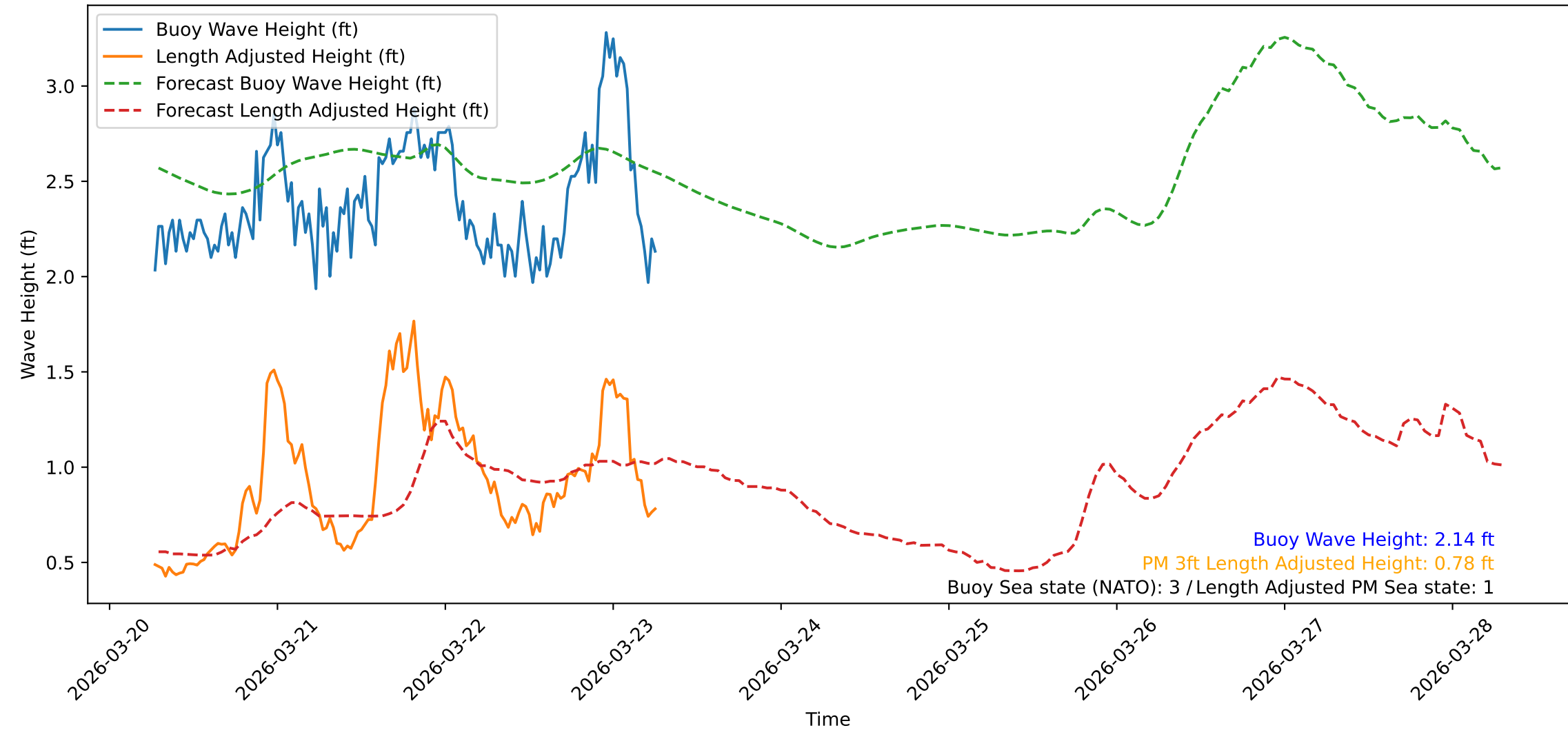
Wave Heights over Time for Green Beach at 2026-03-23 06:41:09
