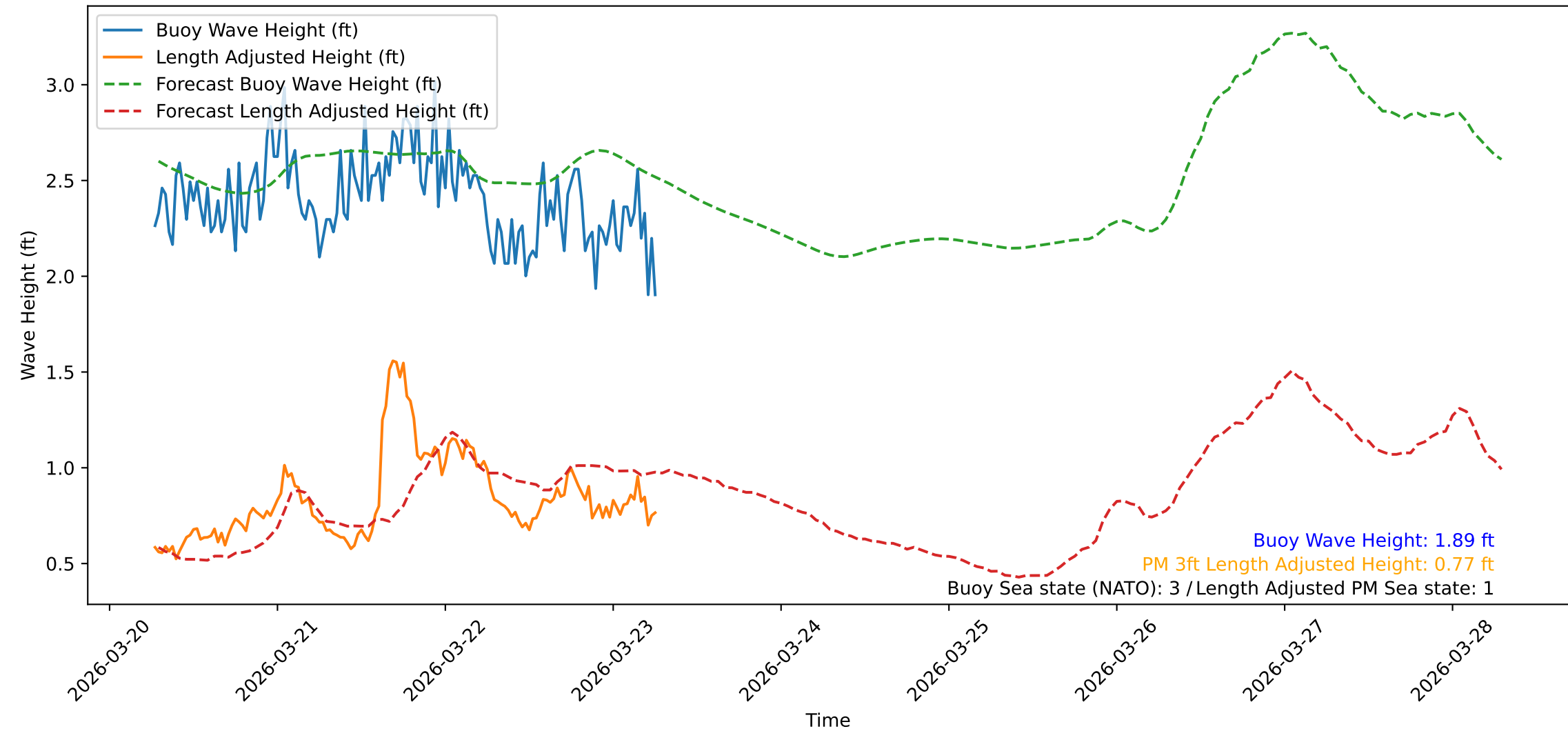
Wave Heights over Time for Oceanside Harbor at 2026-03-23 06:40:31
