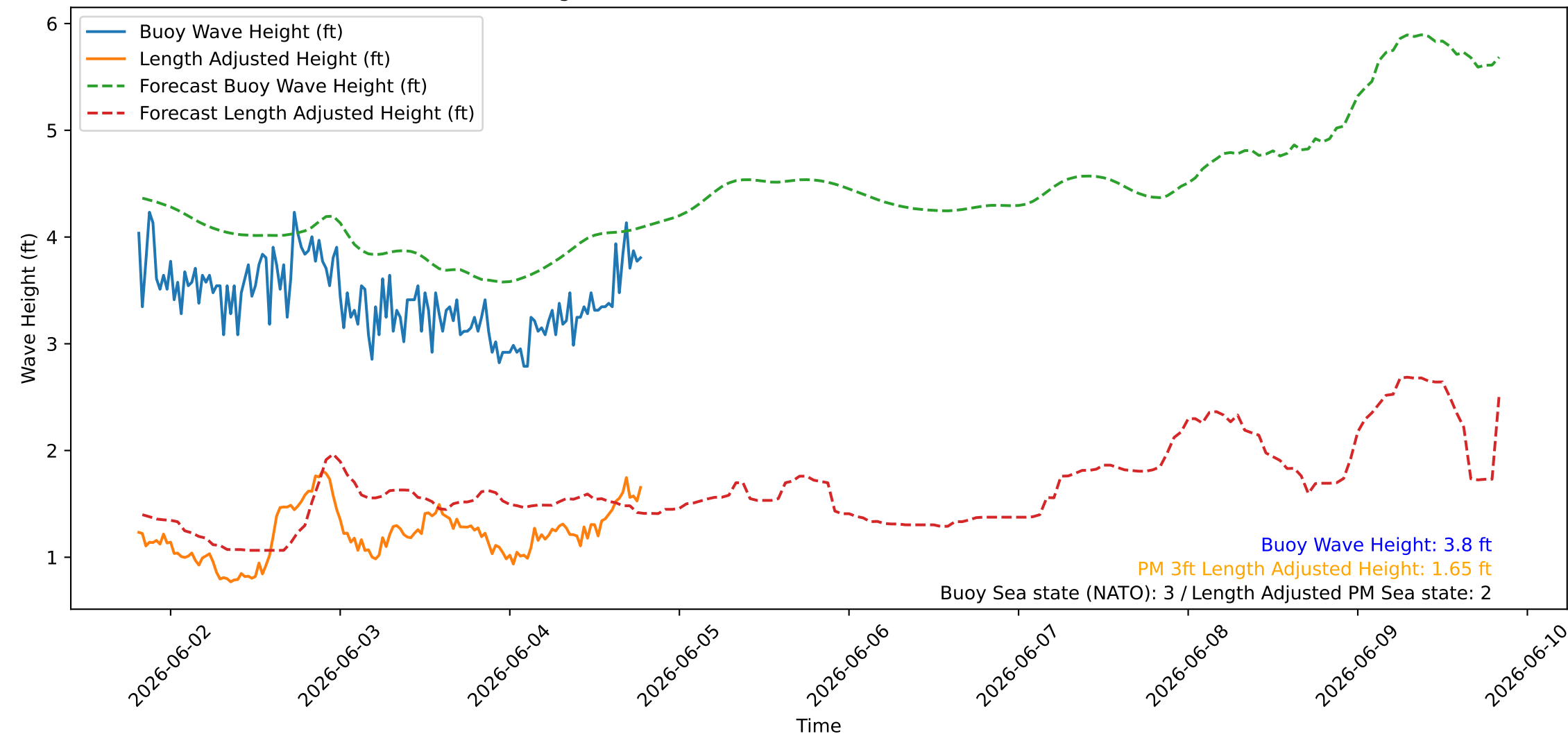
Wave Heights over Time for Green Beach at 2026-06-04 19:41:07
