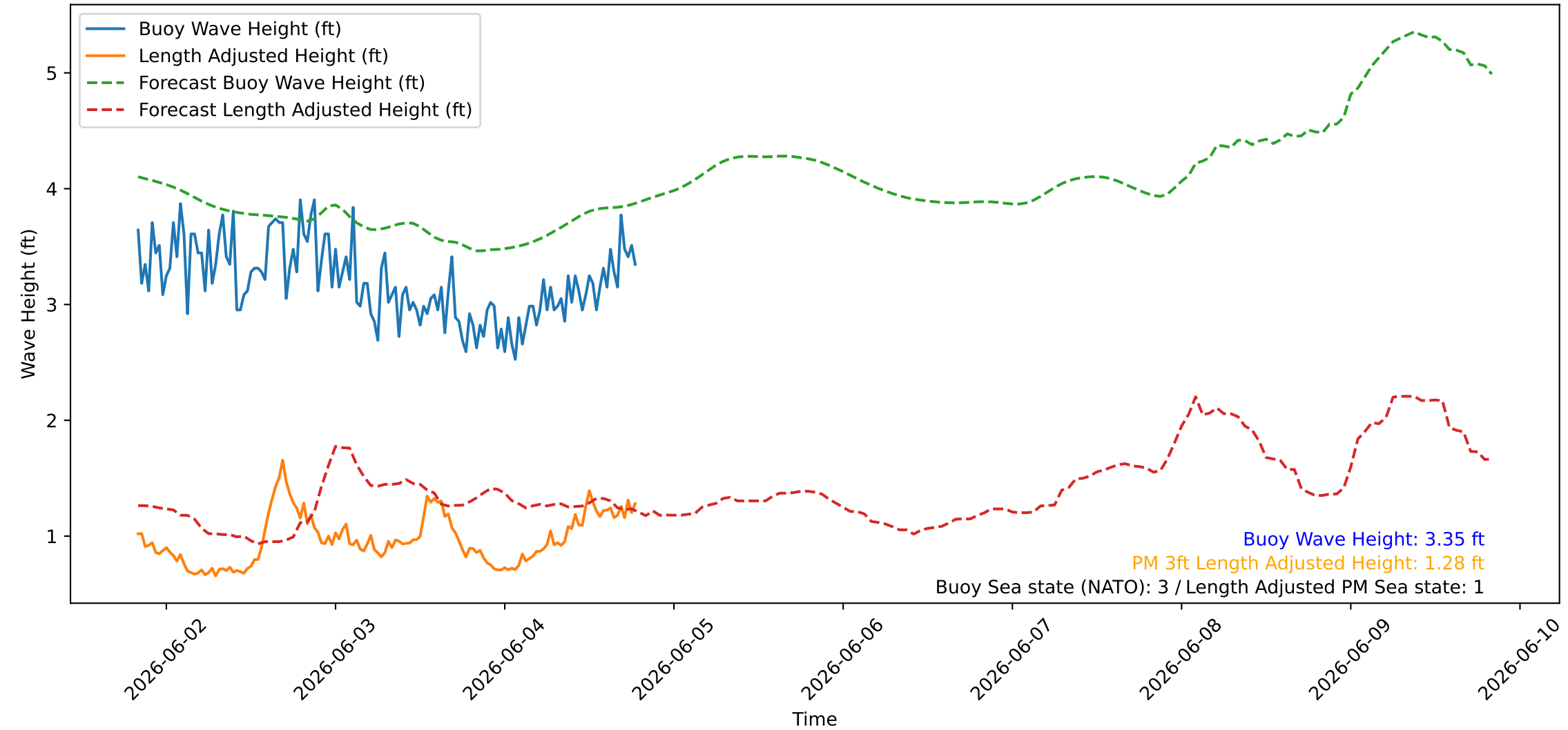
Wave Heights over Time for Red Beach at 2026-06-04 19:40:45
