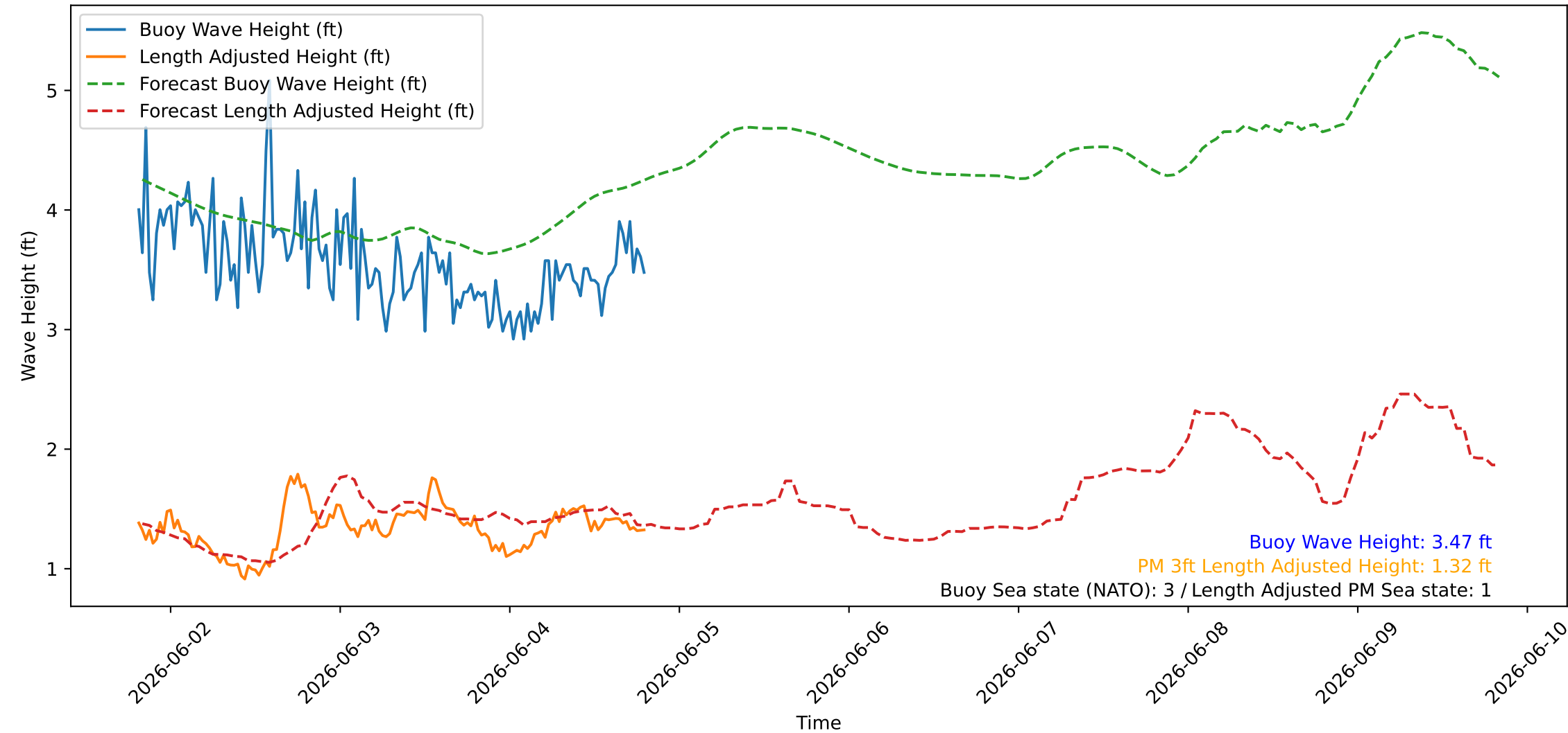
Wave Heights over Time for Oceanside Harbor at 2026-06-04 19:40:26
