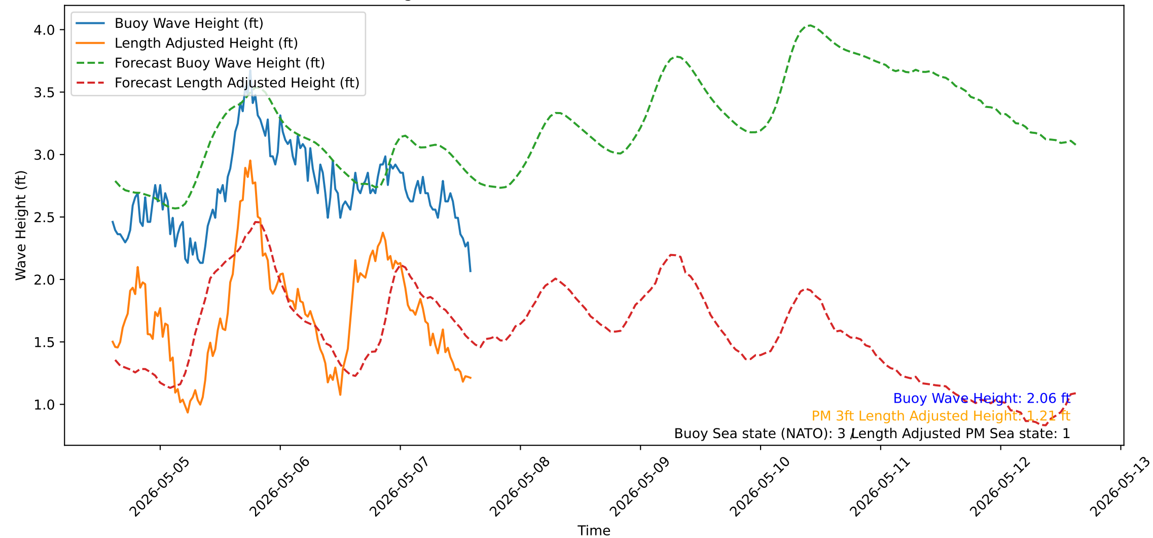
Wave Heights over Time for Green Beach at 2026-05-07 14:41:12
