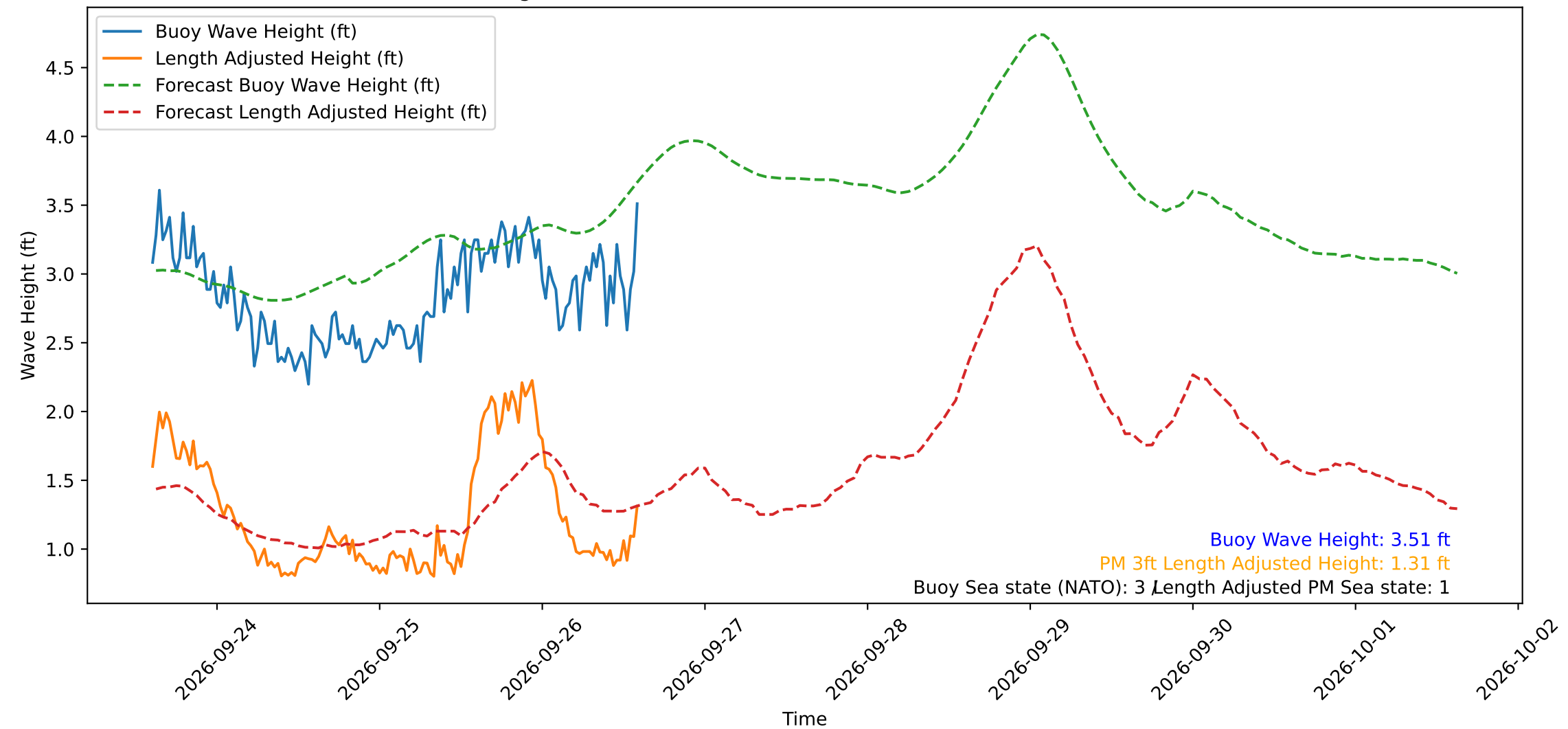
Wave Heights over Time for Oceanside Harbor at 2026-09-26 14:40:30
