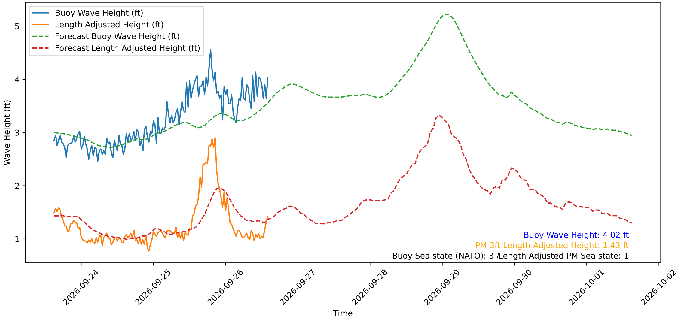
Wave Heights over Time for Green Beach at 2026-09-26 14:41:13
