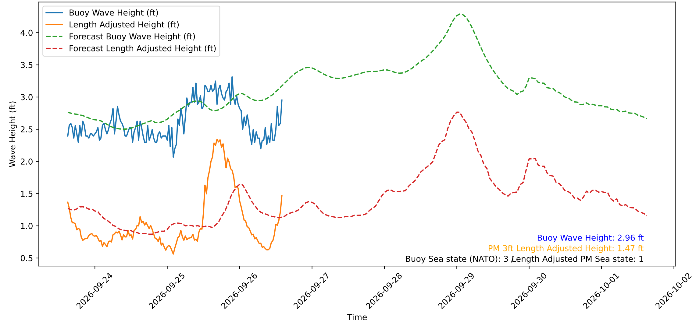
Wave Heights over Time for Red Beach at 2026-09-26 14:40:50
