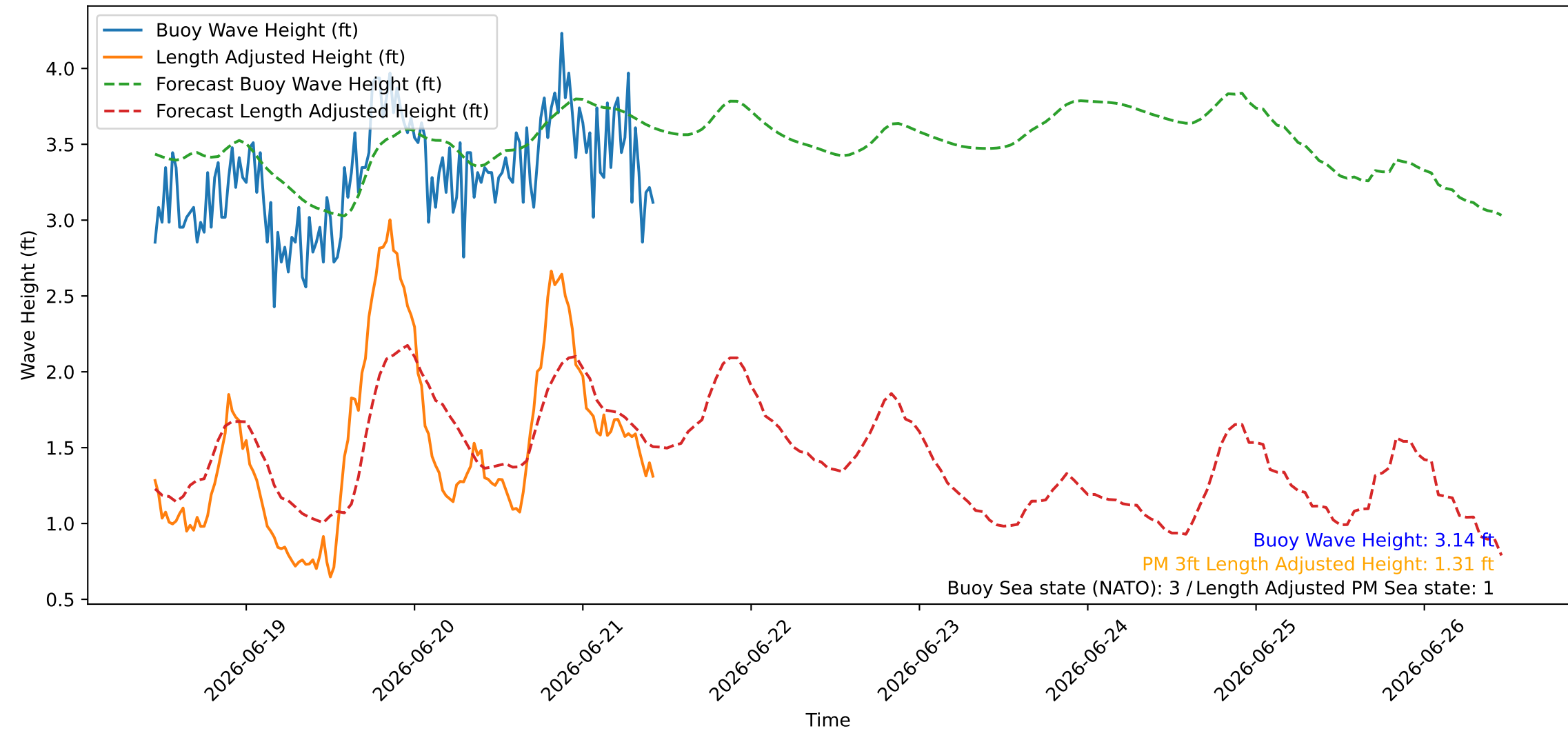
Wave Heights over Time for Green Beach at 2026-06-21 10:51:09
