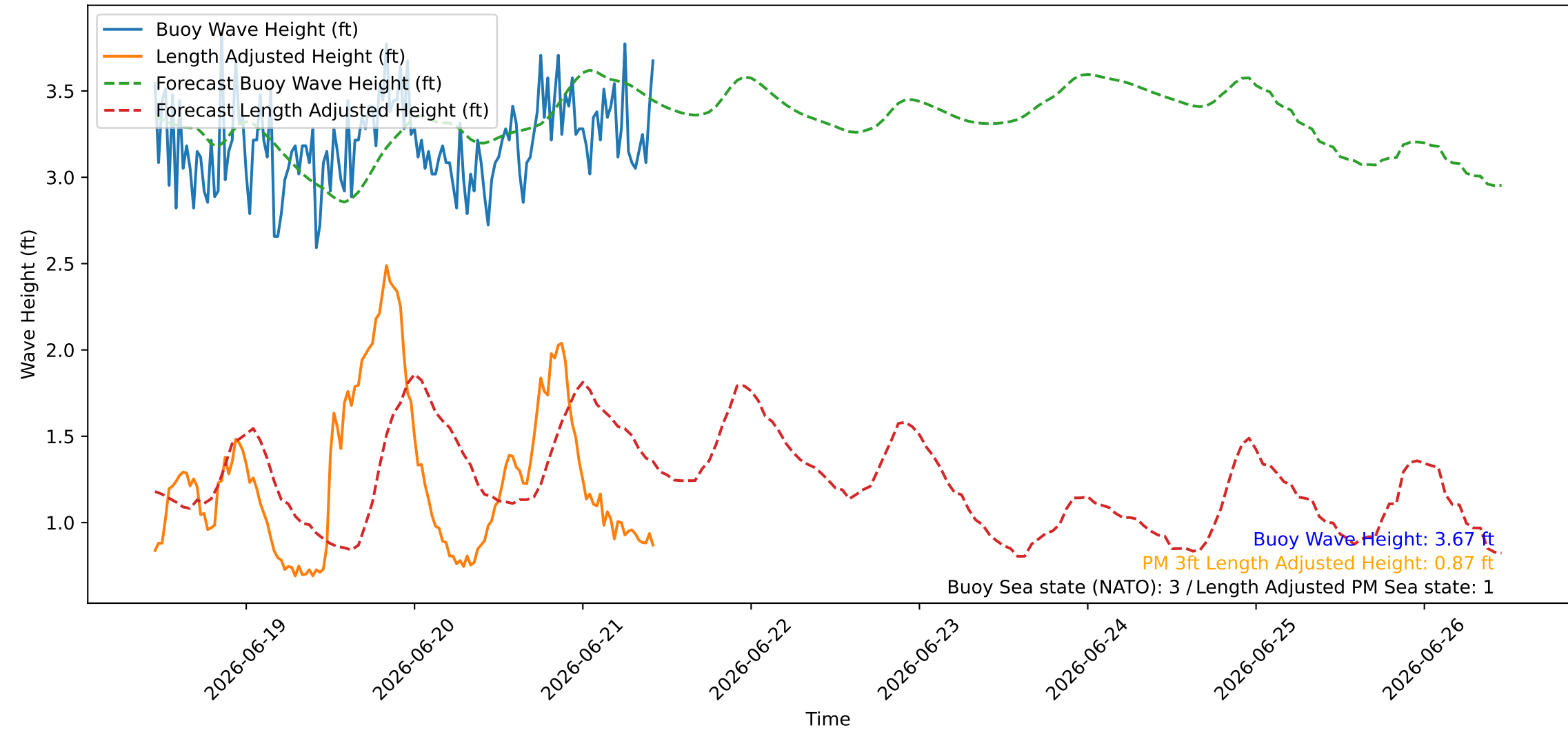
Wave Heights over Time for Red Beach at 2026-06-21 10:50:46
