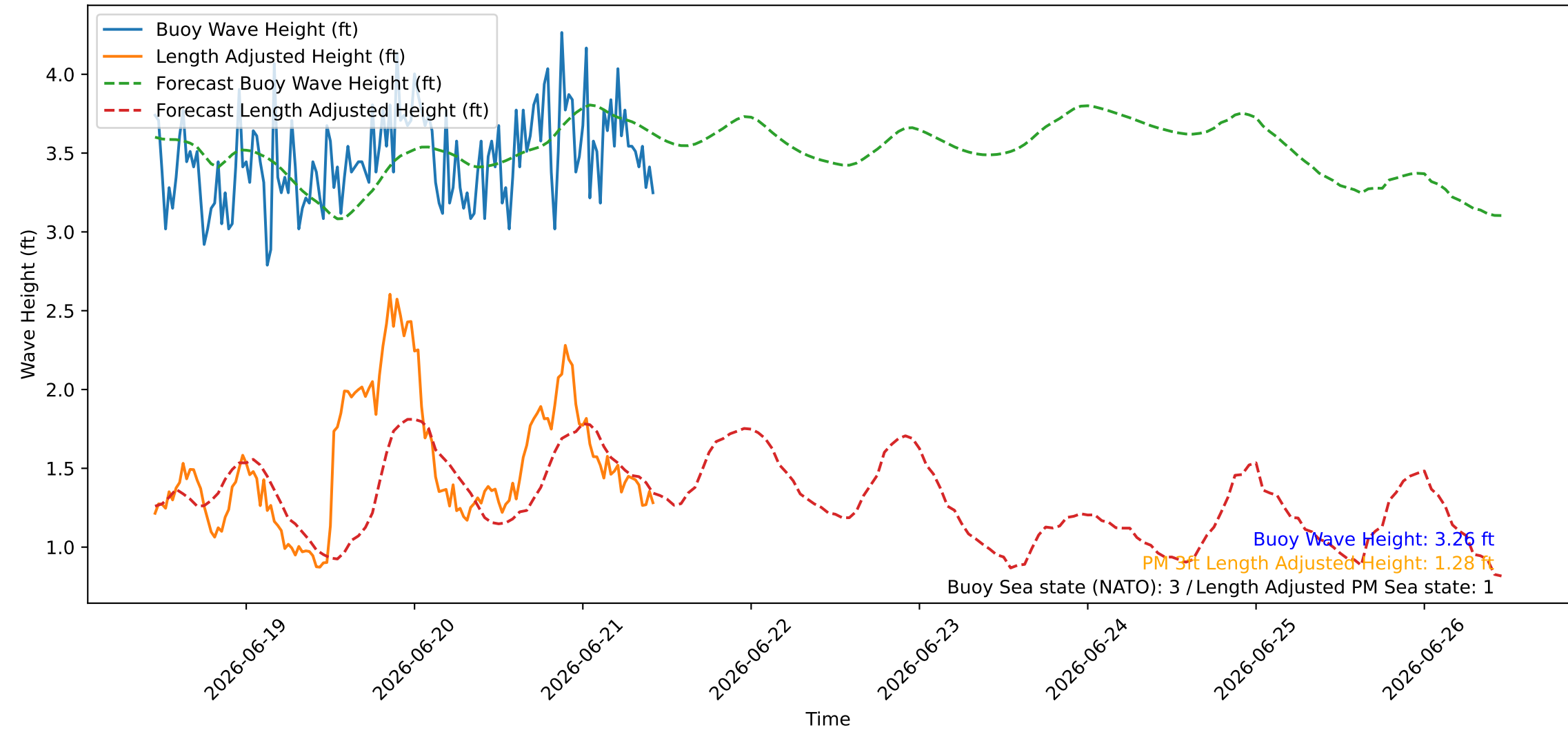
Wave Heights over Time for Oceanside Harbor at 2026-06-21 10:50:26
