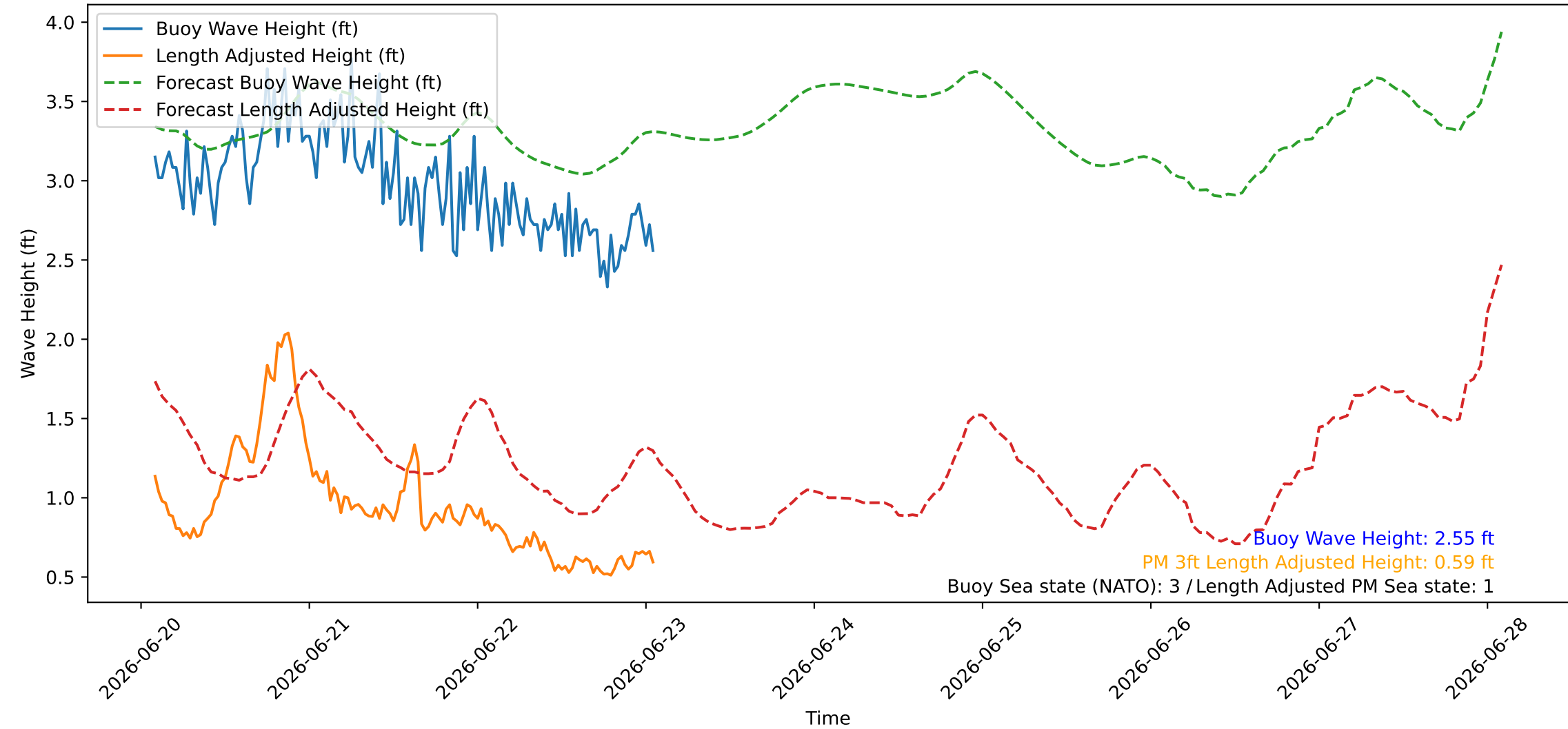
Wave Heights over Time for Red Beach at 2026-06-23 01:50:47
