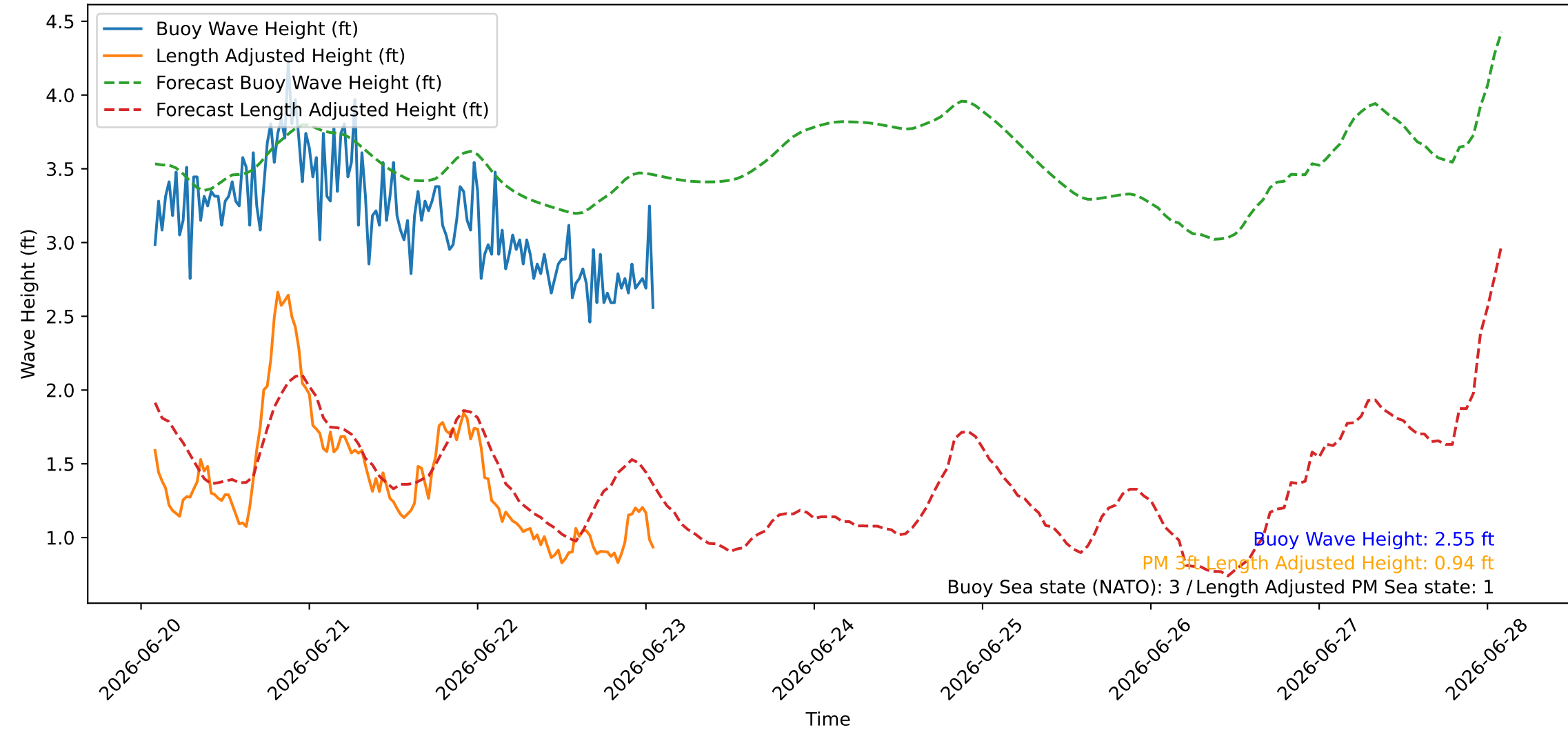
Wave Heights over Time for Green Beach at 2026-06-23 01:51:09
