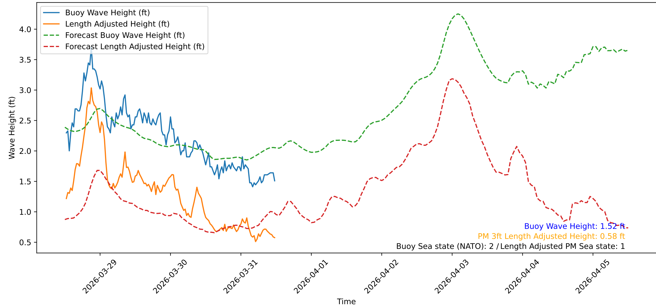
Wave Heights over Time for Green Beach at 2026-03-31 12:21:09
