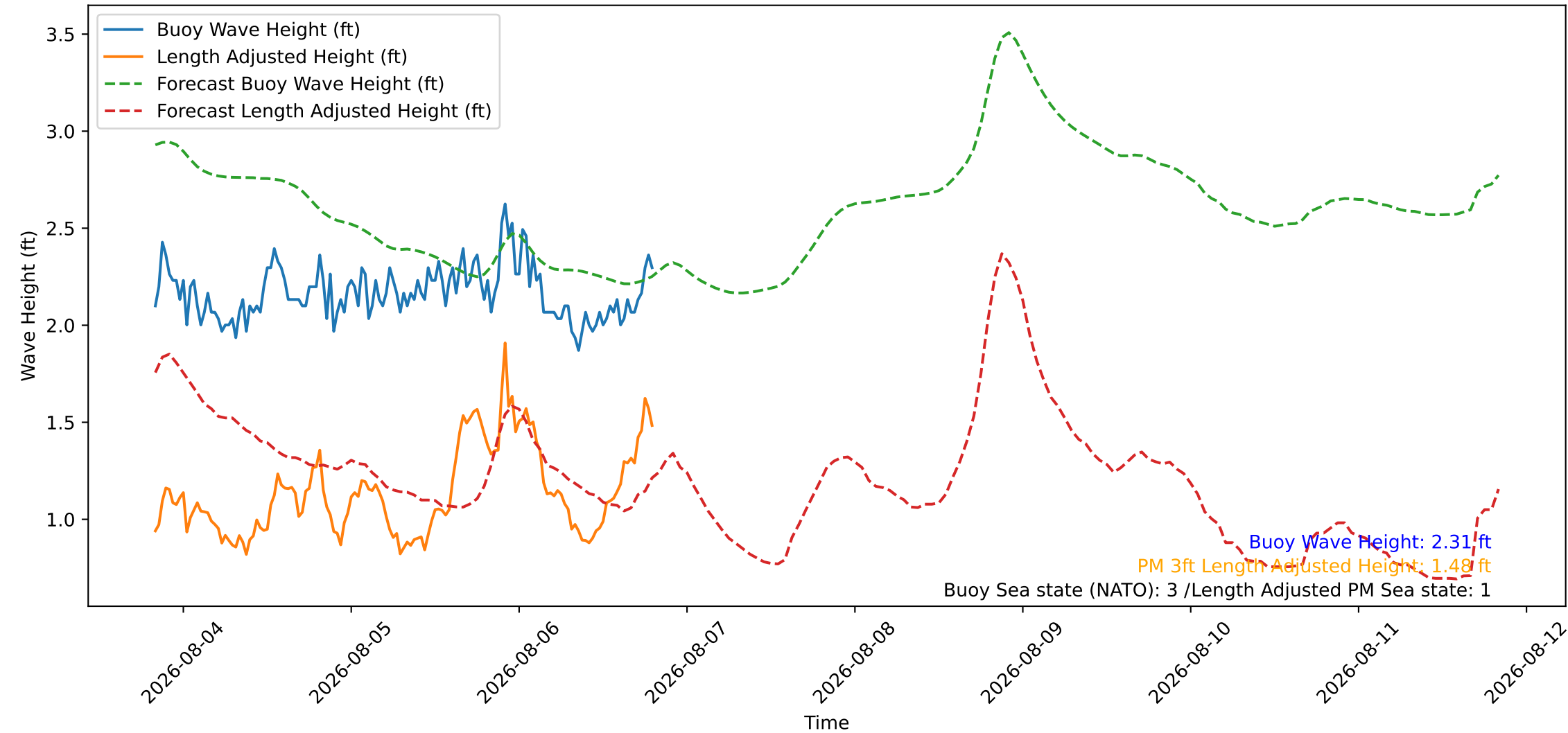
Wave Heights over Time for Green Beach at 2026-08-06 19:51:09
