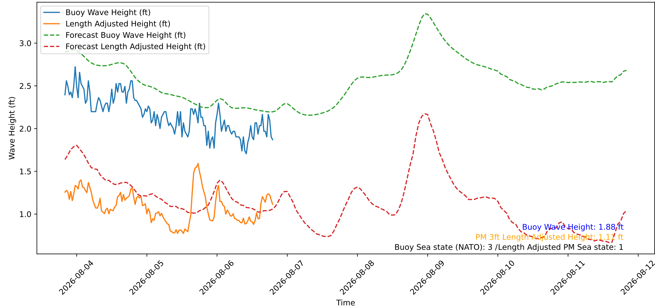
Wave Heights over Time for Oceanside Harbor at 2026-08-06 19:50:26
