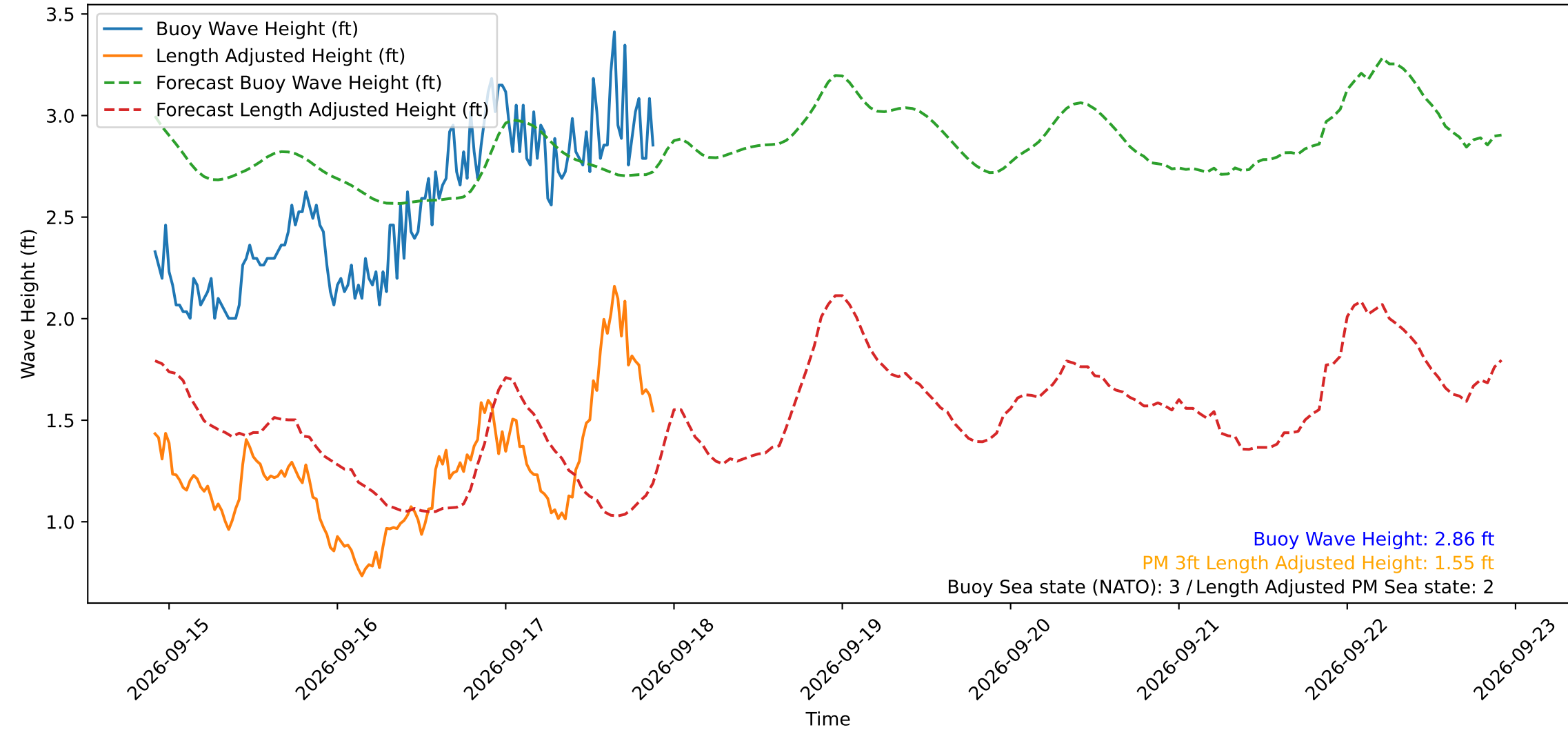
Wave Heights over Time for Red Beach at 2026-09-17 21:50:49
