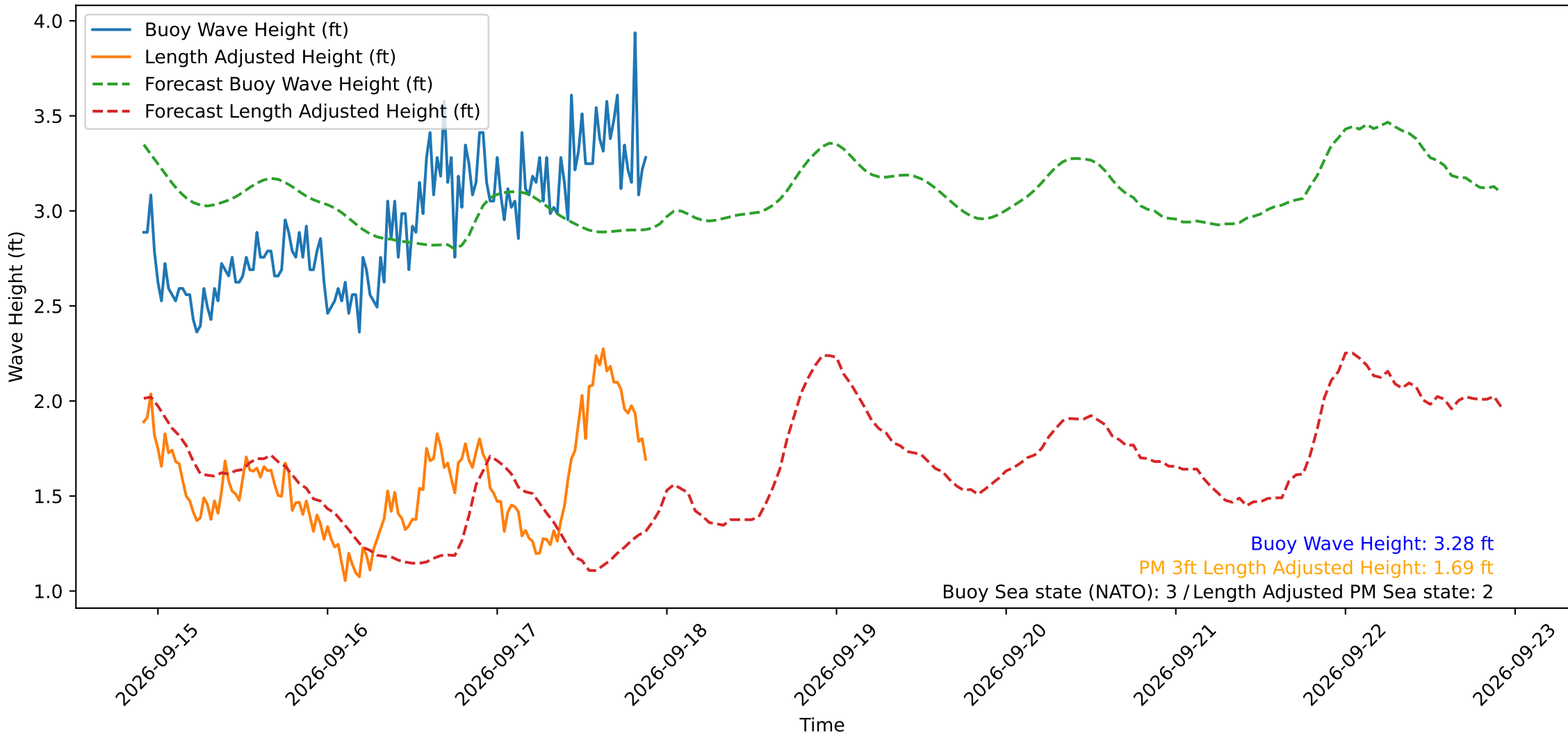
Wave Heights over Time for Oceanside Harbor at 2026-09-17 21:50:29
