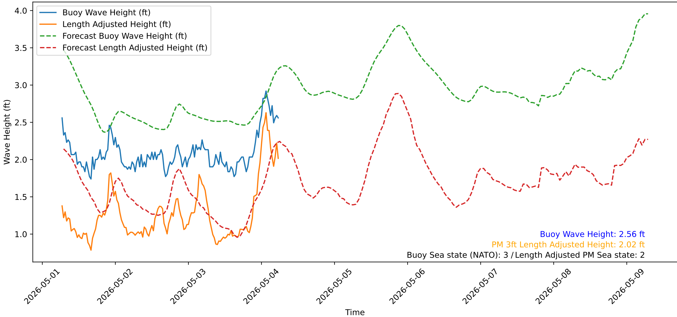
Wave Heights over Time for Green Beach at 2026-05-04 06:31:13
