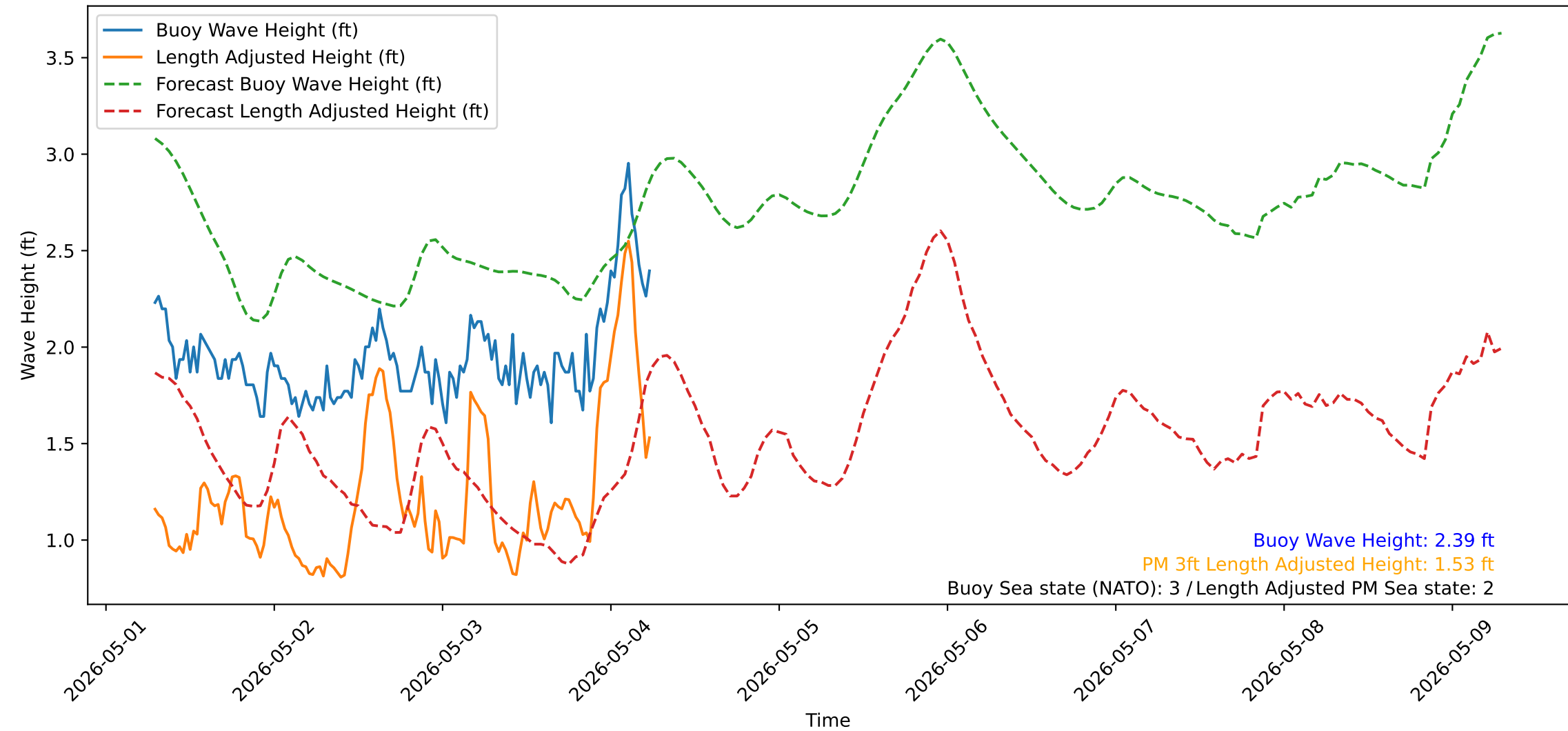
Wave Heights over Time for Red Beach at 2026-05-04 06:30:51
