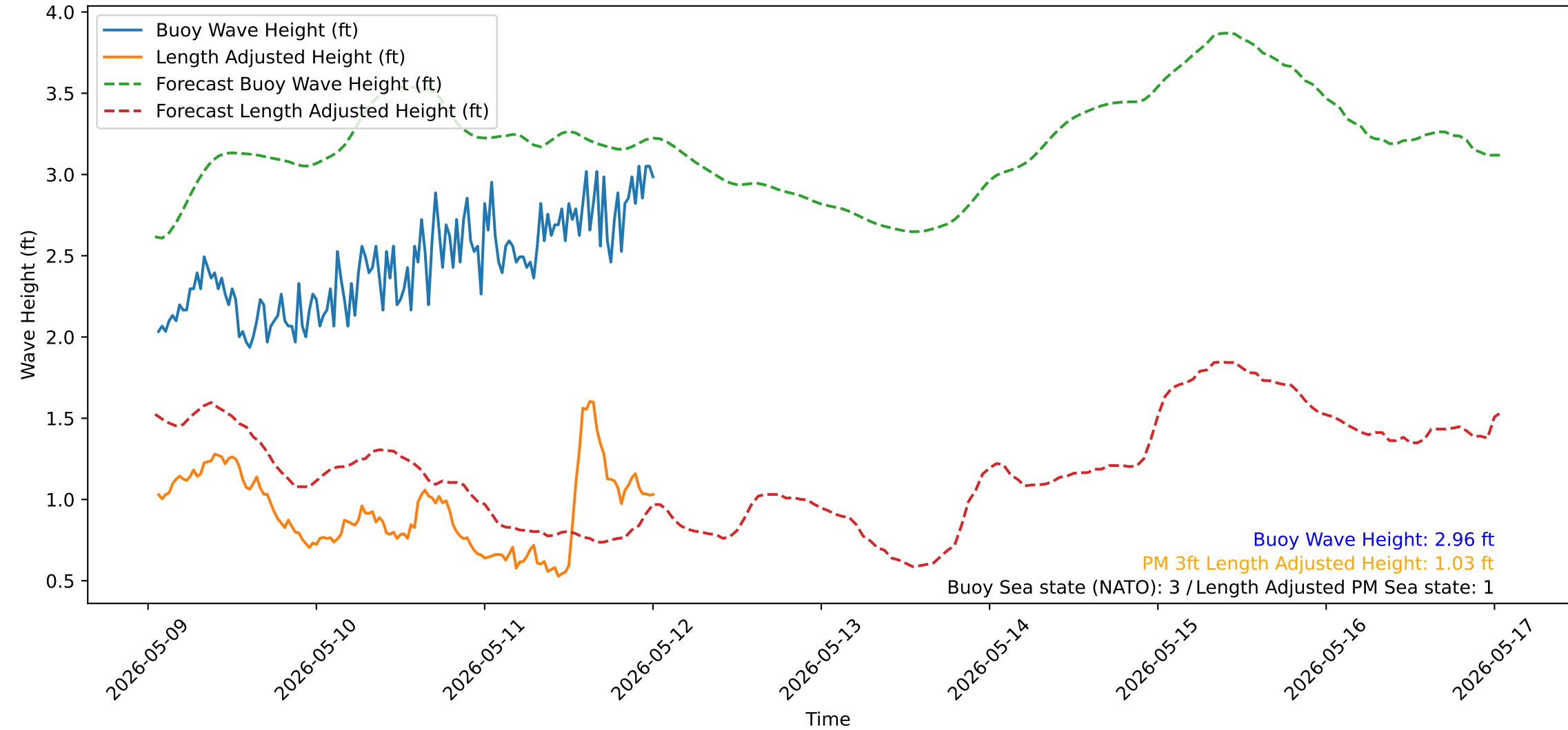
Wave Heights over Time for Red Beach at 2026-05-12 01:00:51
