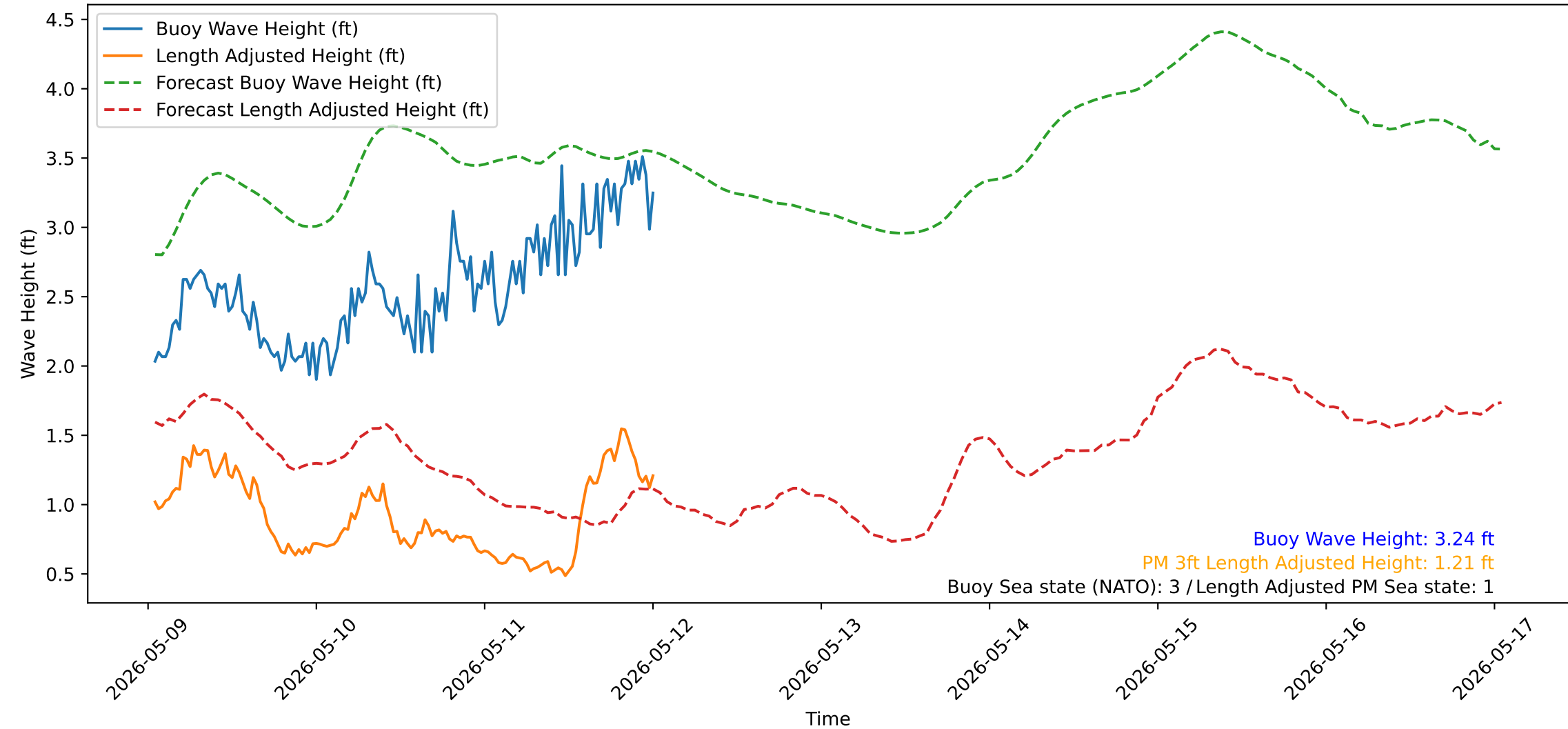
Wave Heights over Time for Green Beach at 2026-05-12 01:01:13
