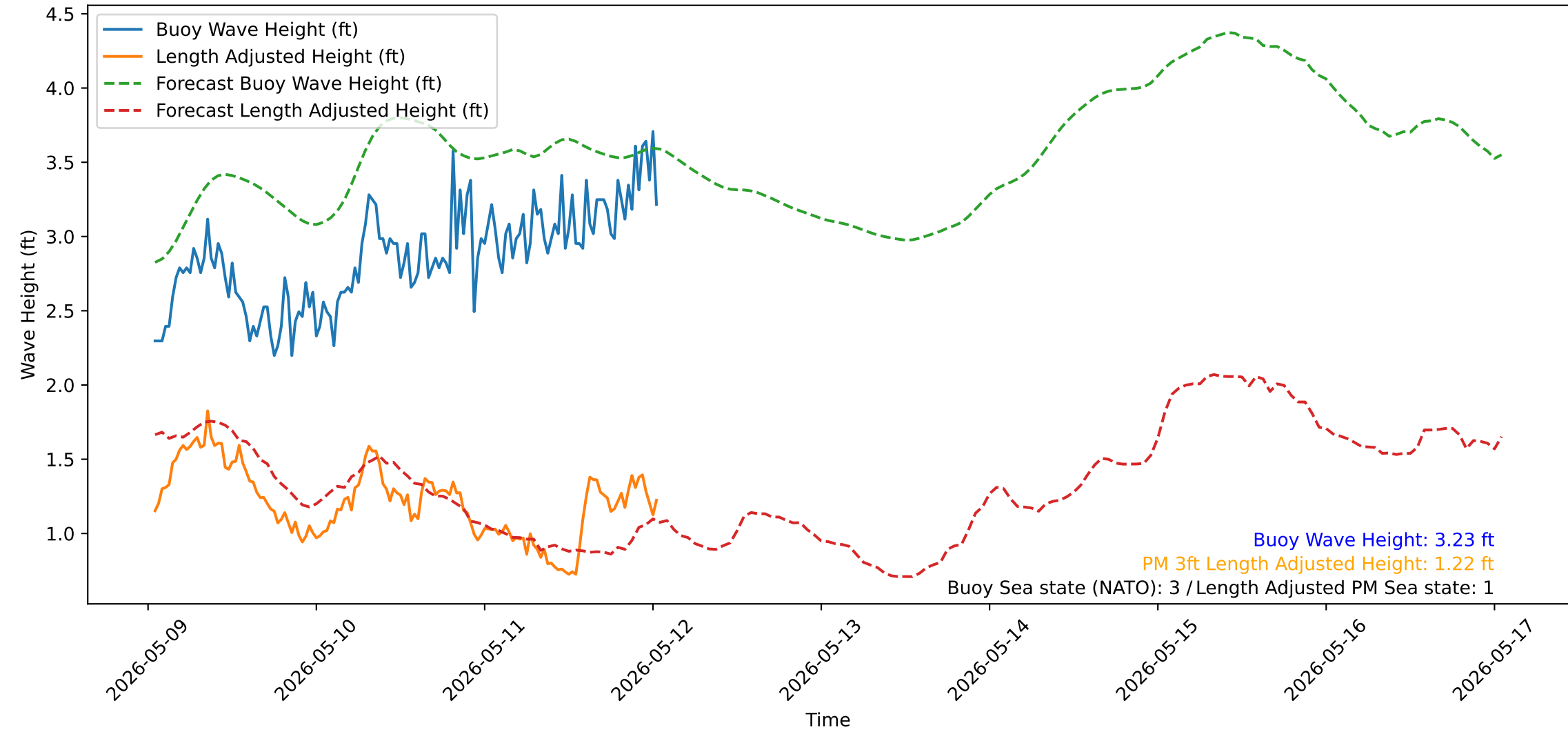
Wave Heights over Time for Oceanside Harbor at 2026-05-12 01:00:32
