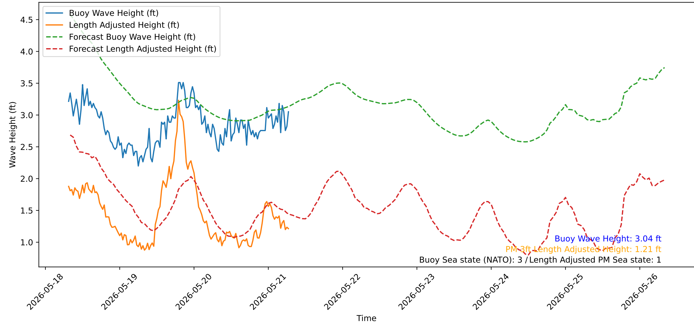
Wave Heights over Time for Oceanside Harbor at 2026-05-21 07:40:31
