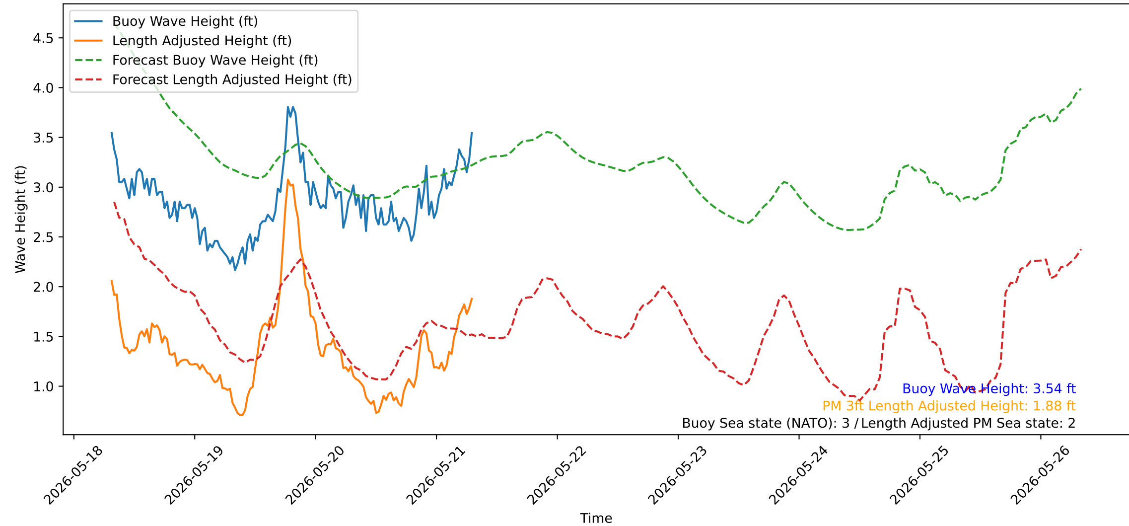
Wave Heights over Time for Green Beach at 2026-05-21 07:41:13
