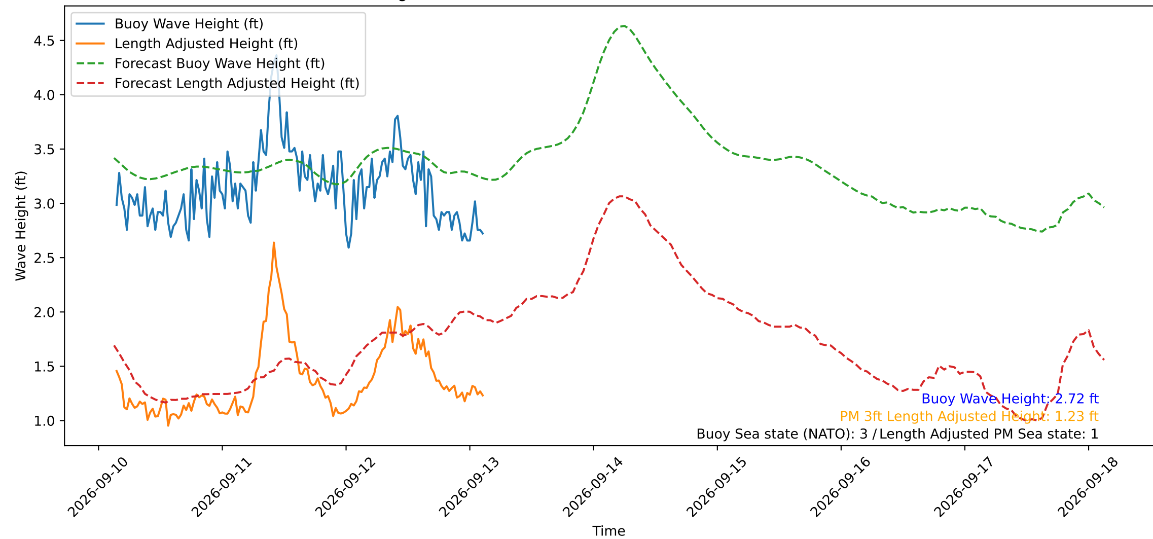
Wave Heights over Time for Oceanside Harbor at 2026-09-13 03:20:30
