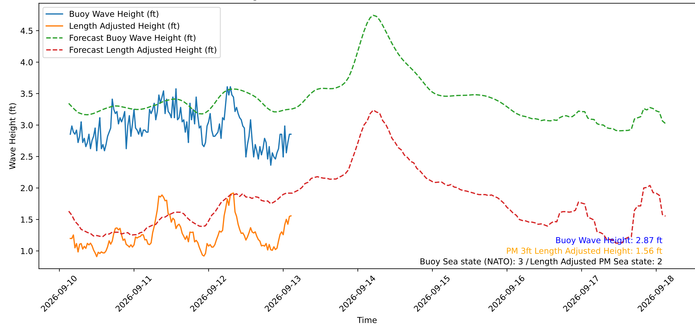
Wave Heights over Time for Green Beach at 2026-09-13 03:21:15
