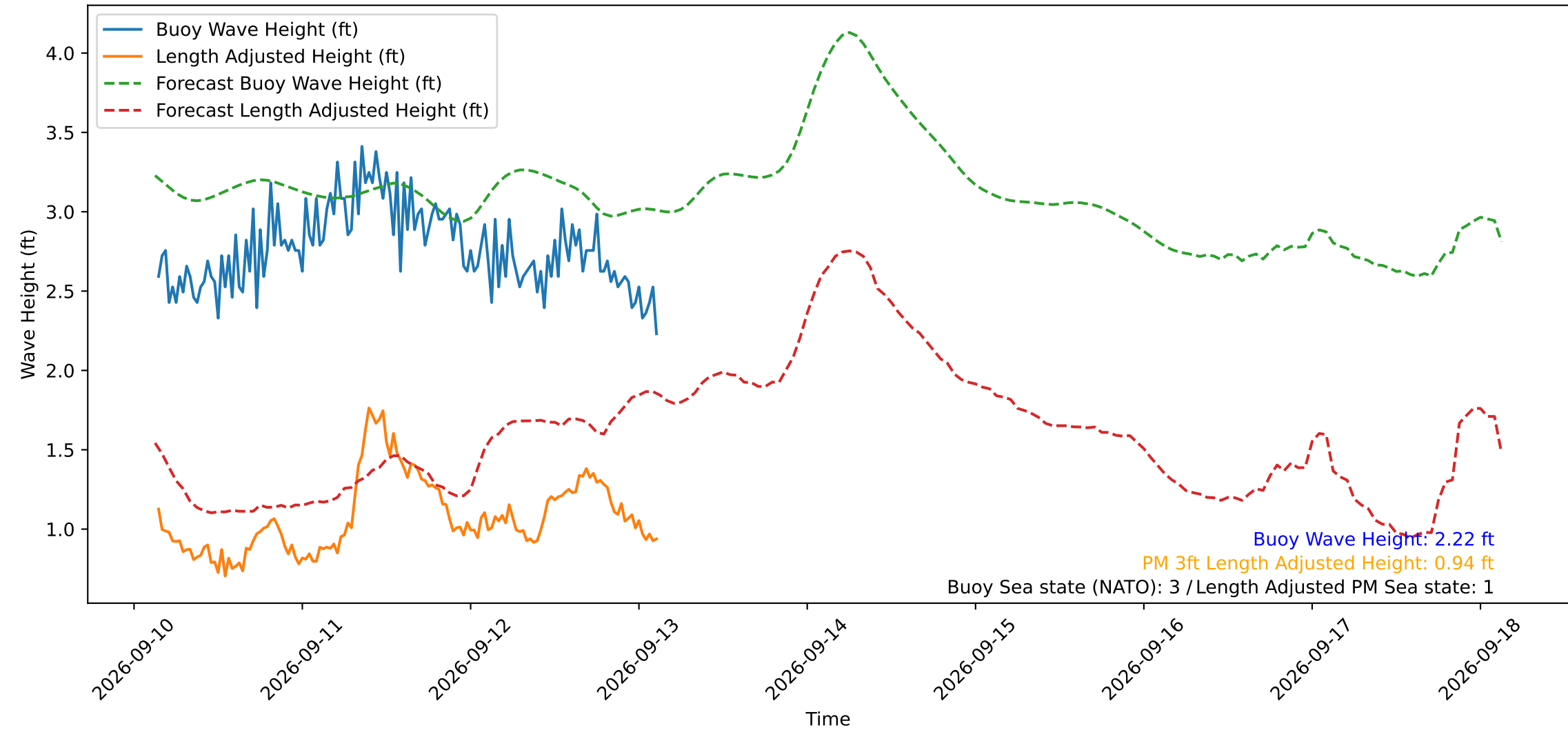
Wave Heights over Time for Red Beach at 2026-09-13 03:20:51
