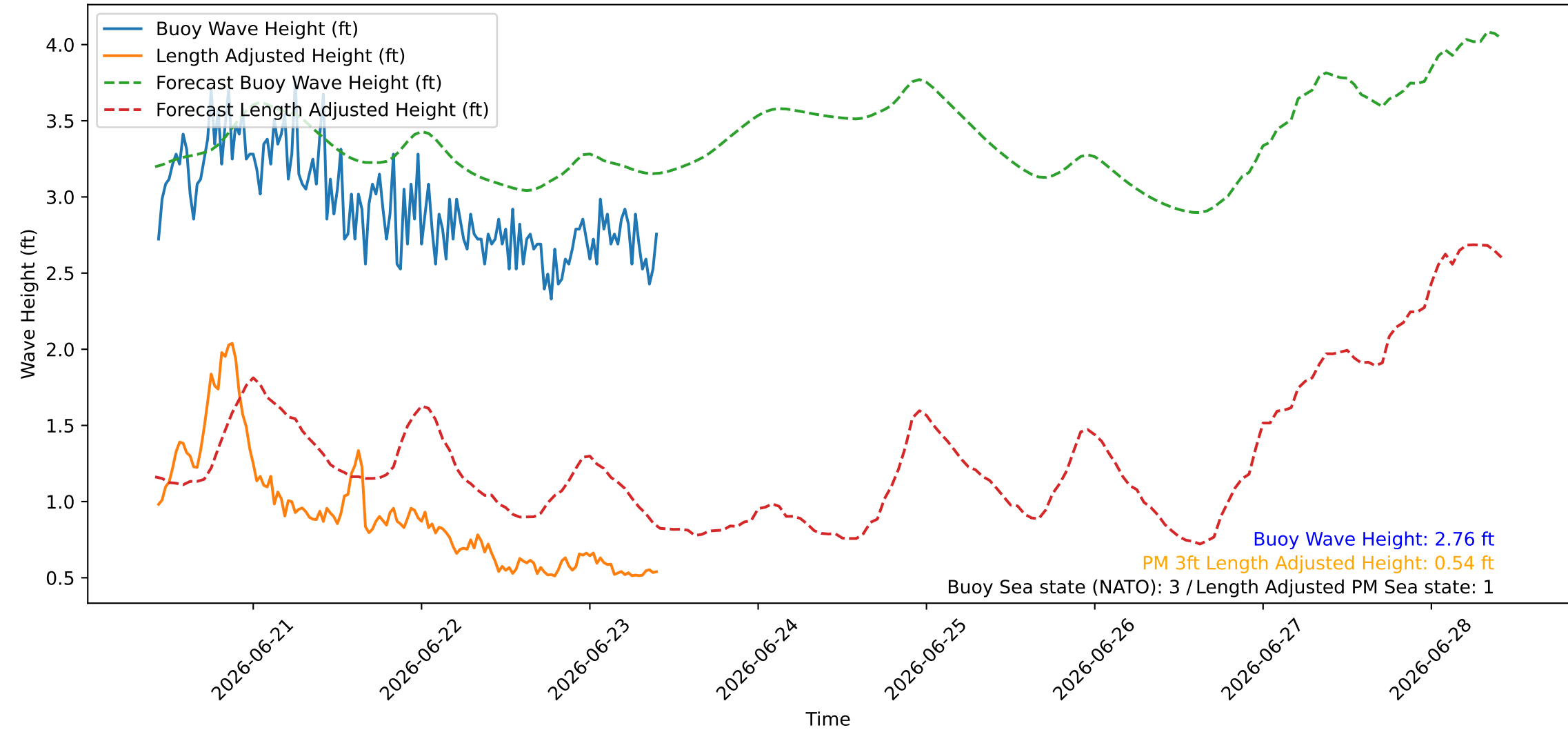
Wave Heights over Time for Red Beach at 2026-06-23 10:20:47
