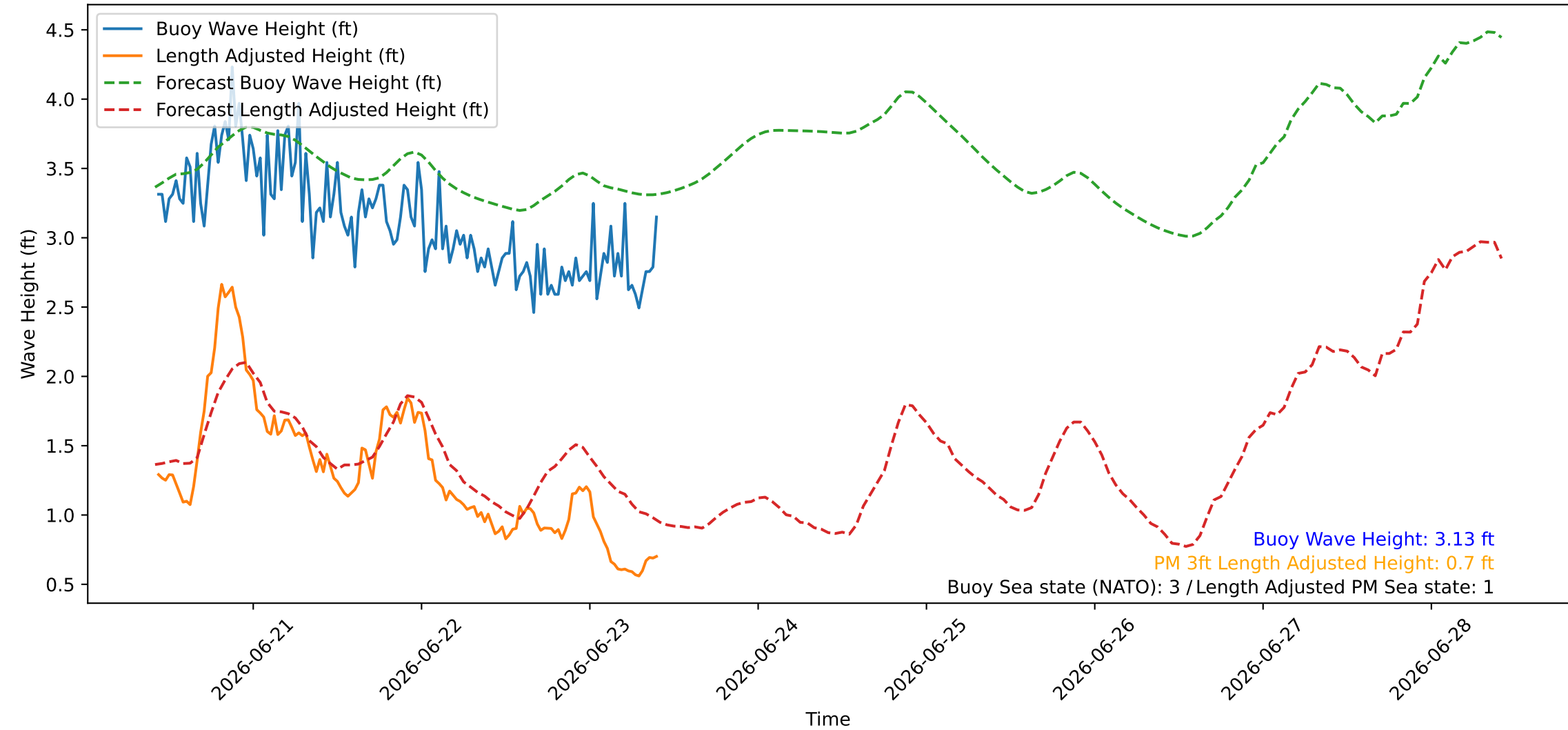
Wave Heights over Time for Green Beach at 2026-06-23 10:21:09
