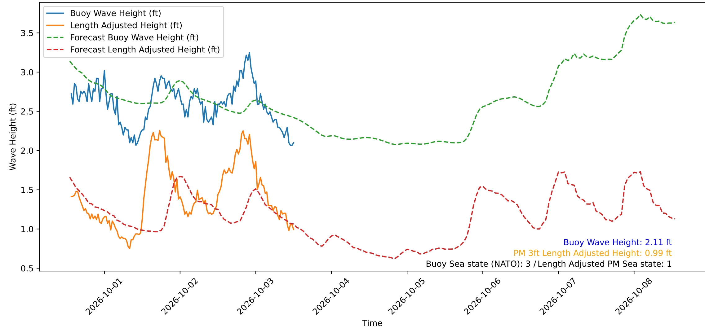
Wave Heights over Time for Red Beach at 2026-10-03 13:00:50
