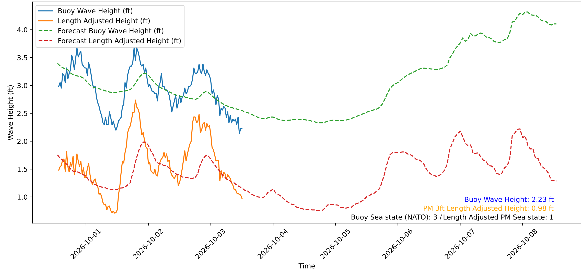
Wave Heights over Time for Green Beach at 2026-10-03 13:01:12
