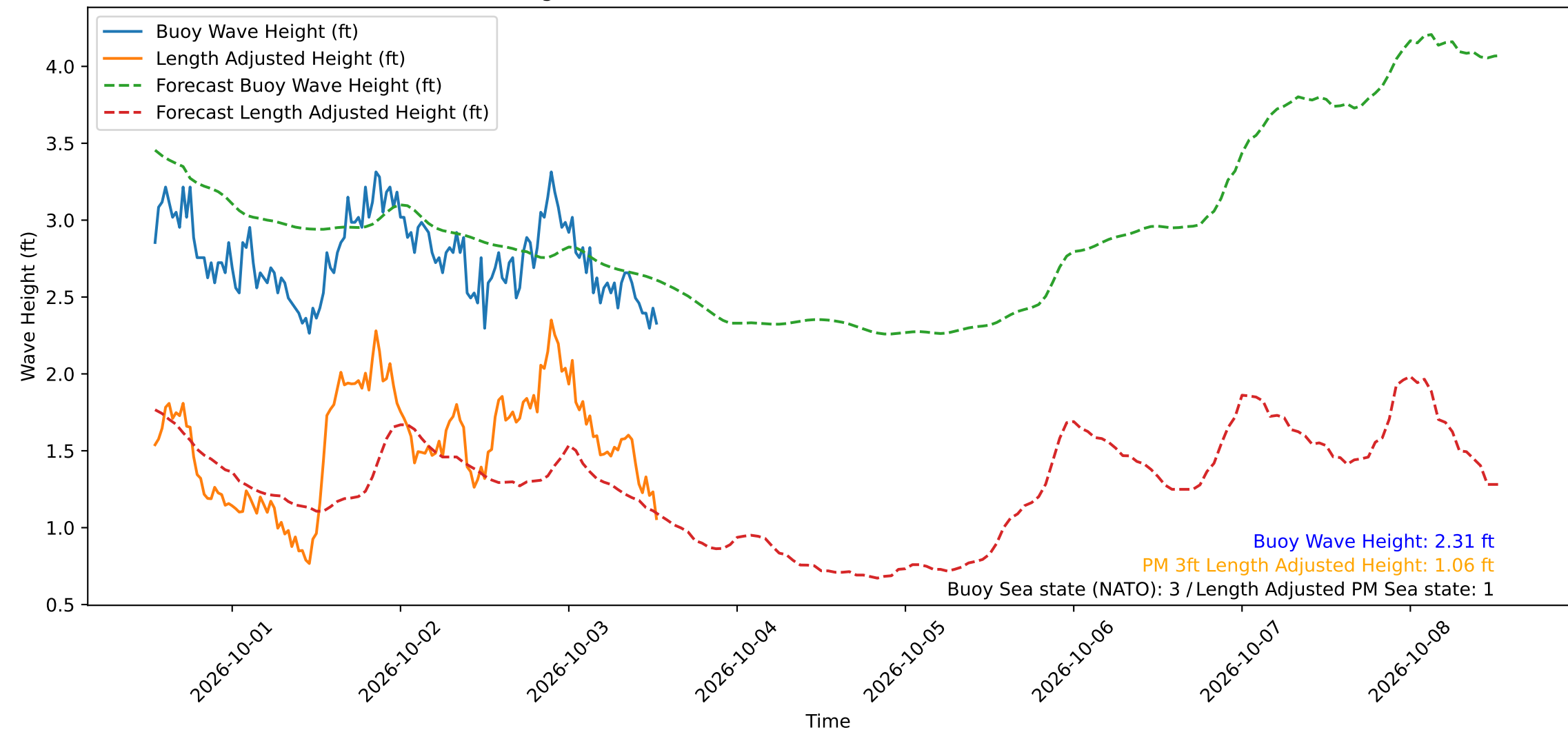
Wave Heights over Time for Oceanside Harbor at 2026-10-03 13:00:30
