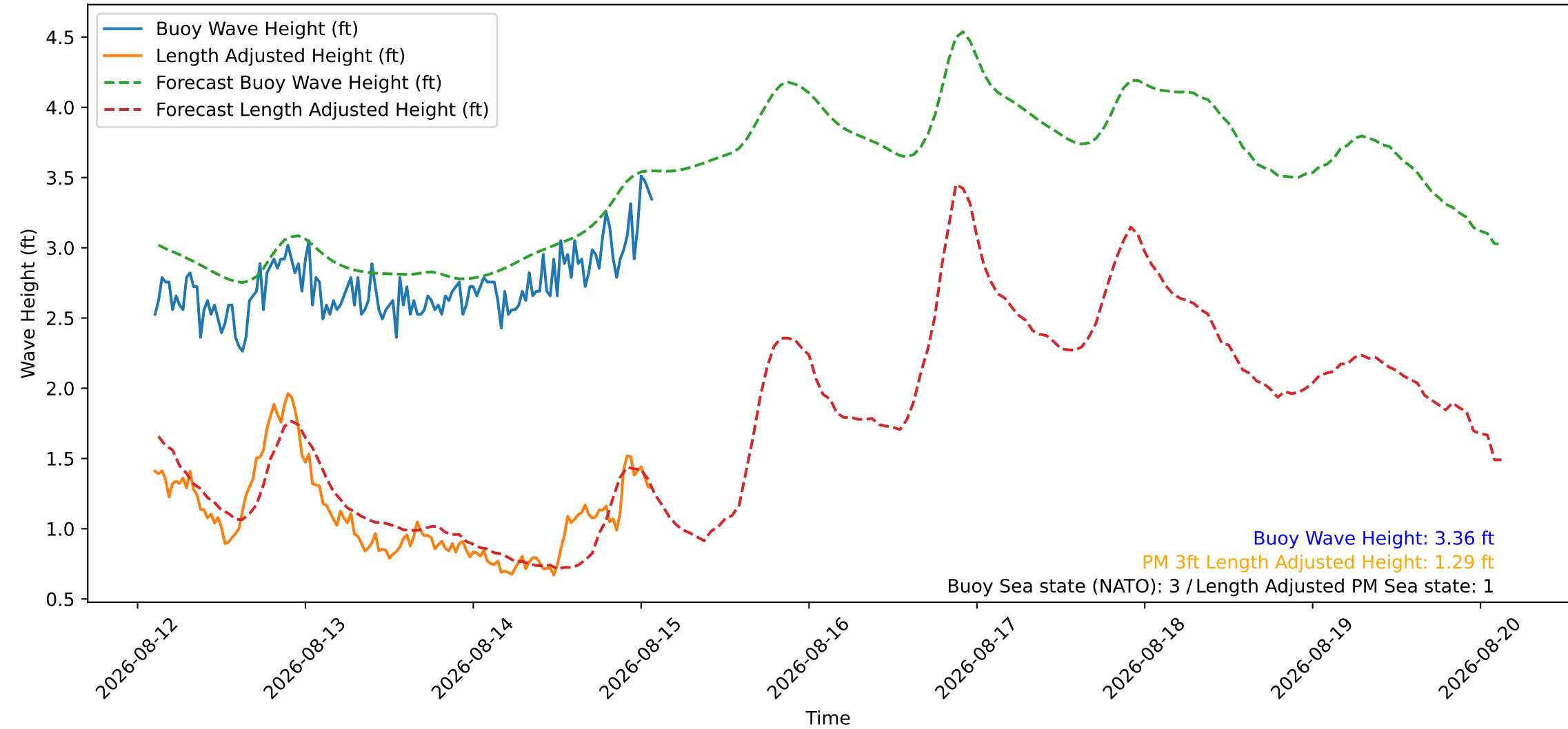
Wave Heights over Time for Green Beach at 2026-08-15 02:31:08
