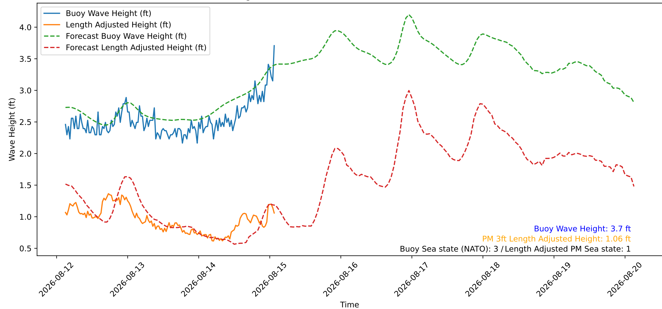
Wave Heights over Time for Red Beach at 2026-08-15 02:30:46
