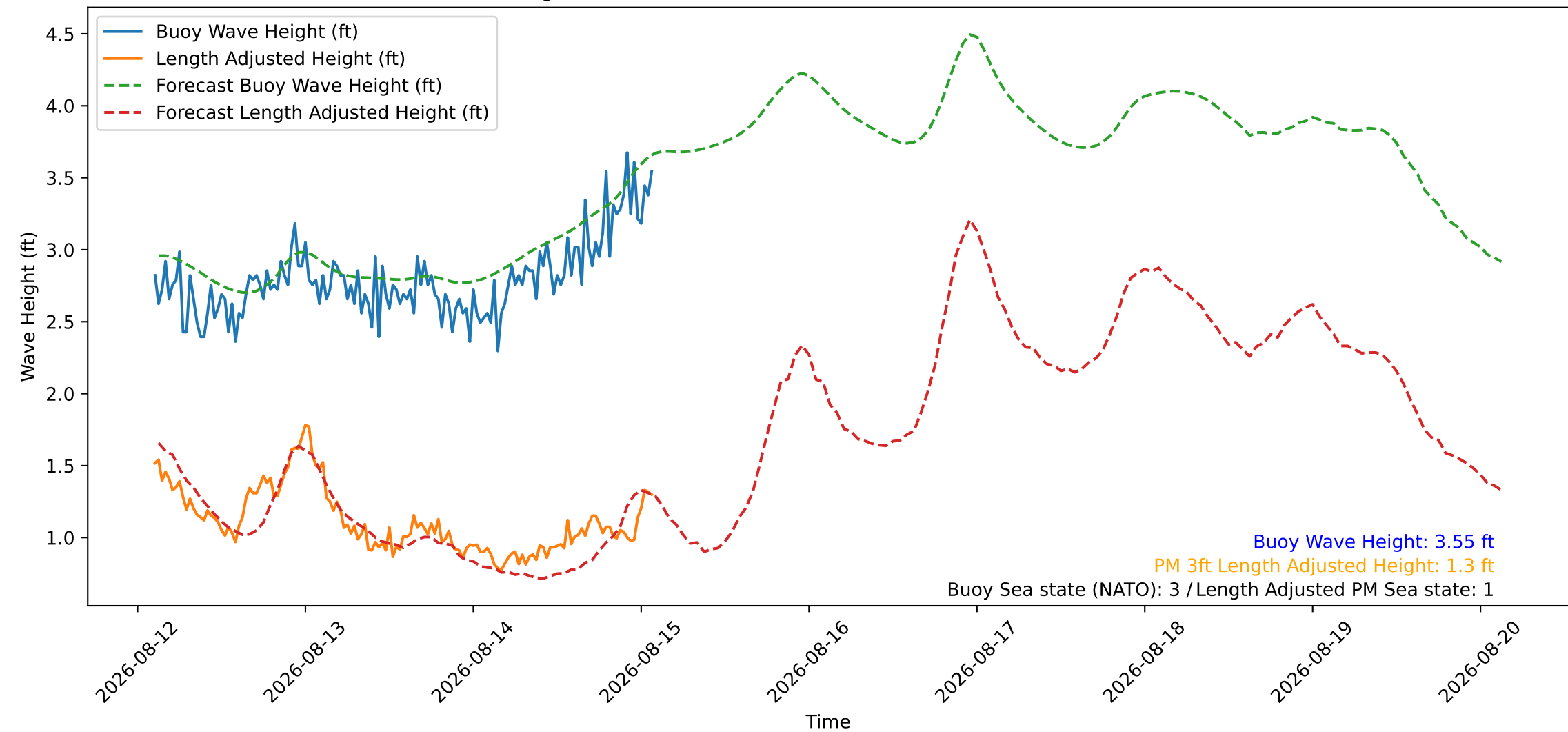
Wave Heights over Time for Oceanside Harbor at 2026-08-15 02:30:26
