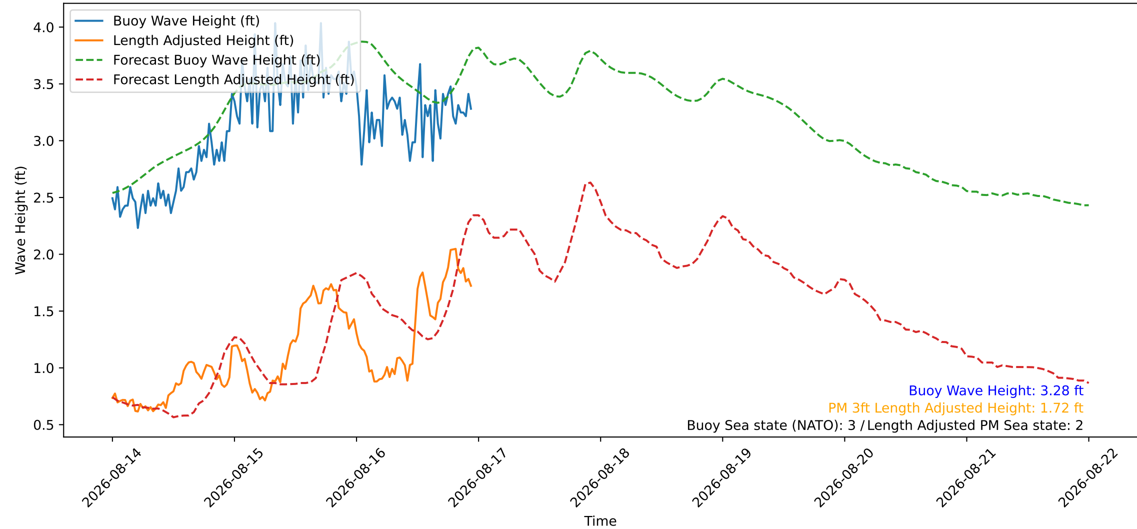
Wave Heights over Time for Red Beach at 2026-08-16 23:30:46
