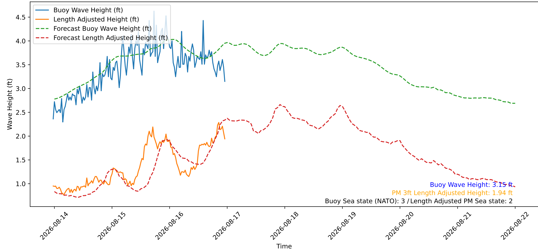
Wave Heights over Time for Oceanside Harbor at 2026-08-16 23:30:26
