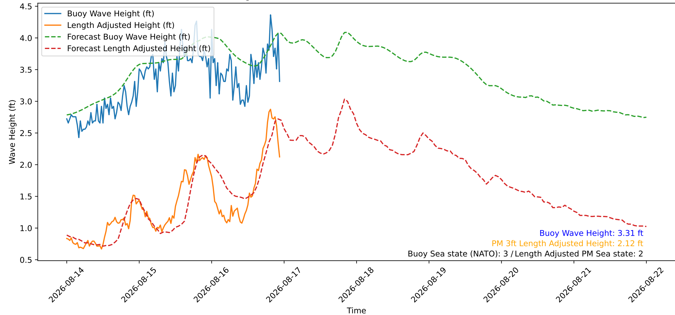
Wave Heights over Time for Green Beach at 2026-08-16 23:31:08
