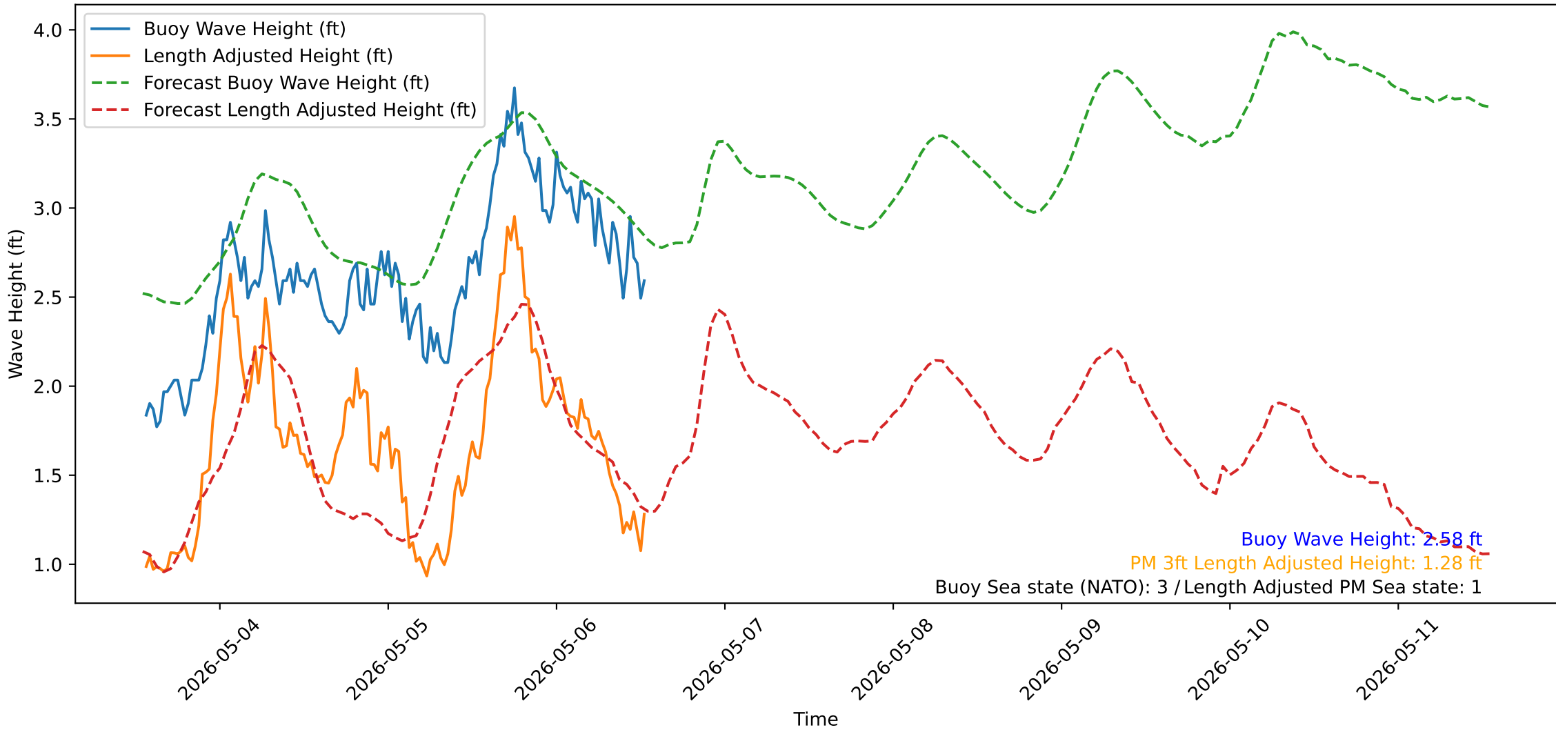
Wave Heights over Time for Green Beach at 2026-05-06 13:21:14
