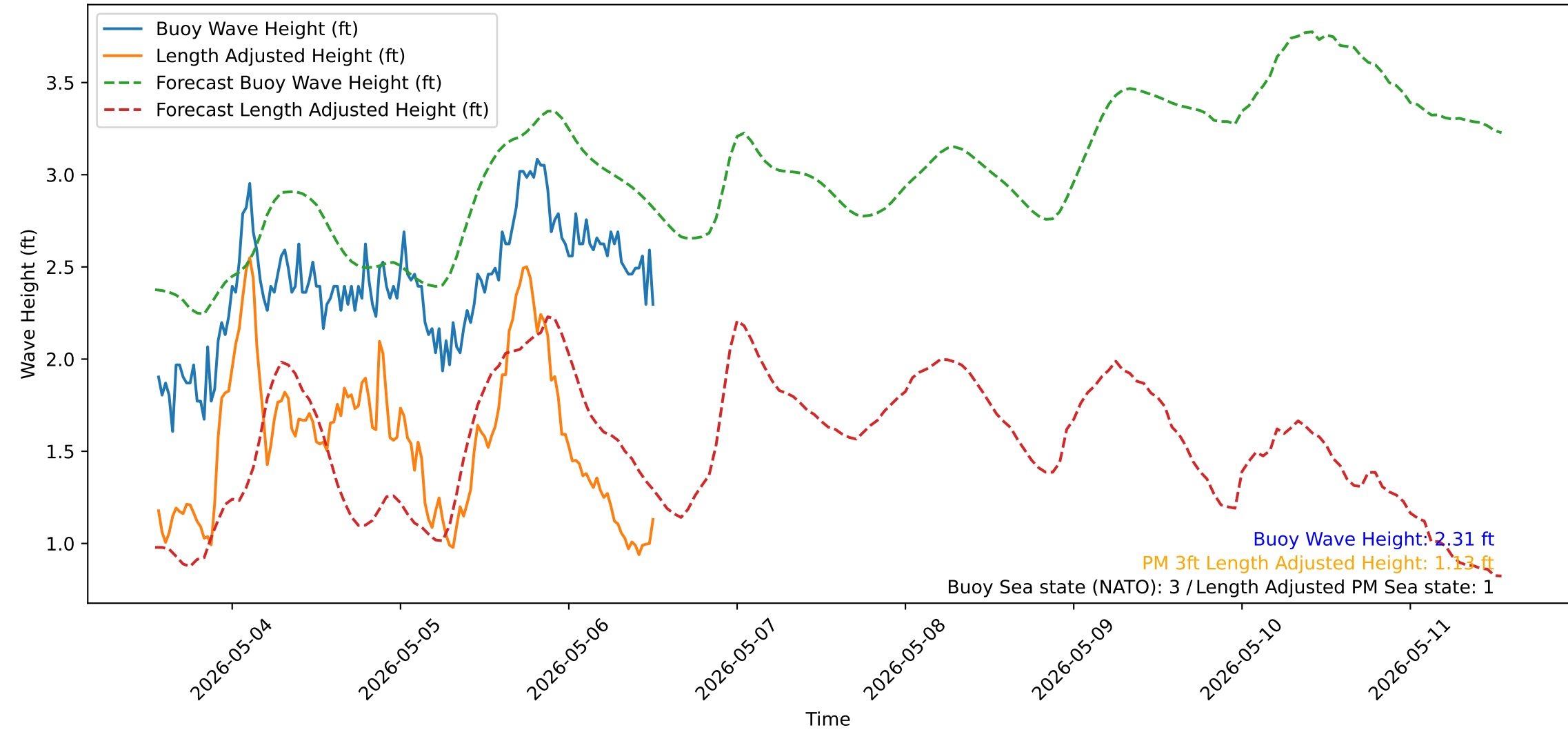
Wave Heights over Time for Red Beach at 2026-05-06 13:20:52
