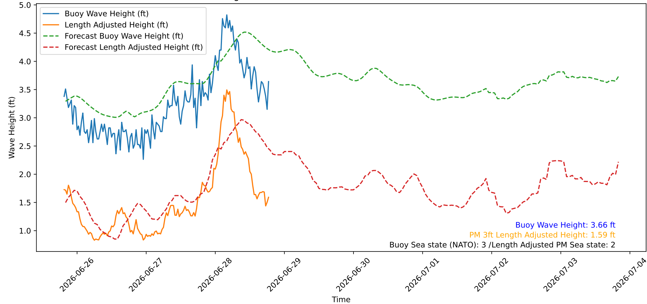
Wave Heights over Time for Green Beach at 2026-06-28 19:31:08
