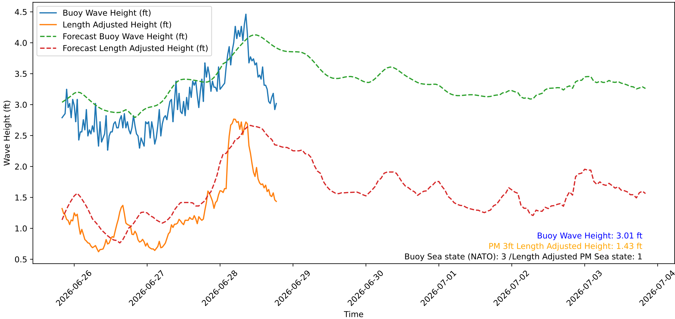
Wave Heights over Time for Red Beach at 2026-06-28 19:30:46
