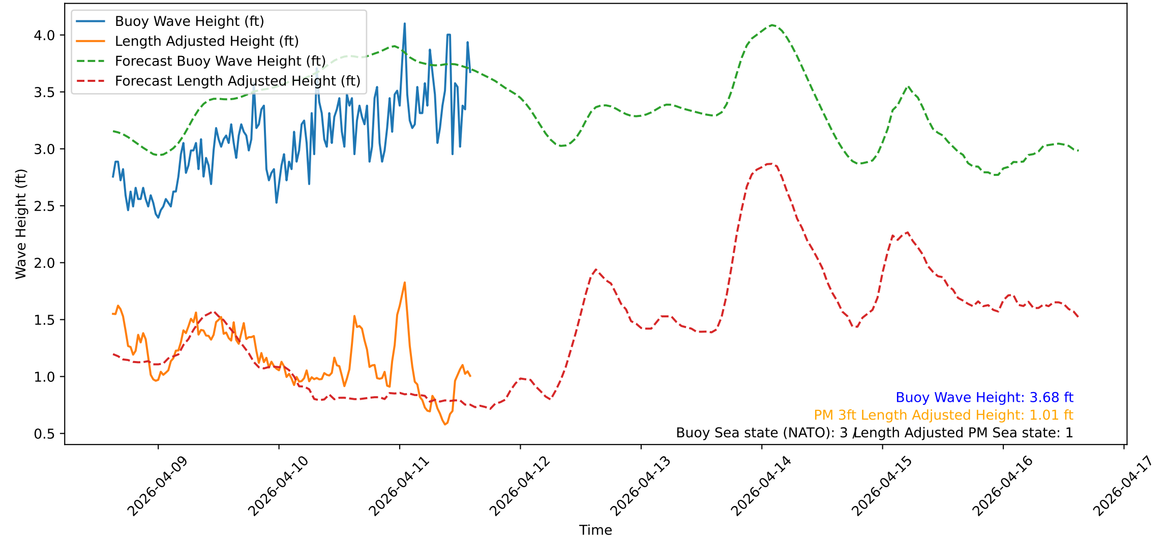
Wave Heights over Time for Red Beach at 2026-04-11 14:50:51
