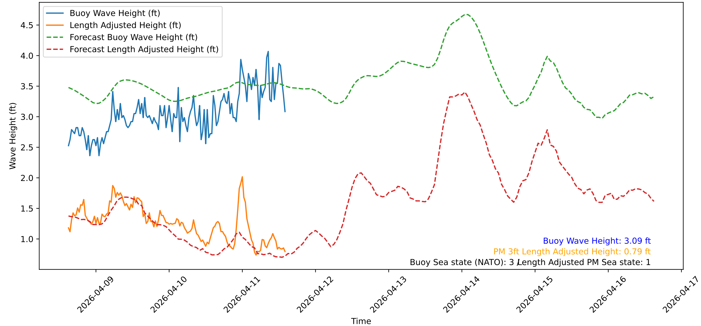
Wave Heights over Time for Green Beach at 2026-04-11 14:51:14
