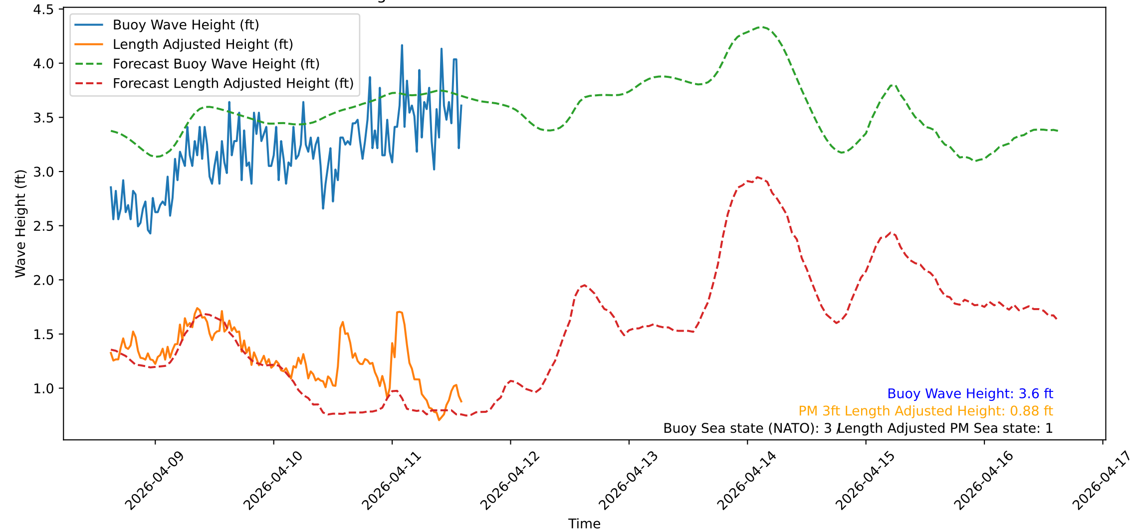
Wave Heights over Time for Oceanside Harbor at 2026-04-11 14:50:31
