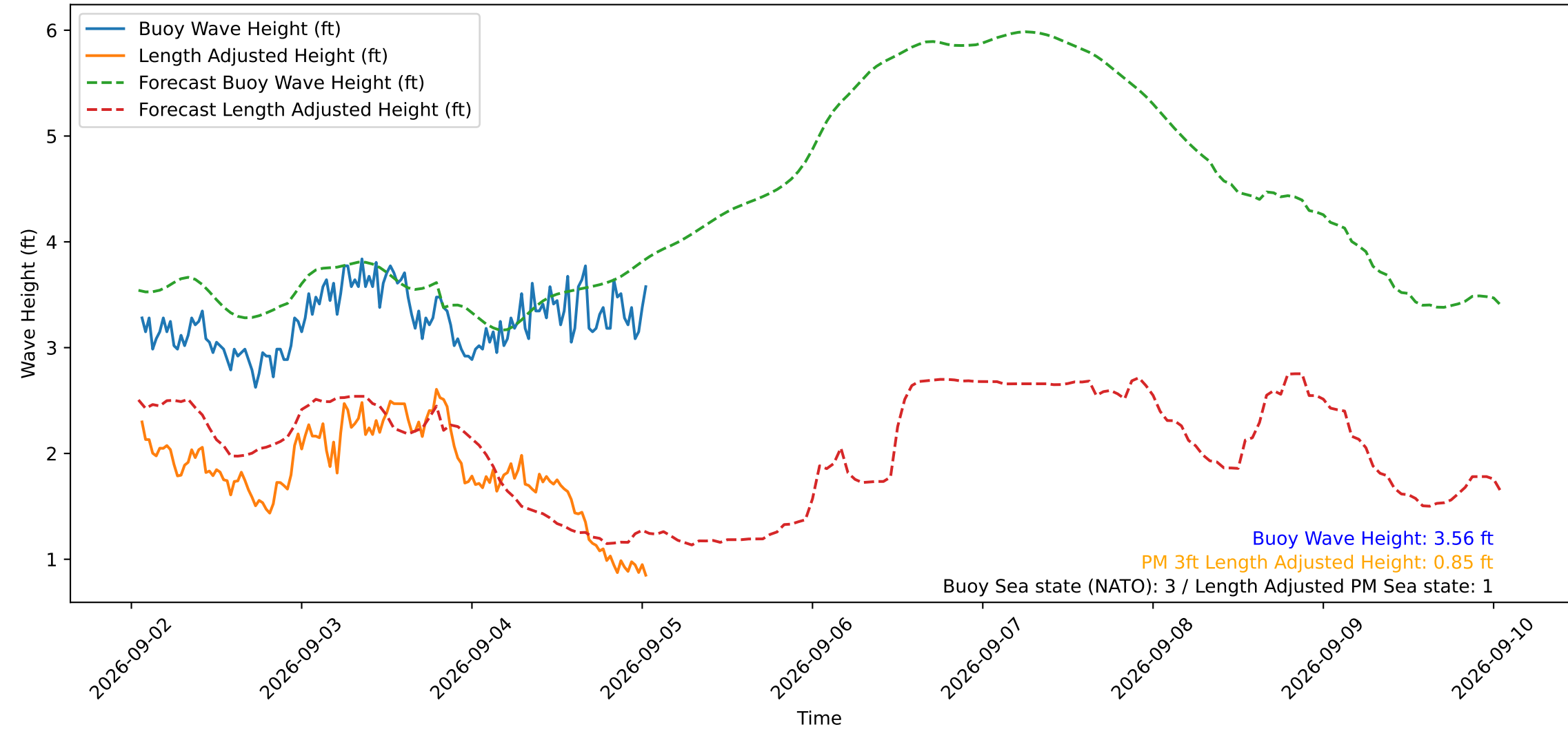
Wave Heights over Time for Oceanside Harbor at 2026-09-05 01:20:29
