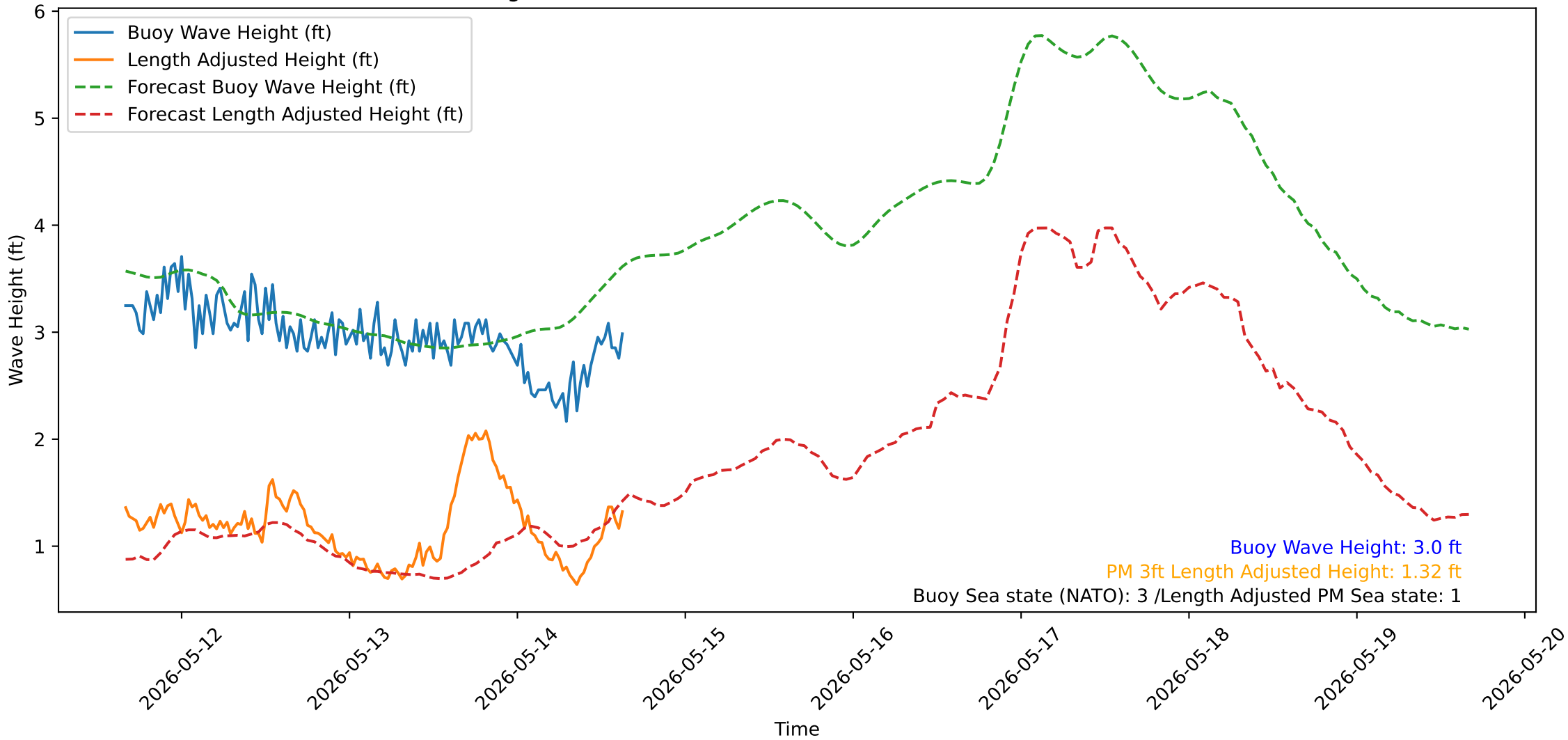
Wave Heights over Time for Oceanside Harbor at 2026-05-14 16:00:32
