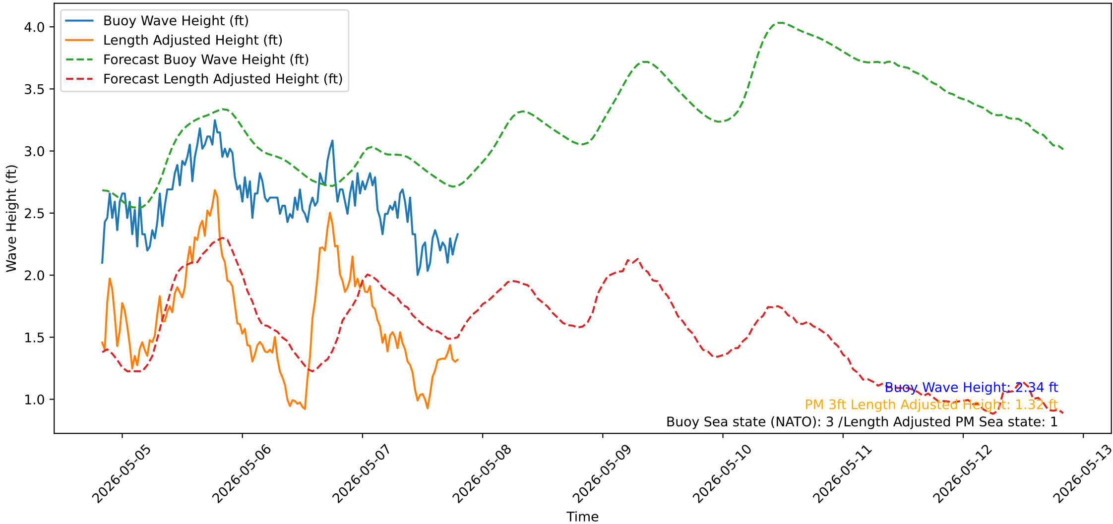
Wave Heights over Time for Oceanside Harbor at 2026-05-07 19:50:31
