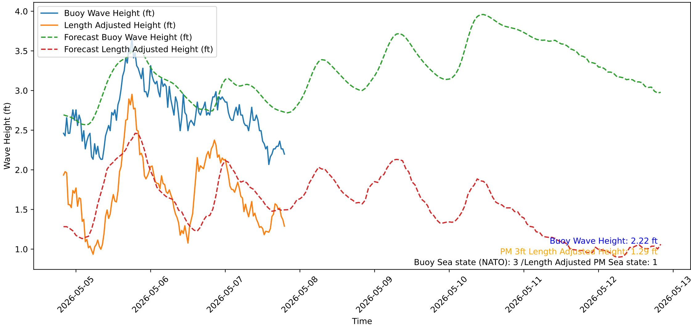
Wave Heights over Time for Green Beach at 2026-05-07 19:51:14
