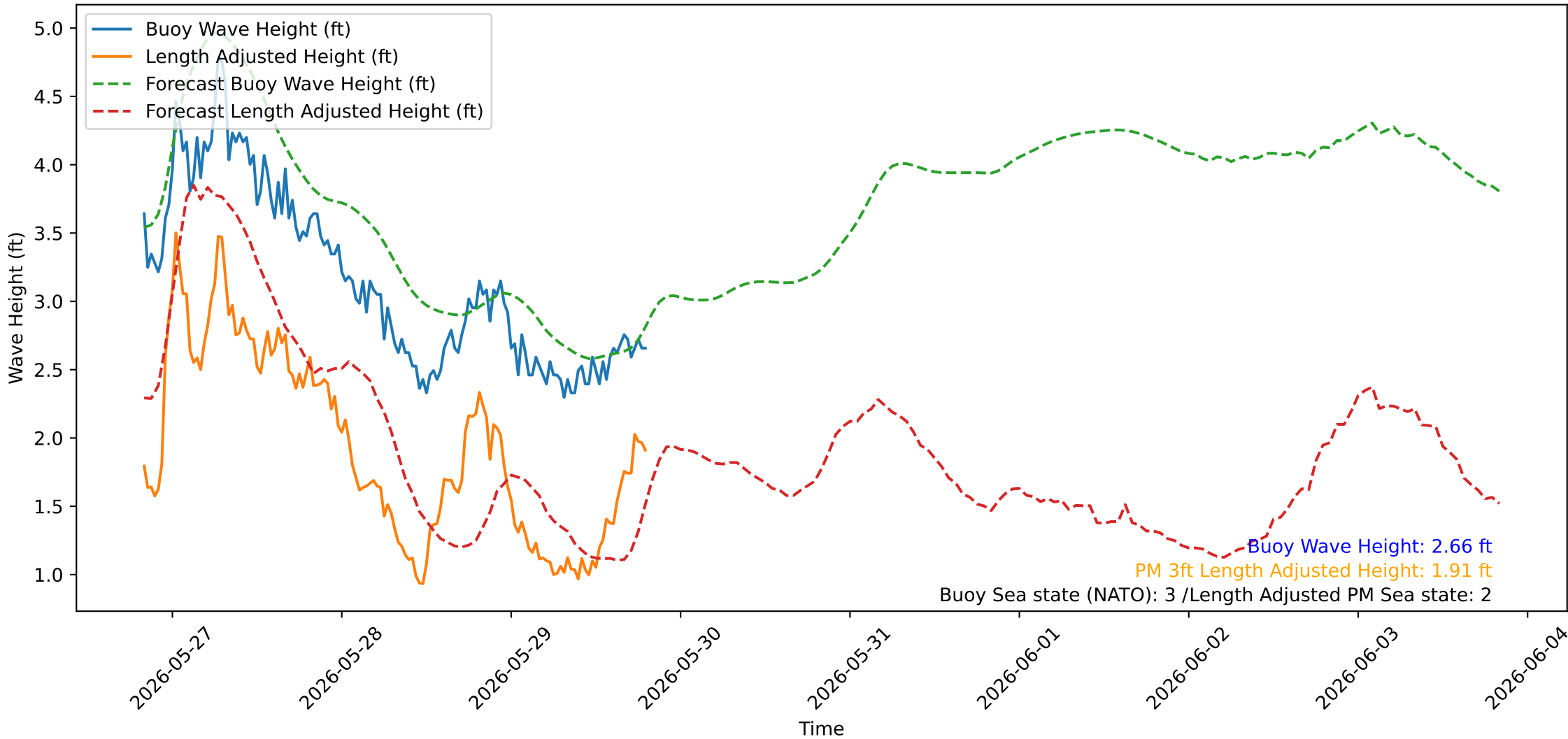
Wave Heights over Time for Red Beach at 2026-05-29 19:50:43
