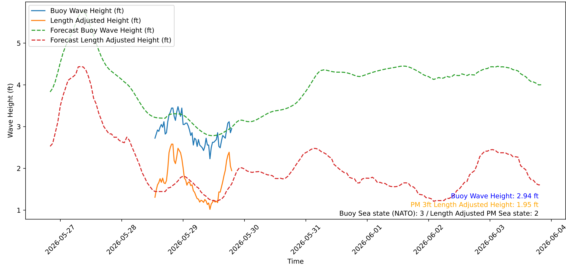
Wave Heights over Time for Oceanside Harbor at 2026-05-29 19:50:22
