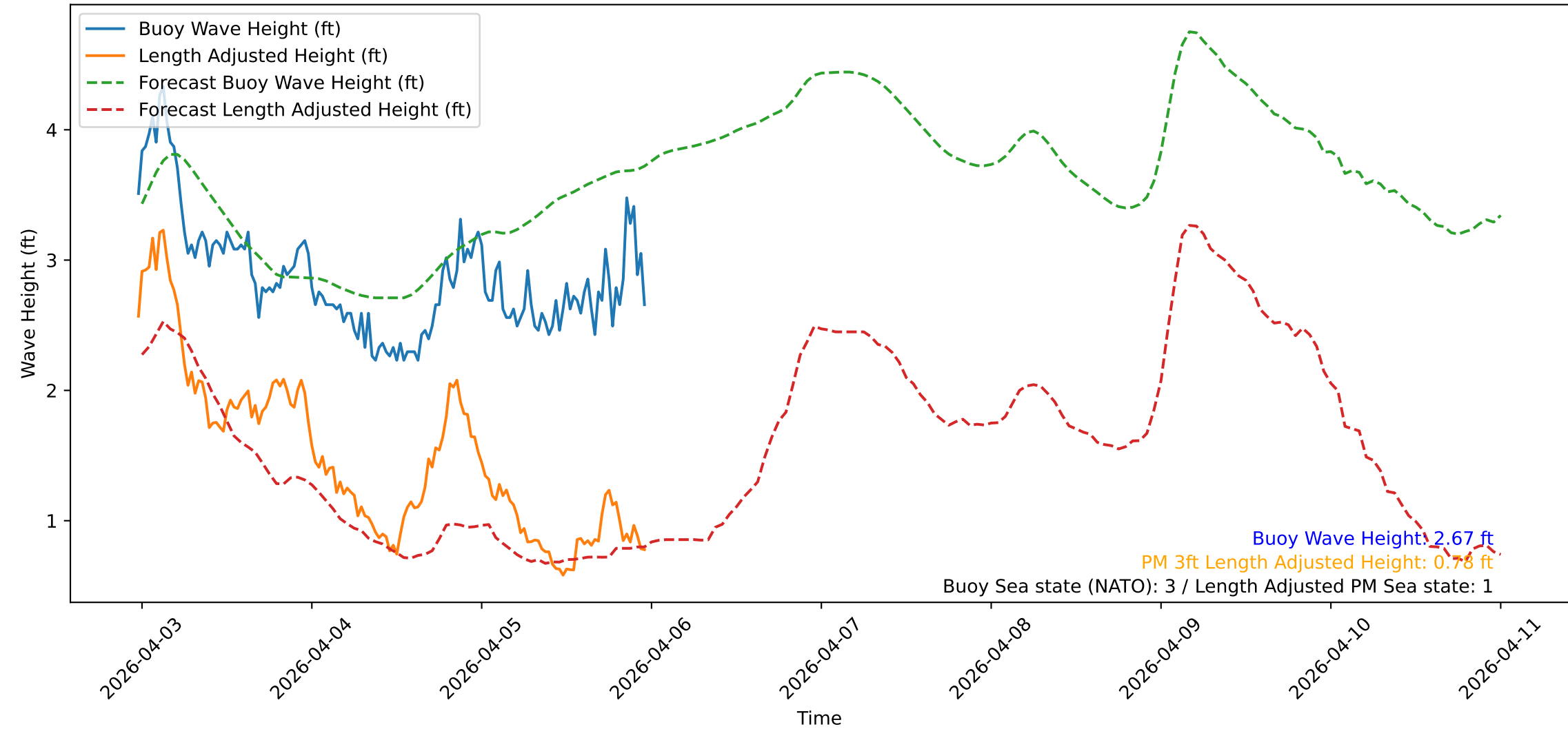
Wave Heights over Time for Green Beach at 2026-04-05 23:41:10
