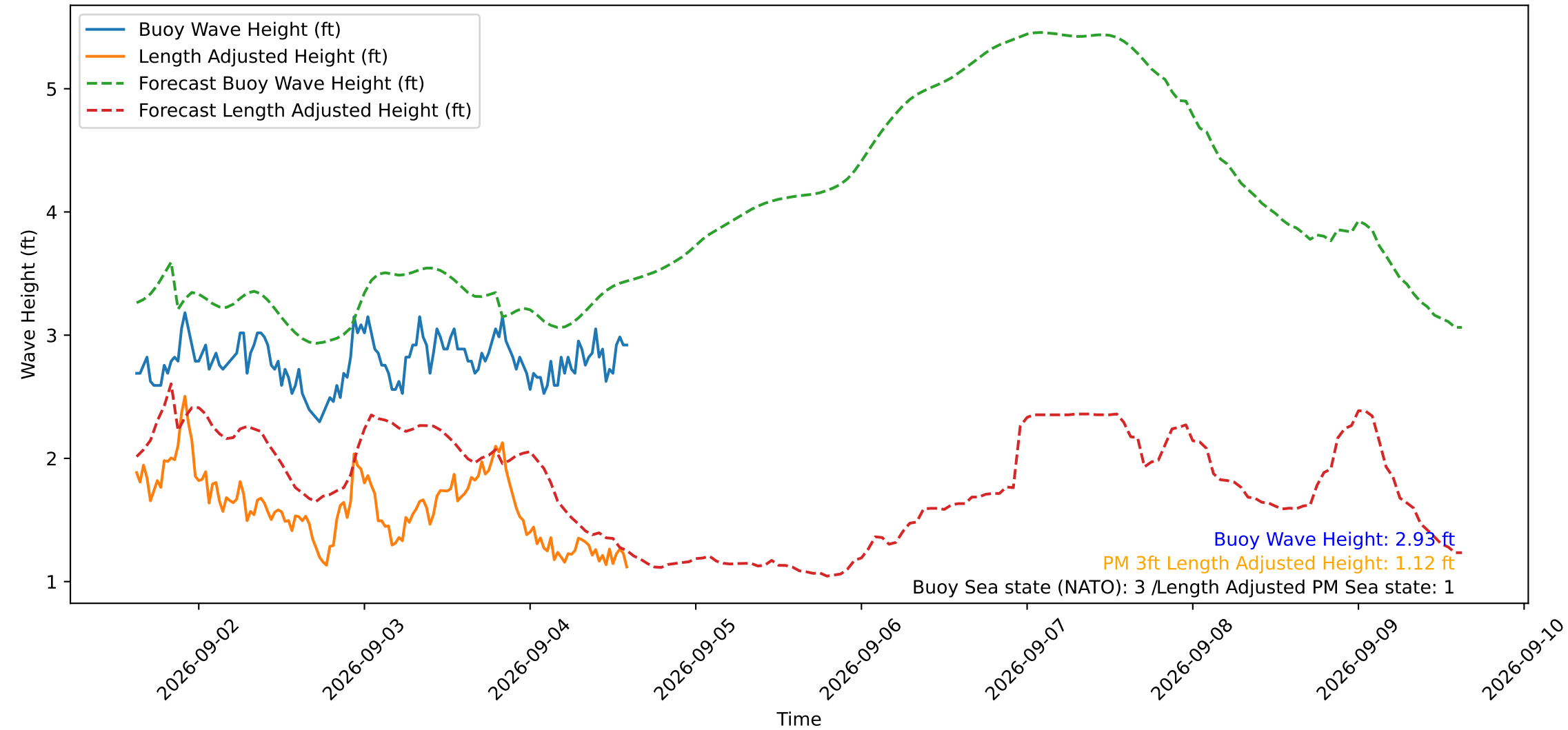
Wave Heights over Time for Red Beach at 2026-09-04 14:50:51
