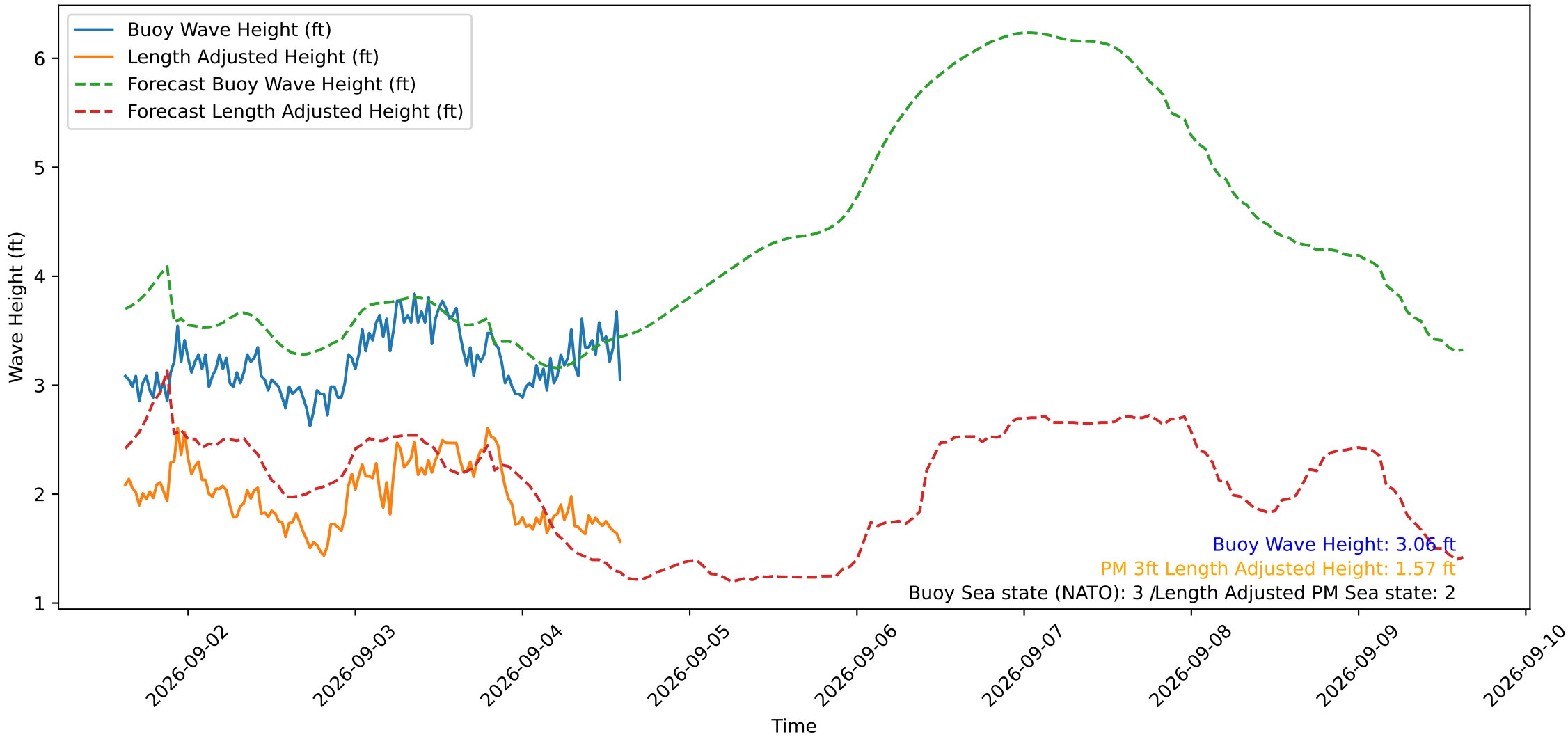
Wave Heights over Time for Oceanside Harbor at 2026-09-04 14:50:30
