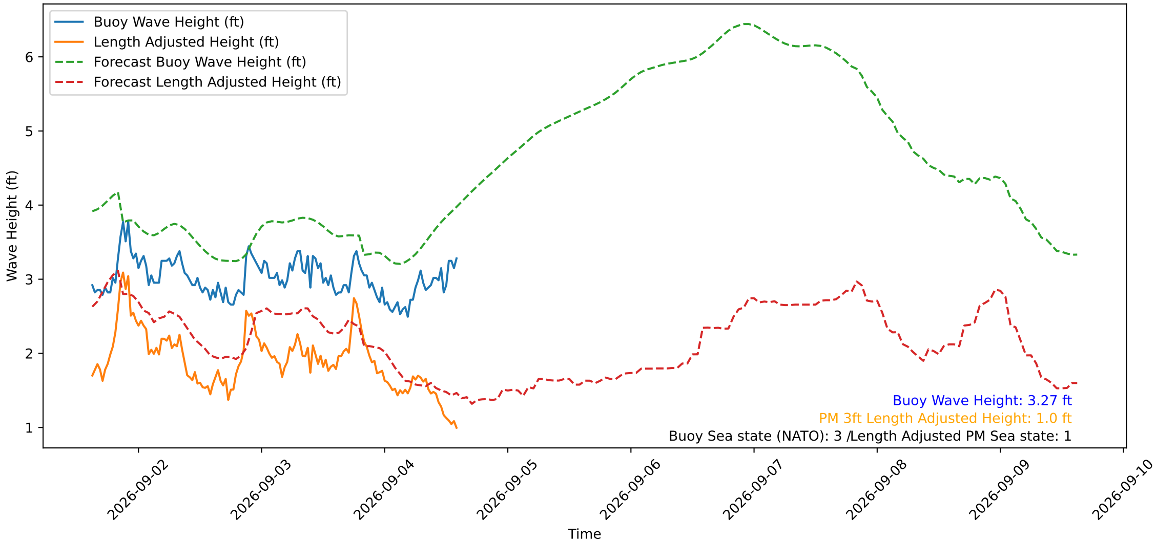
Wave Heights over Time for Green Beach at 2026-09-04 14:51:15
