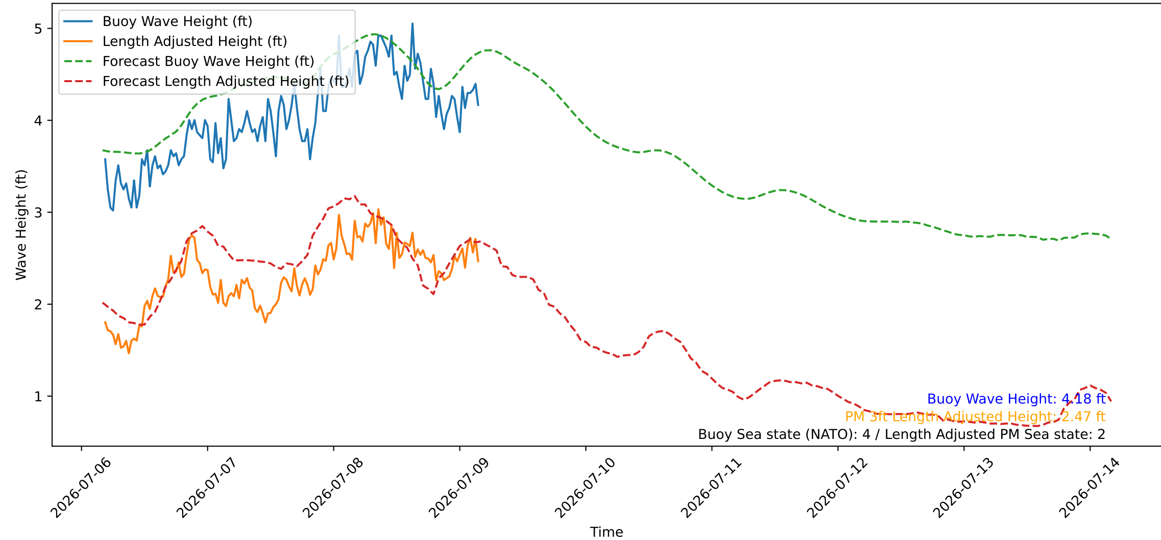
Wave Heights over Time for Oceanside Harbor at 2026-07-09 04:20:26
