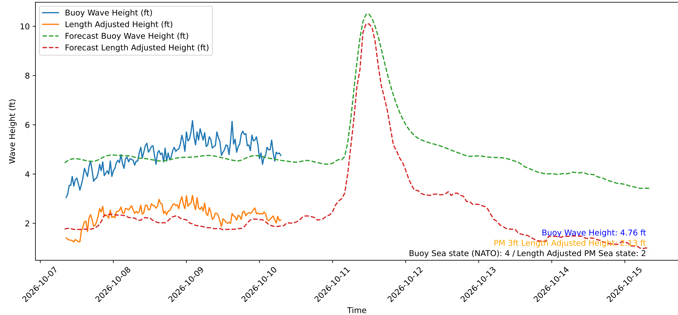
Wave Heights over Time for Green Beach at 2026-10-10 08:01:12
