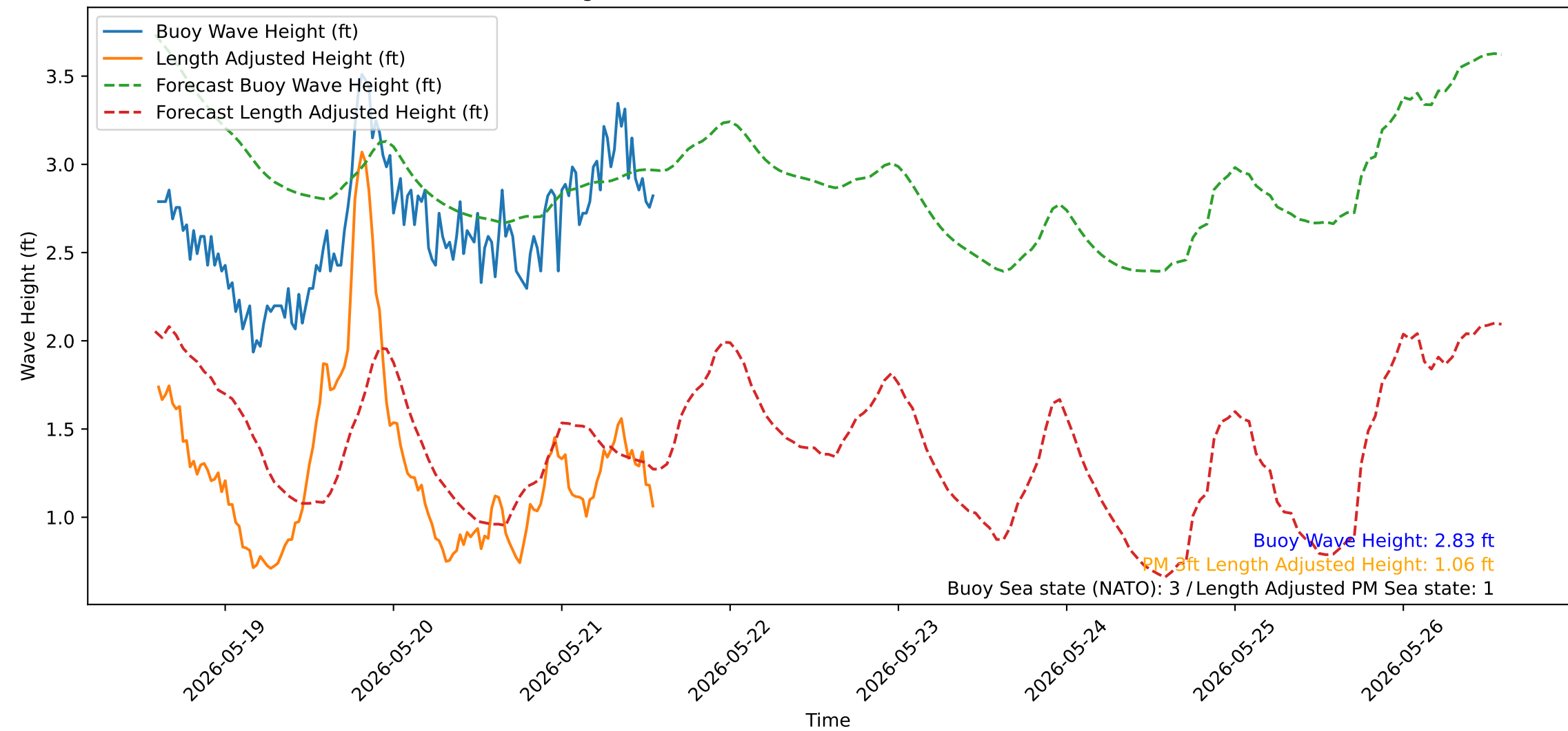
Wave Heights over Time for Red Beach at 2026-05-21 14:00:51
