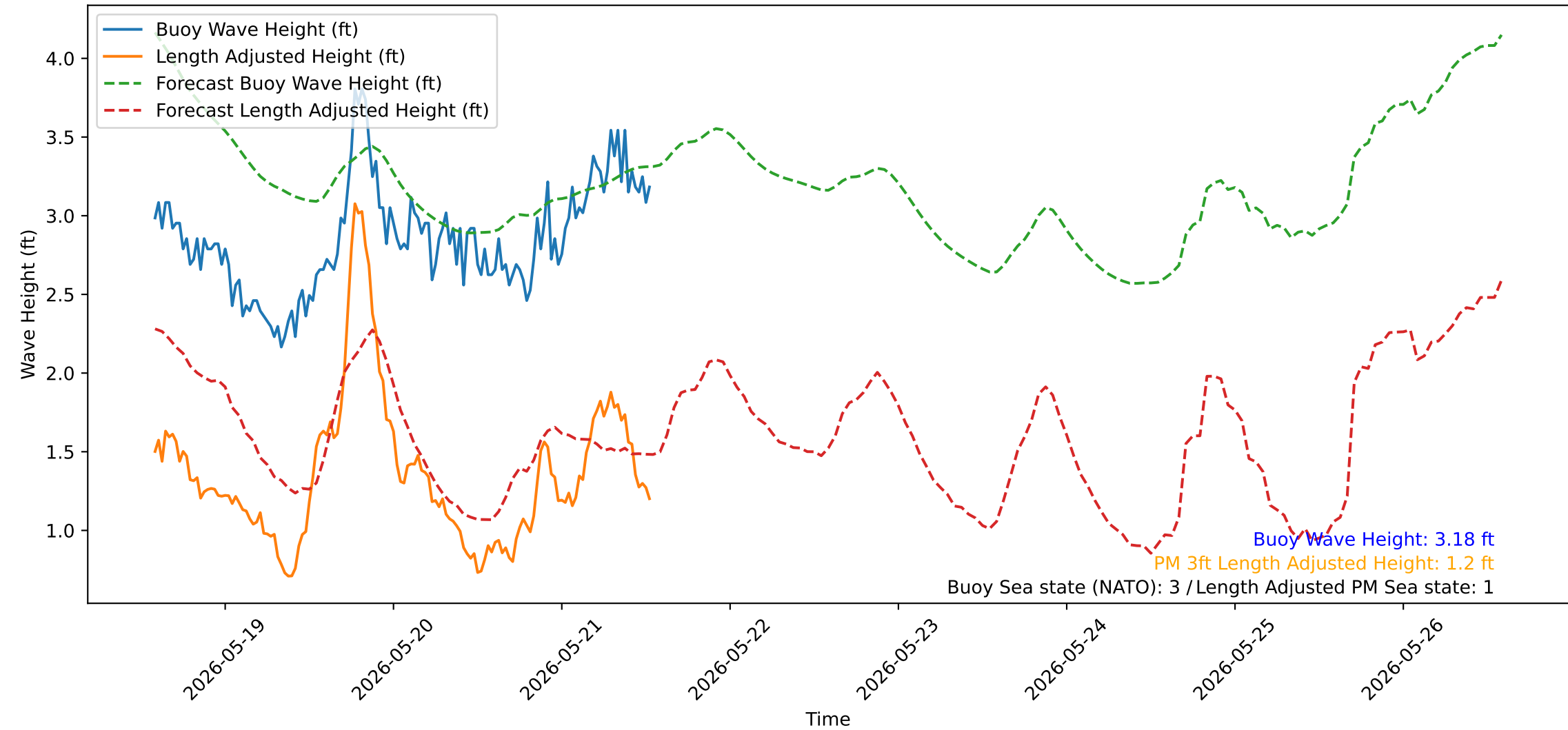
Wave Heights over Time for Green Beach at 2026-05-21 14:01:14
