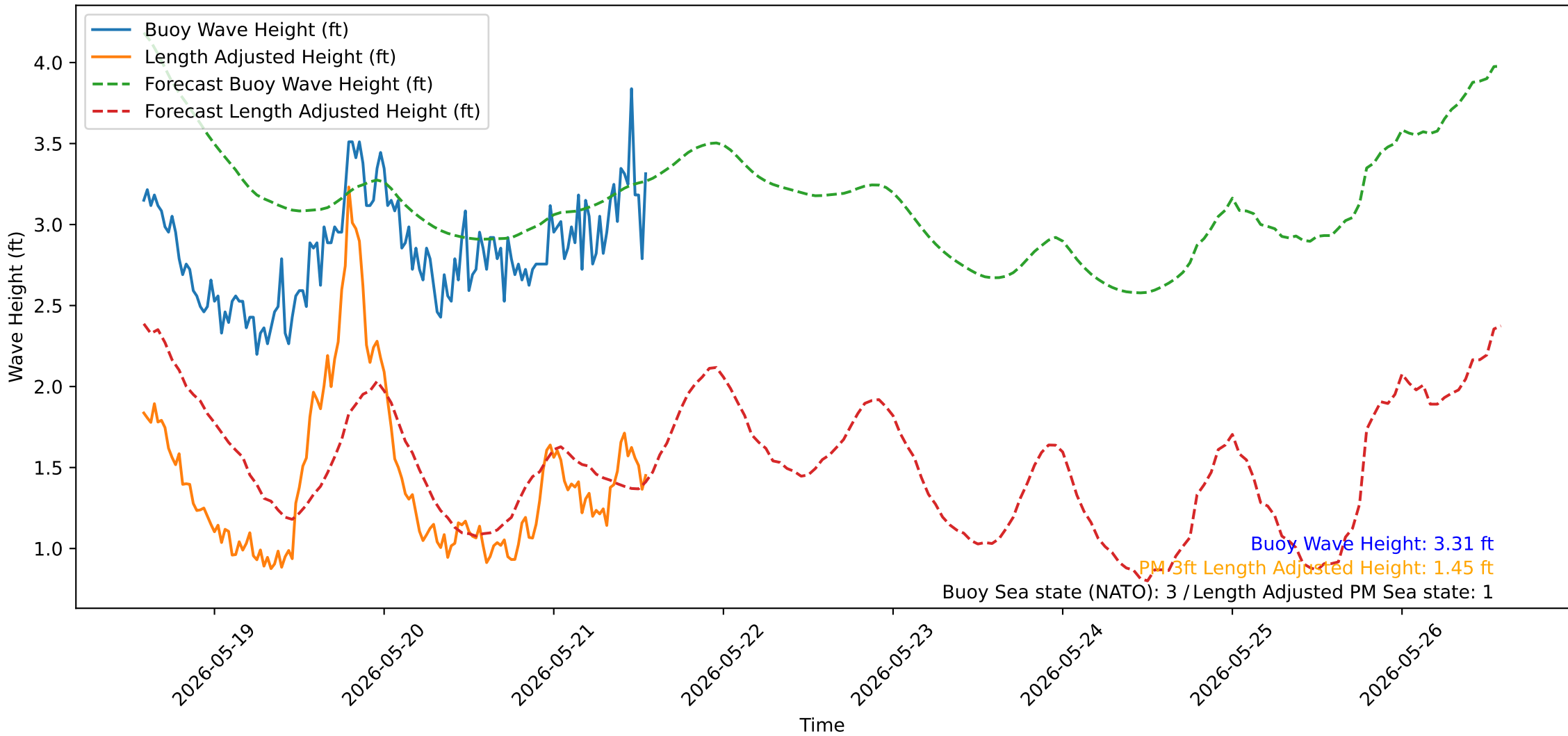
Wave Heights over Time for Oceanside Harbor at 2026-05-21 14:00:31
