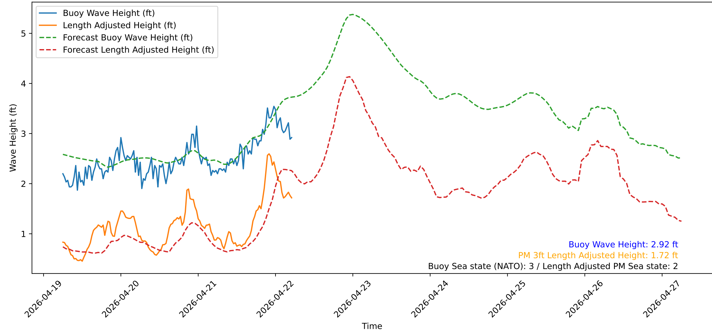
Wave Heights over Time for Green Beach at 2026-04-22 05:51:14
