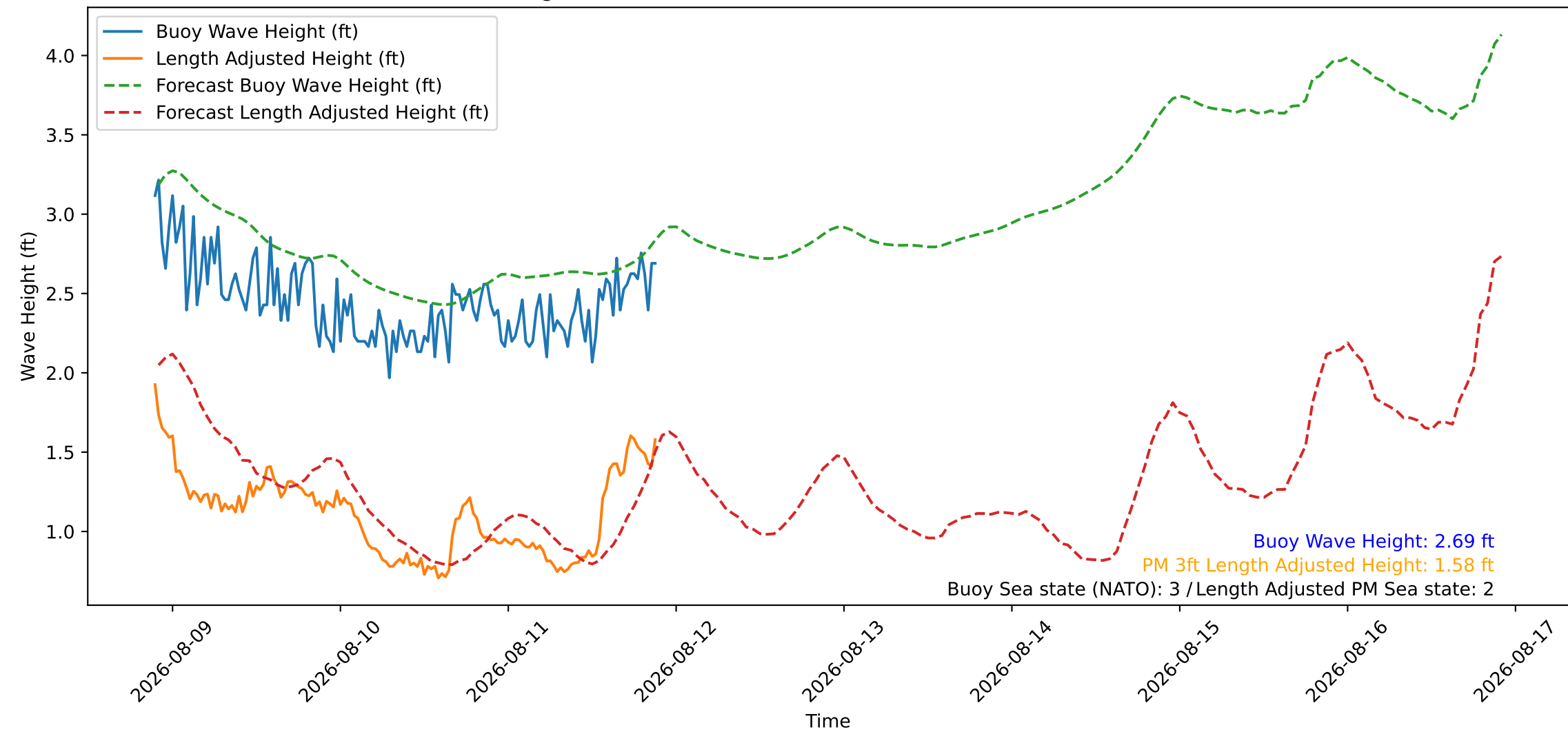
Wave Heights over Time for Oceanside Harbor at 2026-08-11 21:40:27
