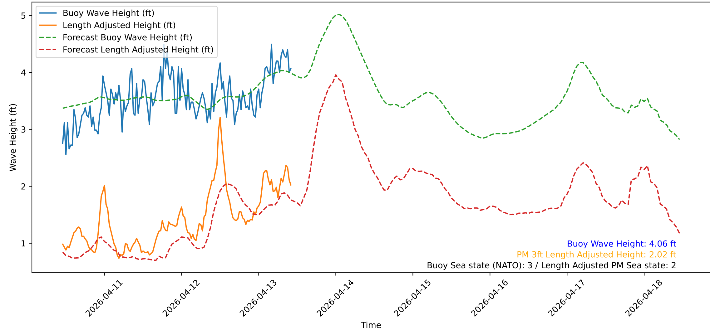
Wave Heights over Time for Green Beach at 2026-04-13 11:01:12
