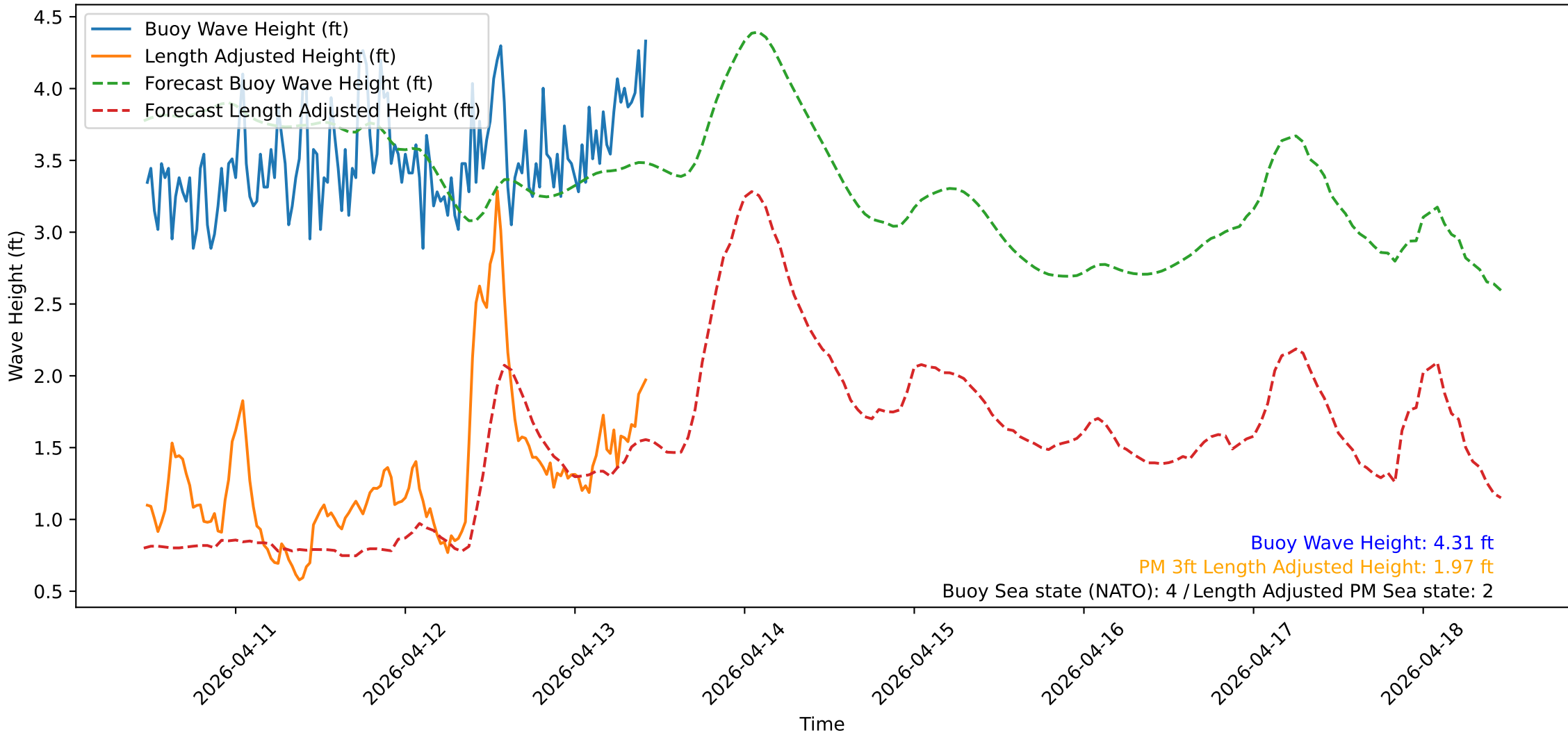
Wave Heights over Time for Red Beach at 2026-04-13 11:00:50
