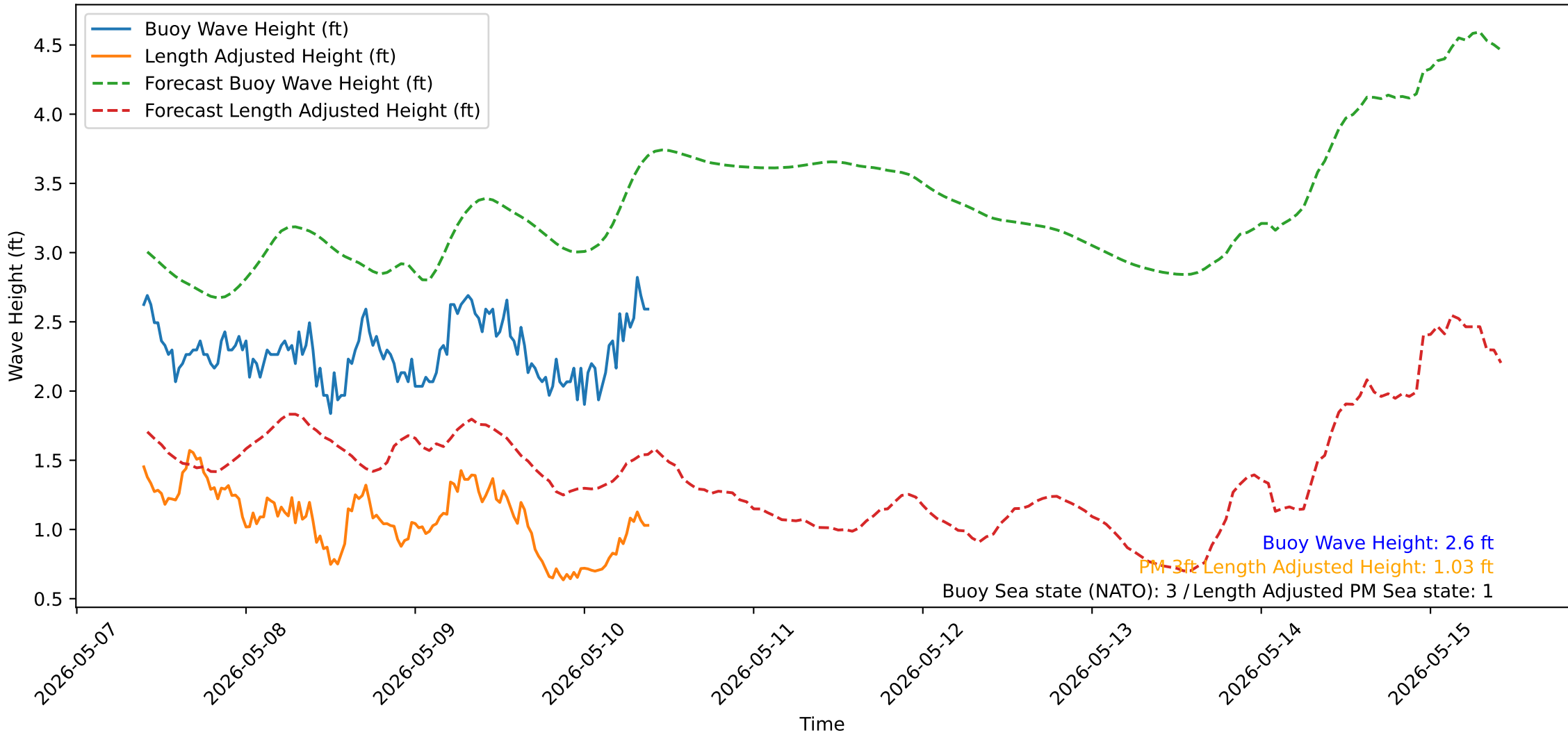
Wave Heights over Time for Green Beach at 2026-05-10 09:41:13
