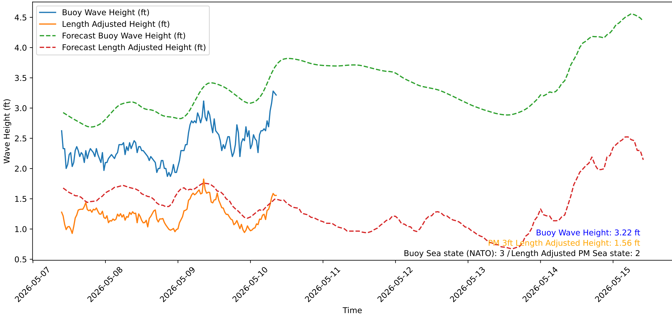
Wave Heights over Time for Oceanside Harbor at 2026-05-10 09:40:32
