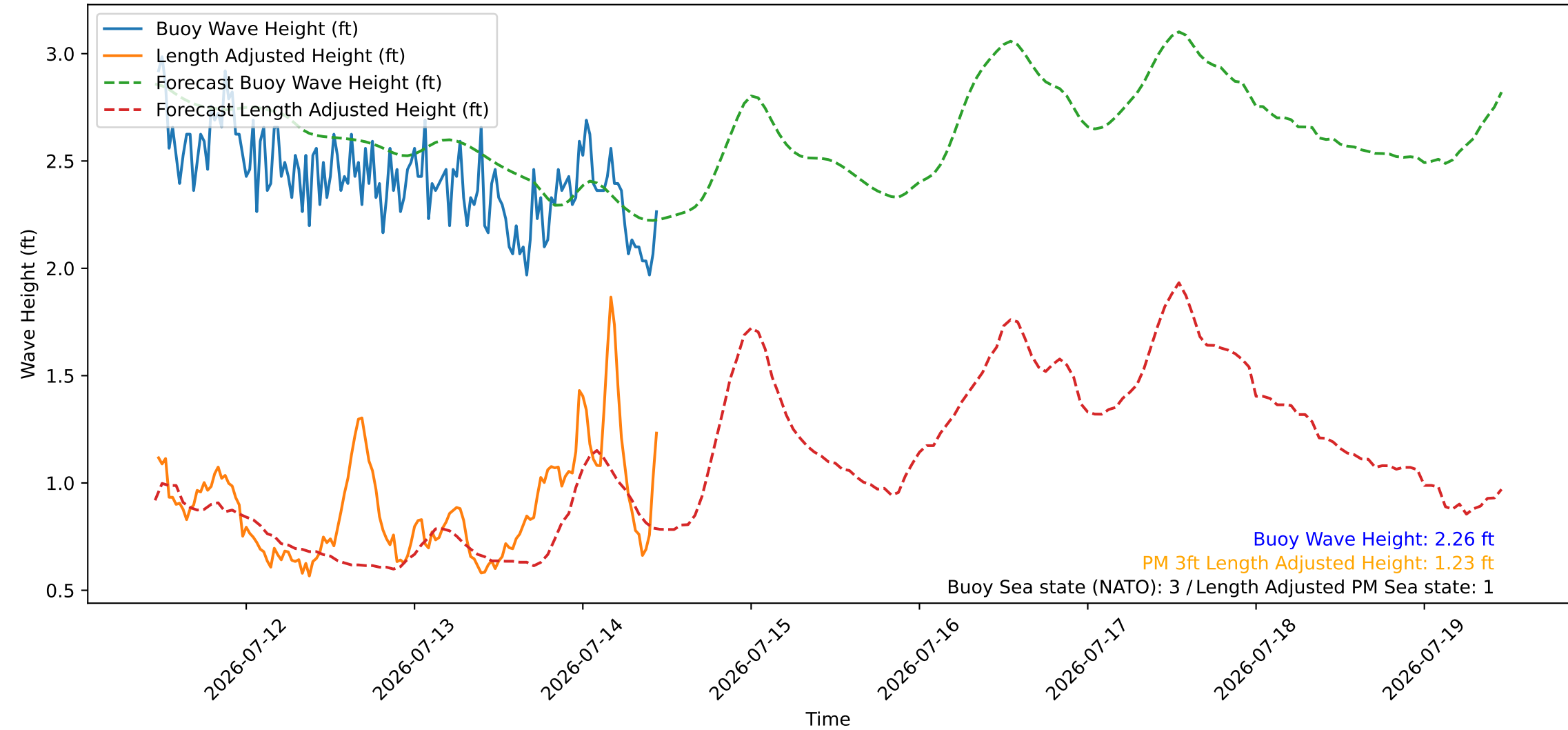
Wave Heights over Time for Red Beach at 2026-07-14 11:20:47
