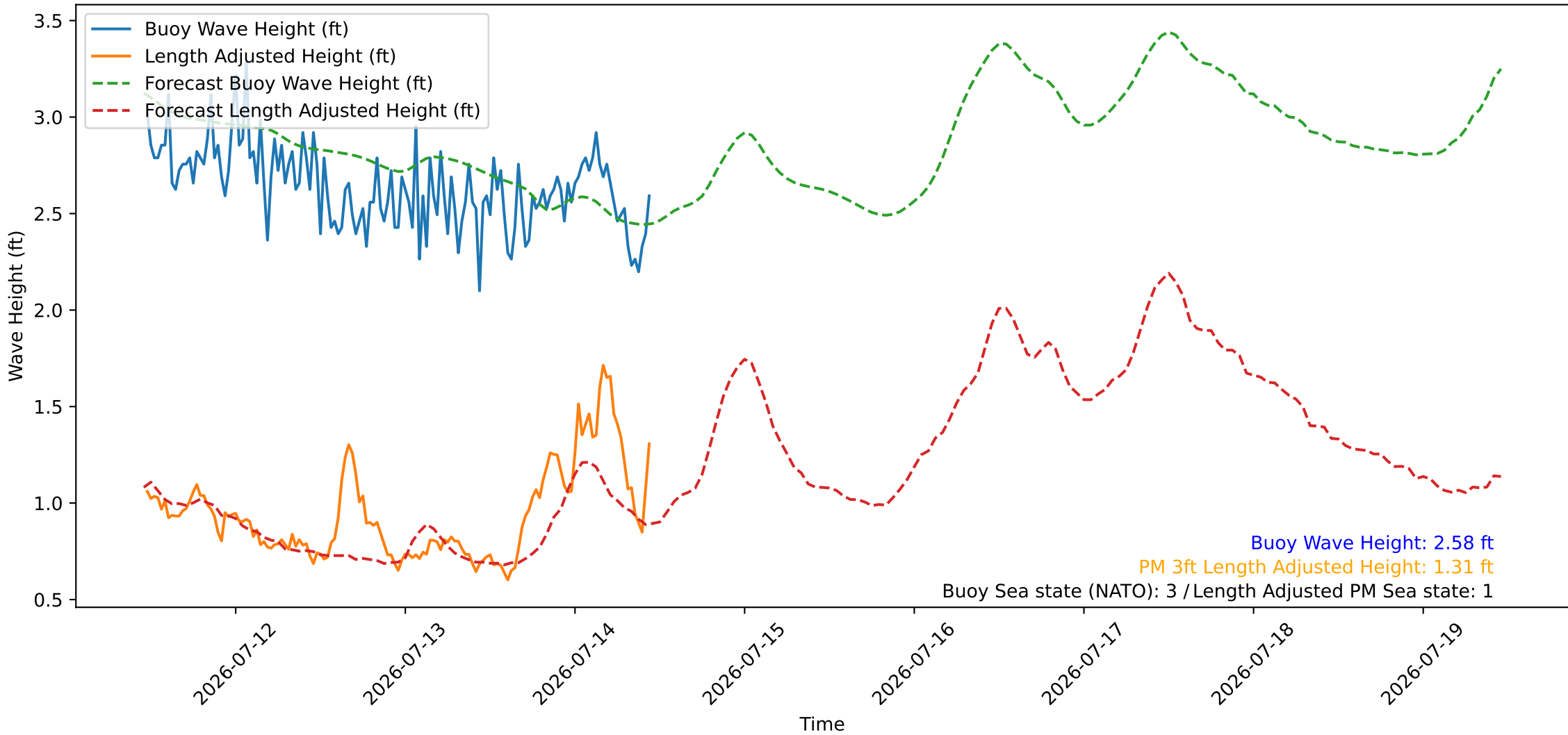
Wave Heights over Time for Oceanside Harbor at 2026-07-14 11:20:27
