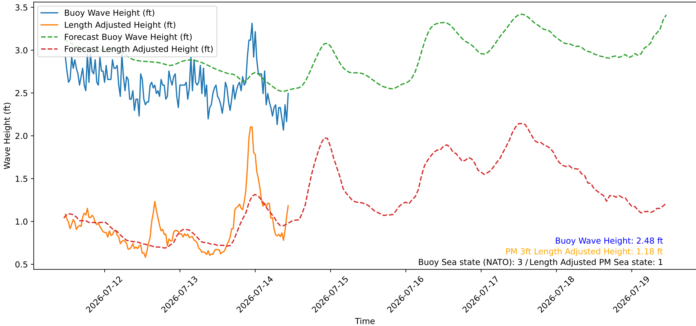
Wave Heights over Time for Green Beach at 2026-07-14 11:21:10
