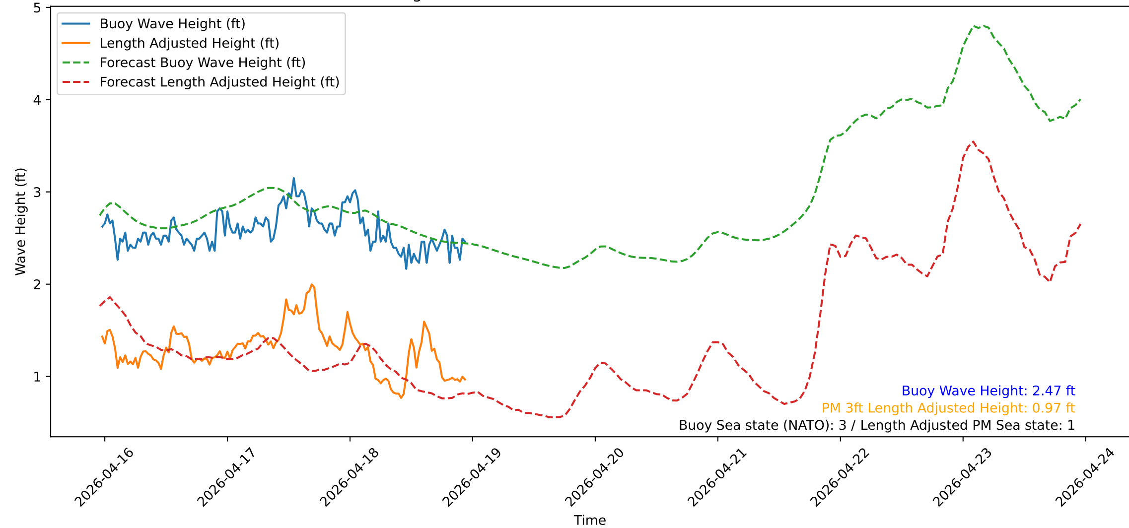
Wave Heights over Time for Red Beach at 2026-04-18 23:20:51
