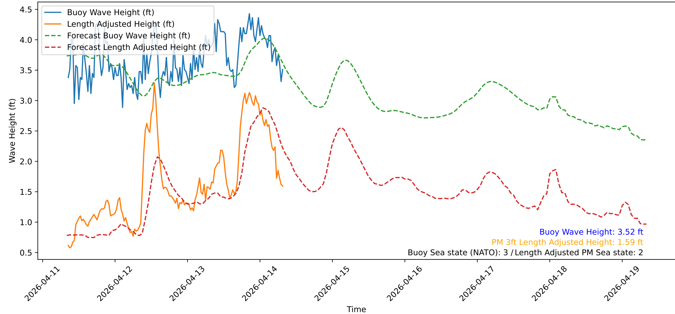
Wave Heights over Time for Red Beach at 2026-04-14 08:20:51
