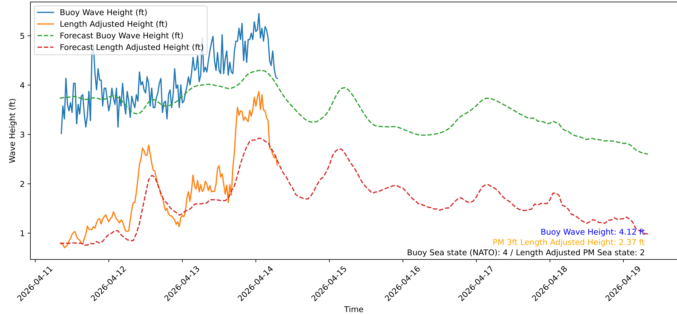
Wave Heights over Time for Oceanside Harbor at 2026-04-14 08:20:31
