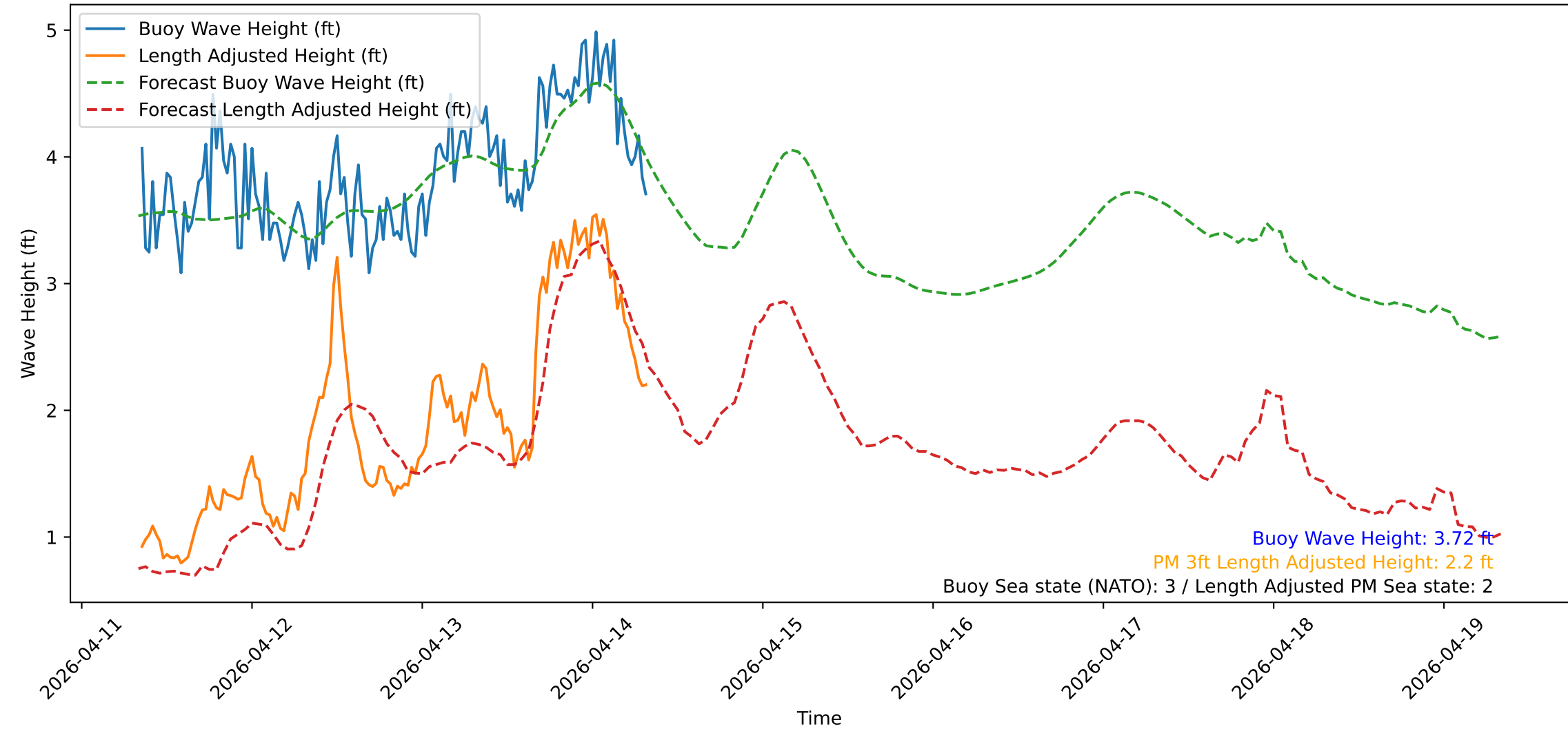
Wave Heights over Time for Green Beach at 2026-04-14 08:21:14
