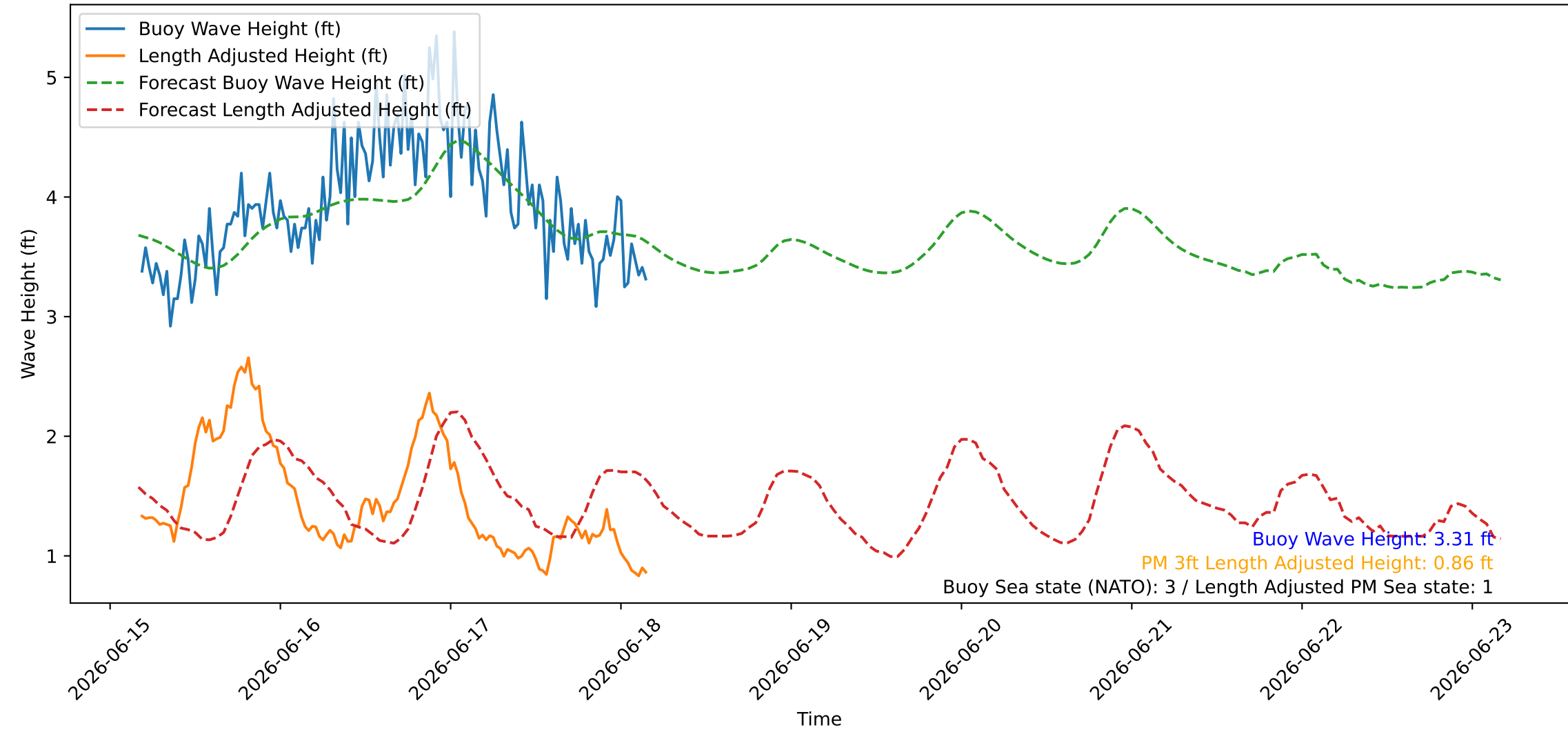
Wave Heights over Time for Red Beach at 2026-06-18 04:10:45
