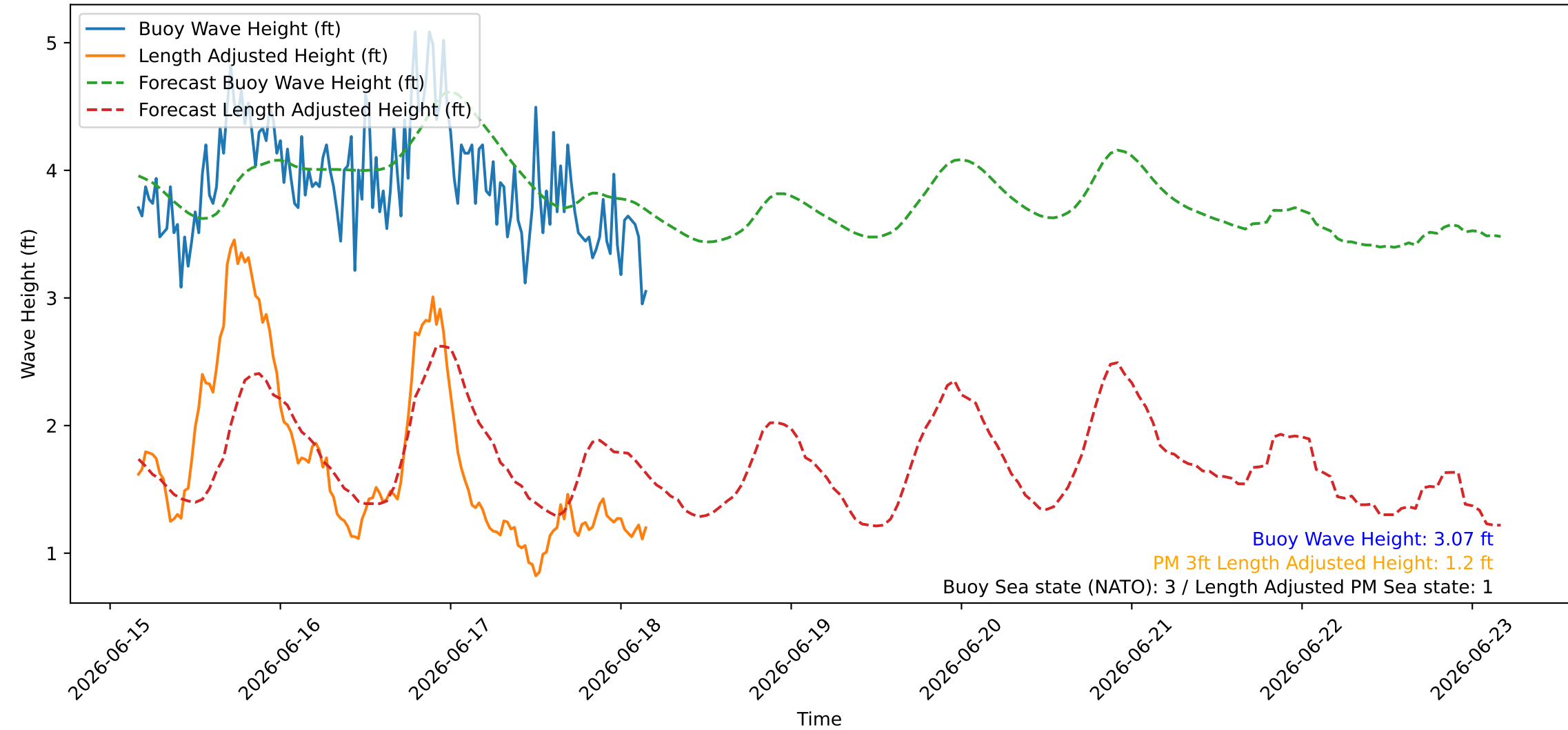
Wave Heights over Time for Green Beach at 2026-06-18 04:11:08
