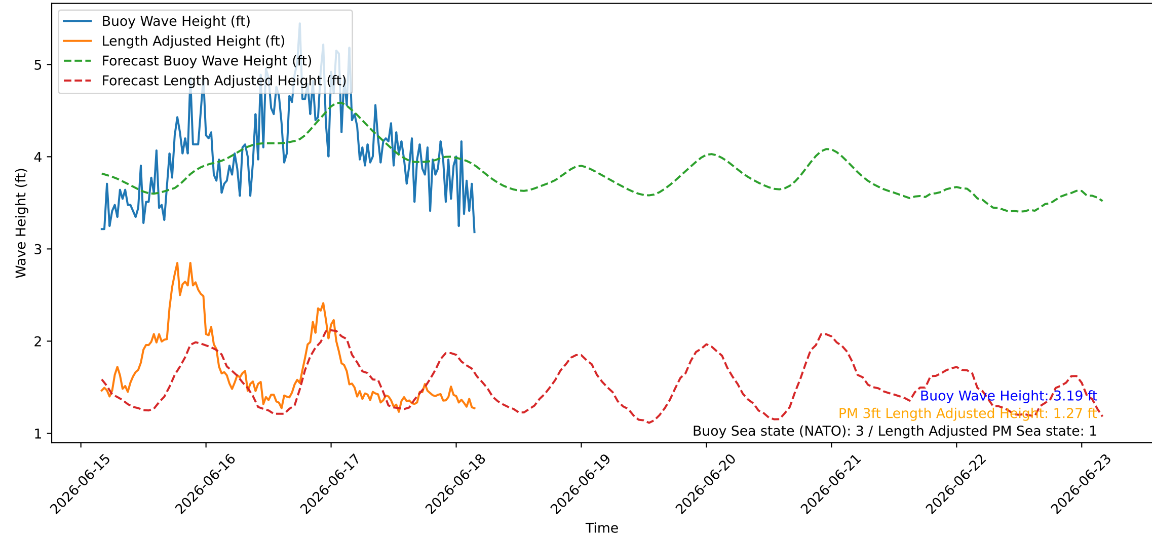
Wave Heights over Time for Oceanside Harbor at 2026-06-18 04:10:26
