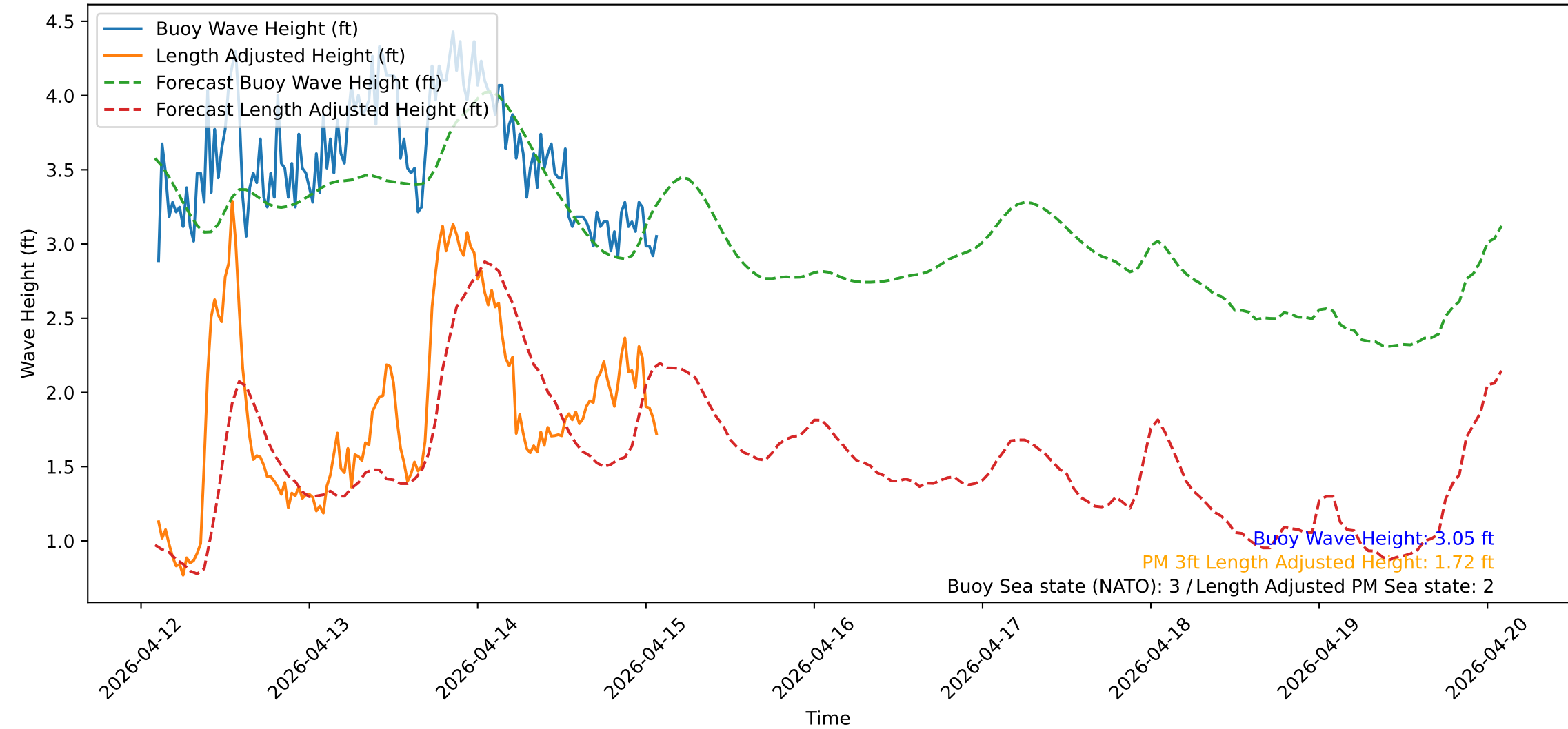
Wave Heights over Time for Red Beach at 2026-04-15 02:20:51
