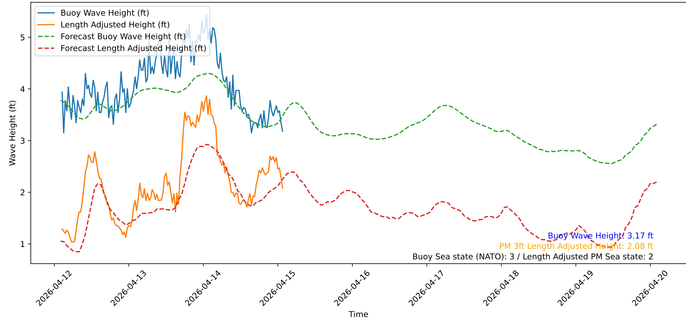
Wave Heights over Time for Oceanside Harbor at 2026-04-15 02:20:31
