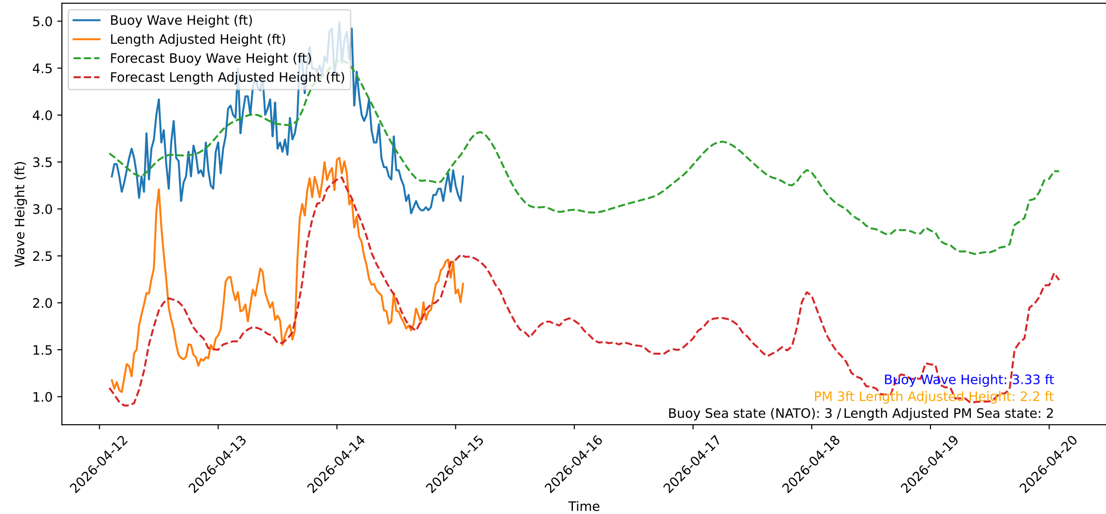
Wave Heights over Time for Green Beach at 2026-04-15 02:21:13
