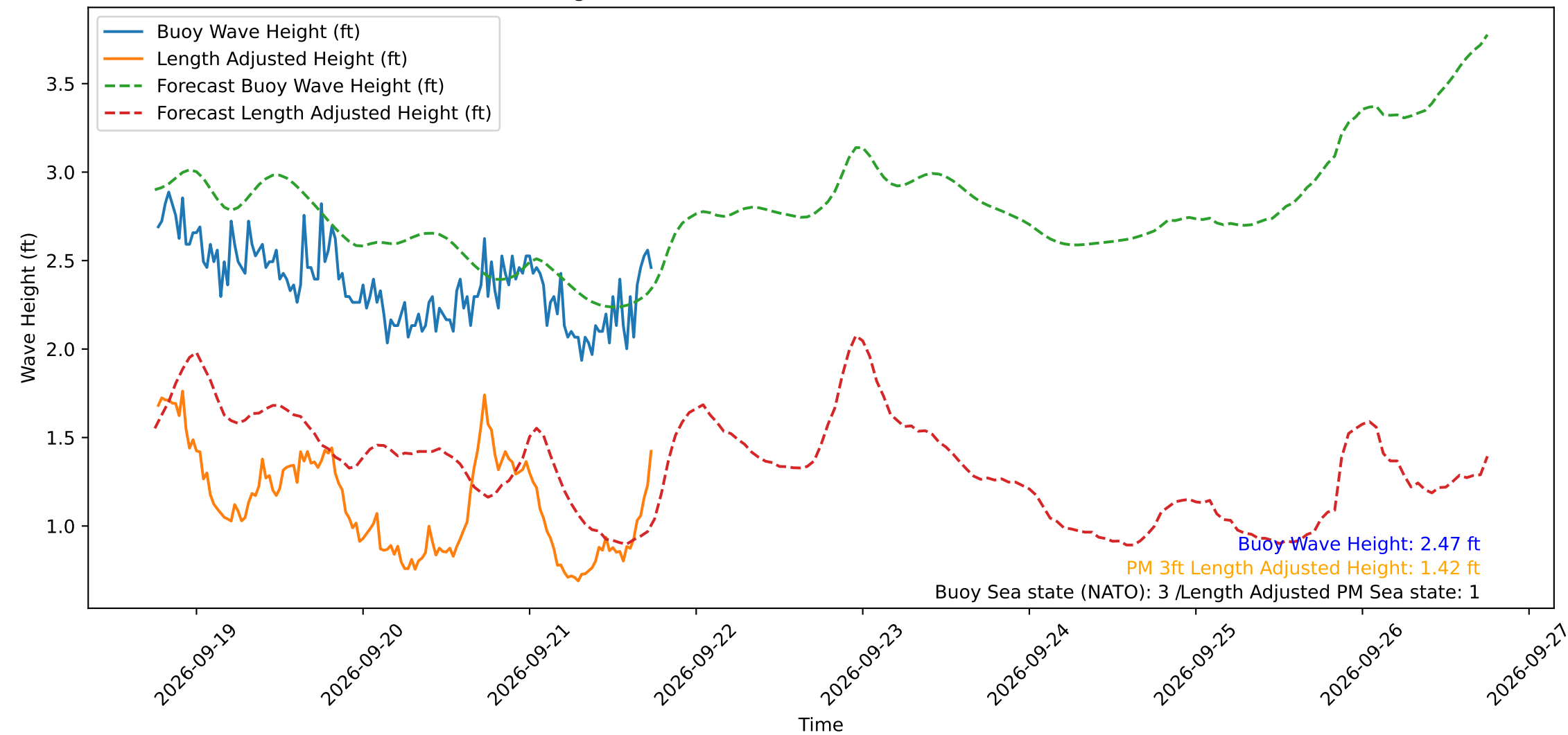
Wave Heights over Time for Red Beach at 2026-09-21 18:20:50
