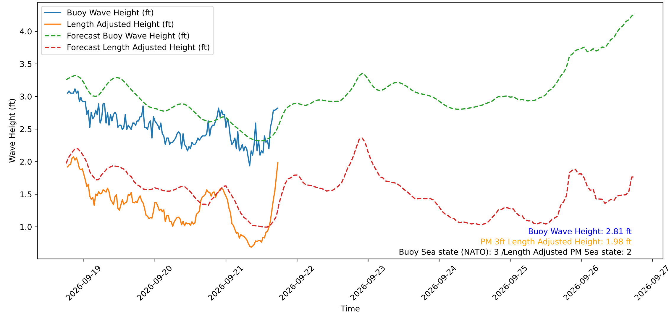
Wave Heights over Time for Green Beach at 2026-09-21 18:21:14
