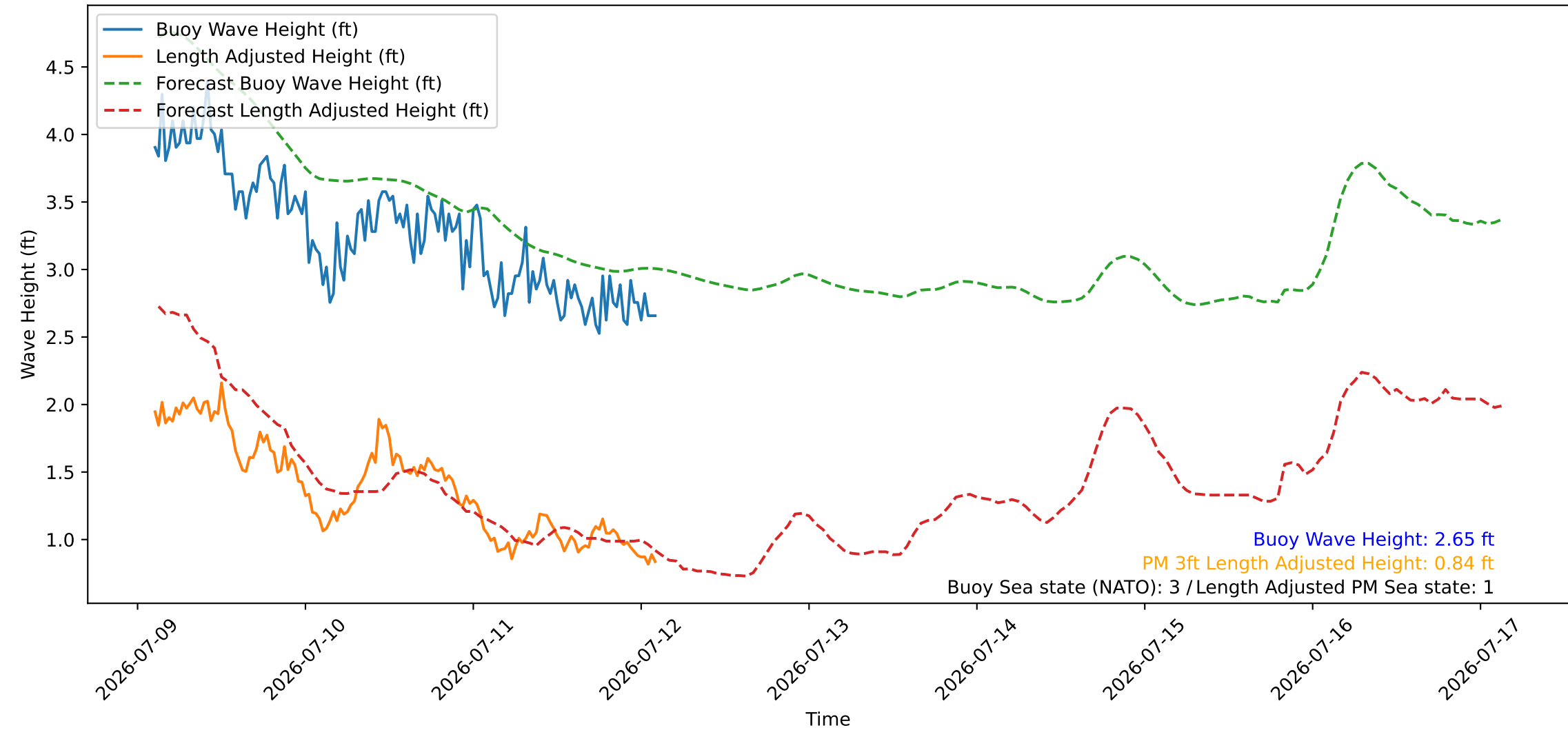
Wave Heights over Time for Green Beach at 2026-07-12 02:41:09
