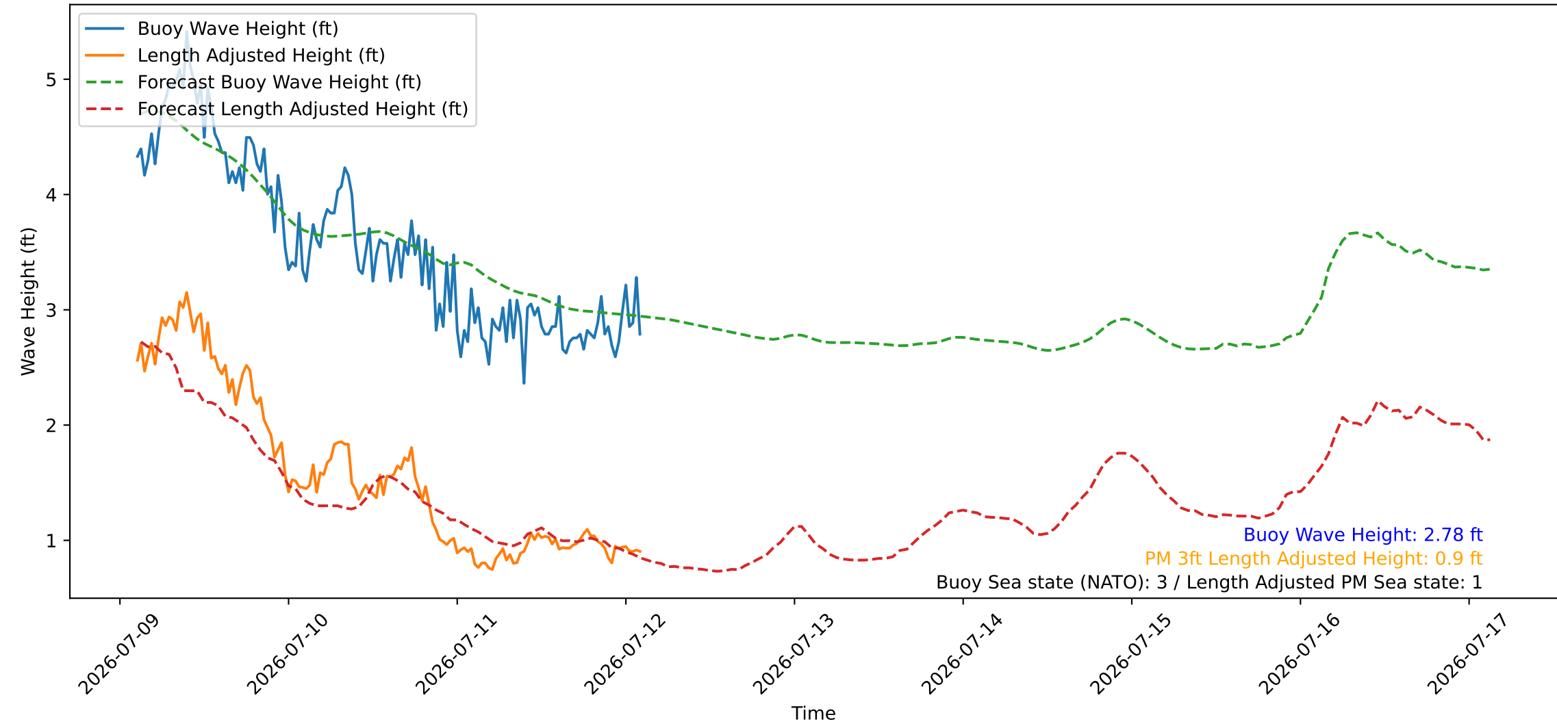
Wave Heights over Time for Oceanside Harbor at 2026-07-12 02:40:26
