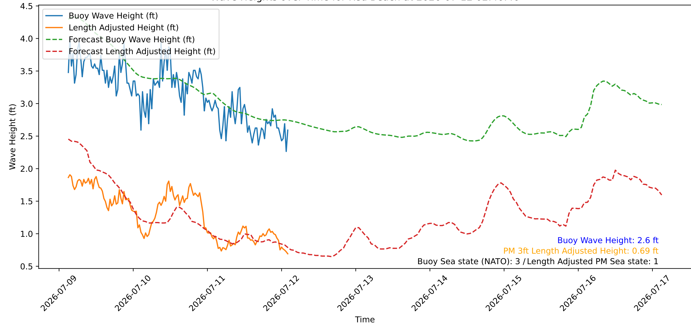
Wave Heights over Time for Red Beach at 2026-07-12 02:40:46
