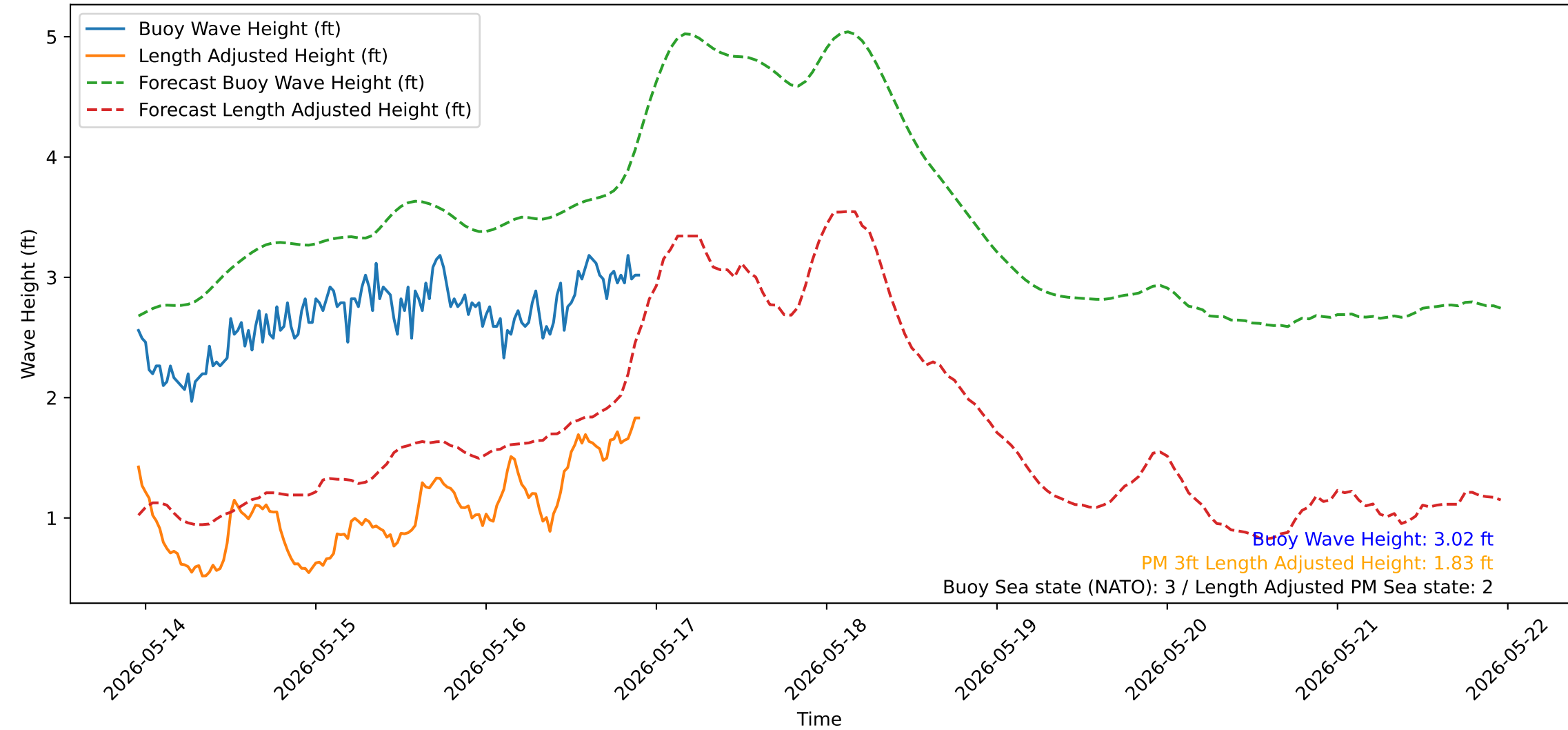
Wave Heights over Time for Red Beach at 2026-05-16 22:30:51
