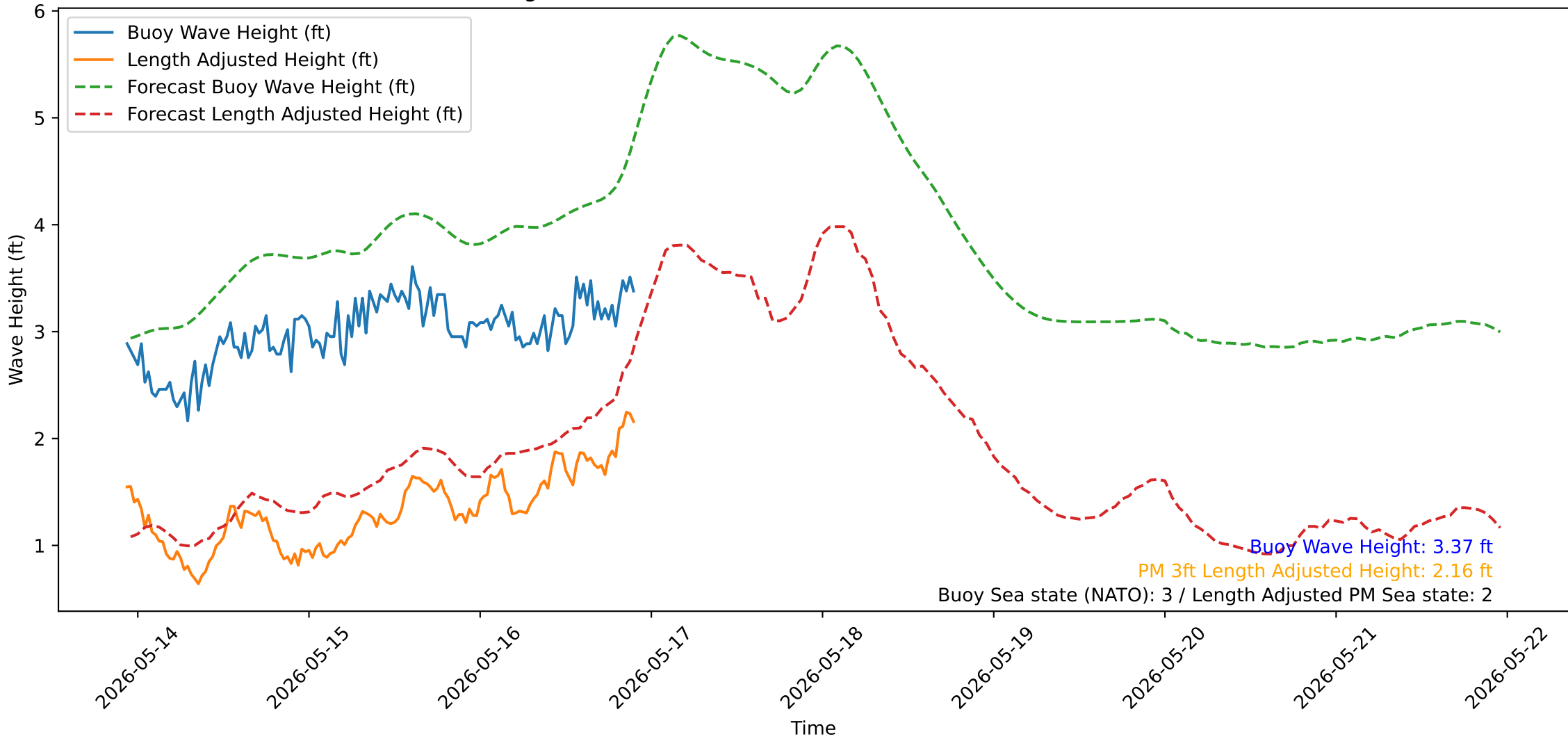
Wave Heights over Time for Oceanside Harbor at 2026-05-16 22:30:31
