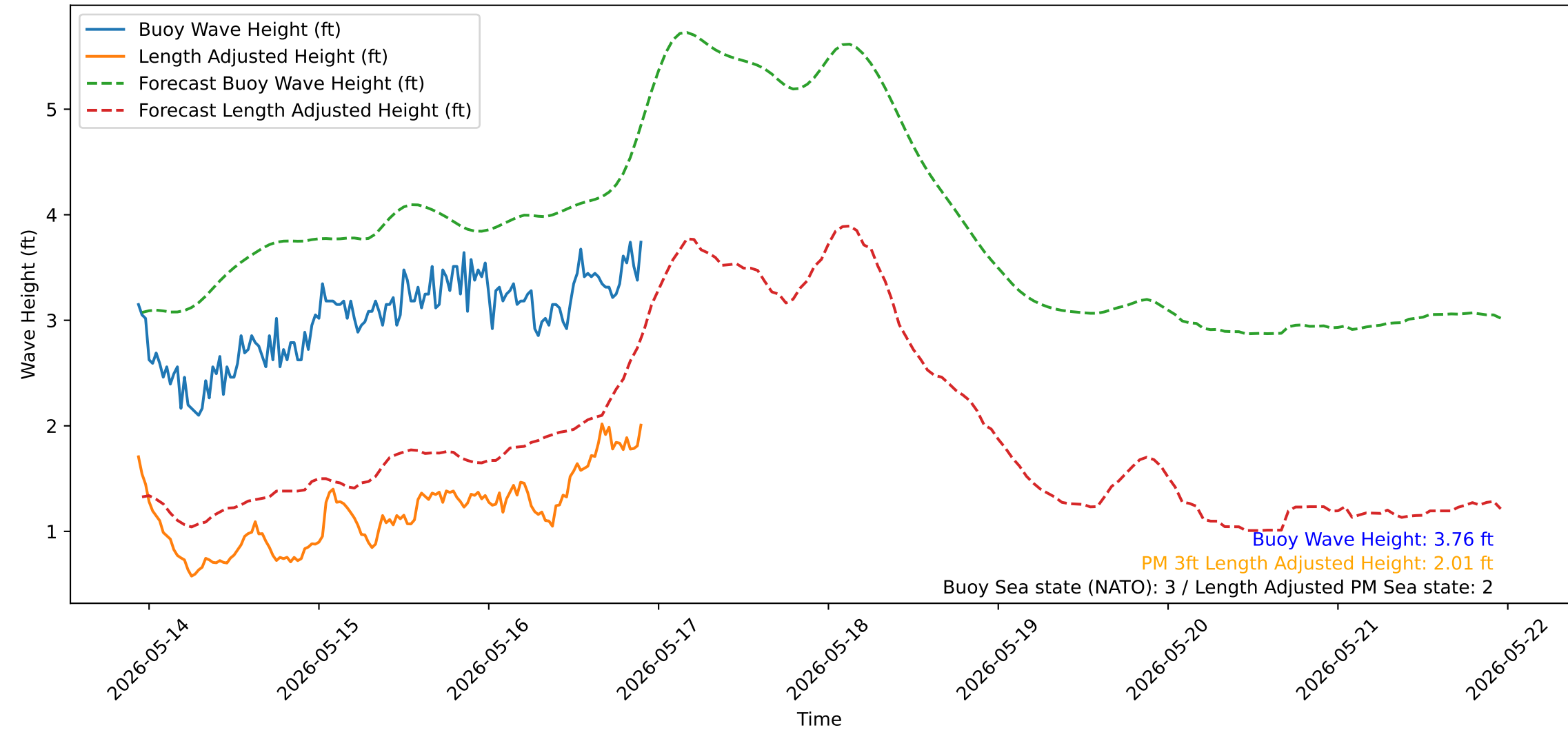
Wave Heights over Time for Green Beach at 2026-05-16 22:31:13
