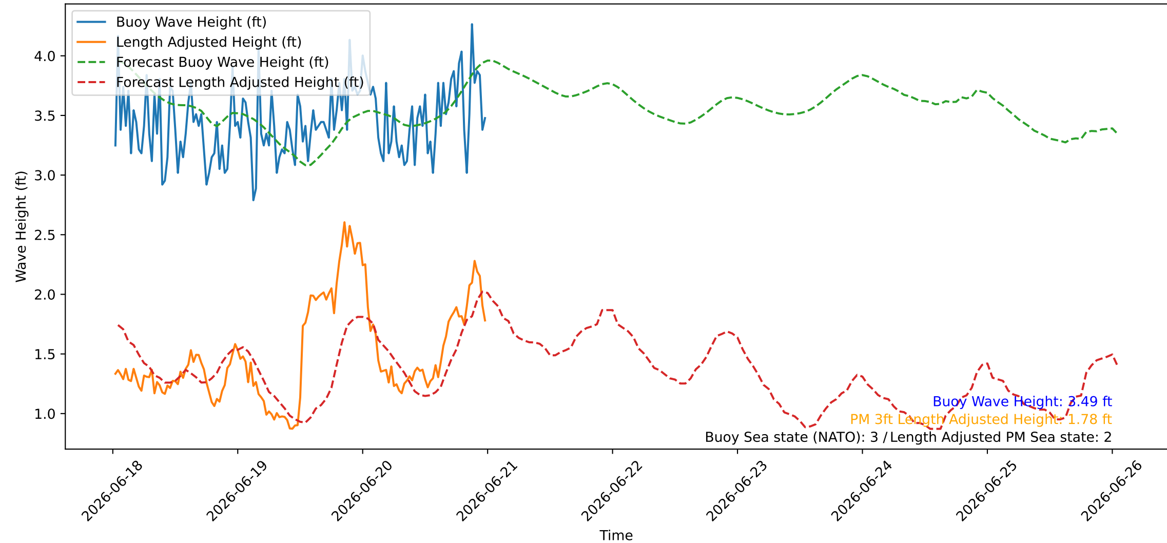
Wave Heights over Time for Oceanside Harbor at 2026-06-21 00:30:26
