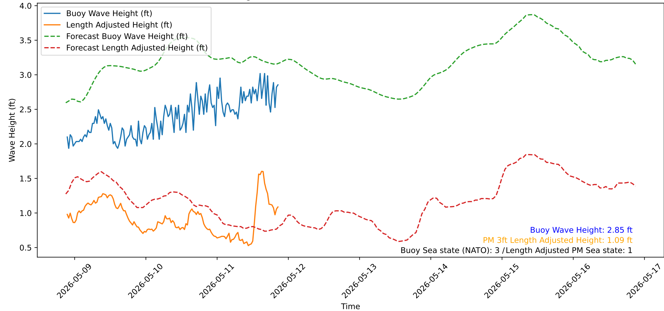
Wave Heights over Time for Red Beach at 2026-05-11 21:20:52
