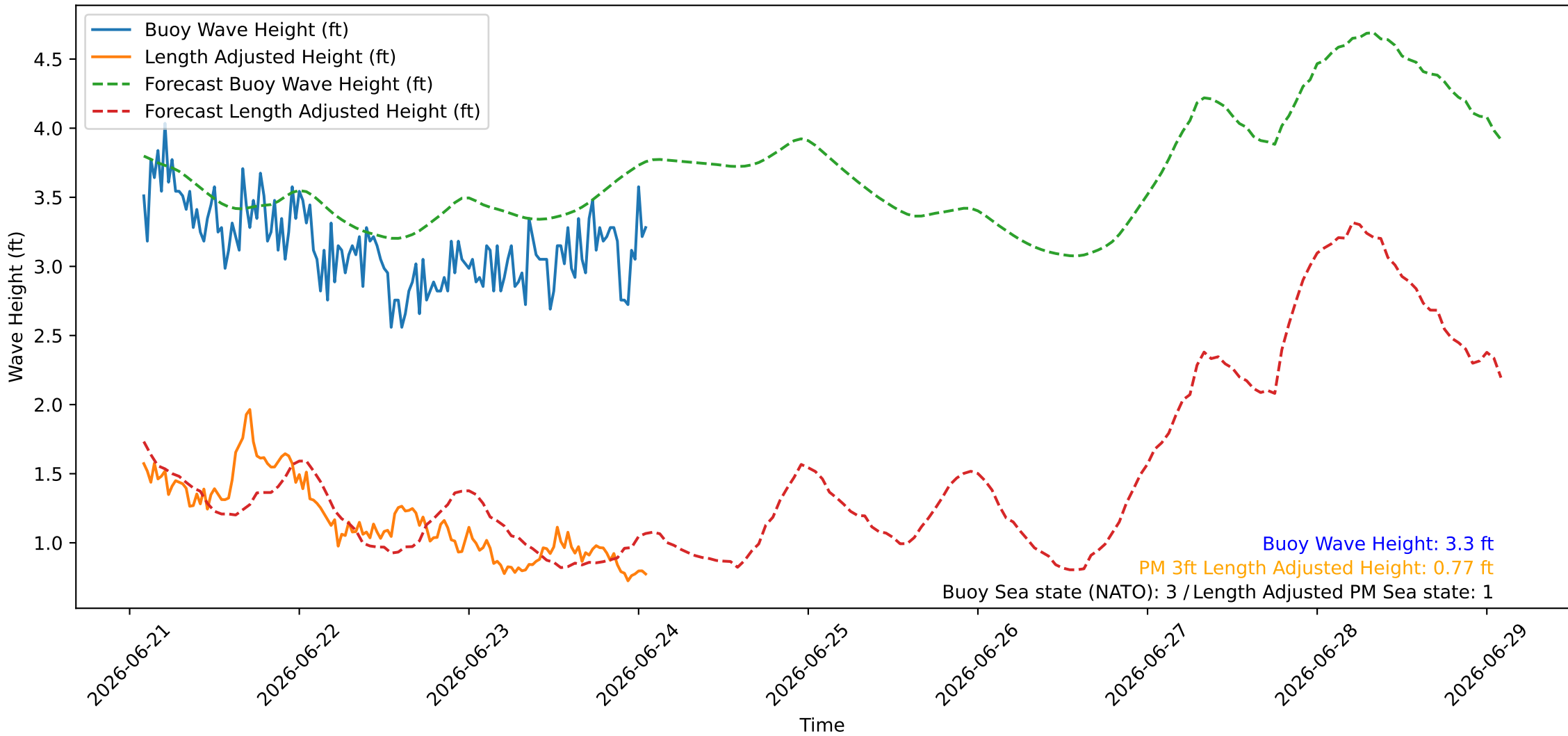
Wave Heights over Time for Oceanside Harbor at 2026-06-24 01:50:26
