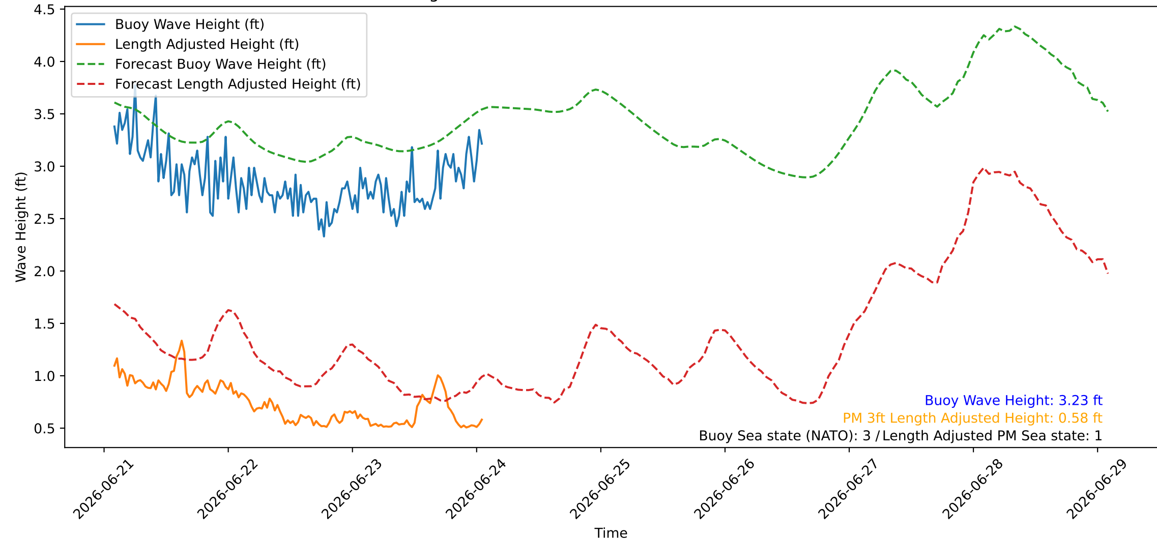
Wave Heights over Time for Red Beach at 2026-06-24 01:50:47
