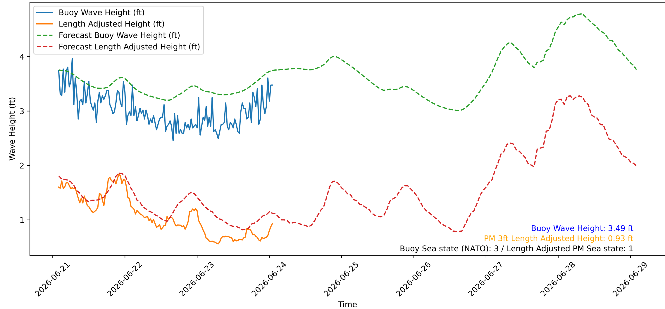
Wave Heights over Time for Green Beach at 2026-06-24 01:51:09
