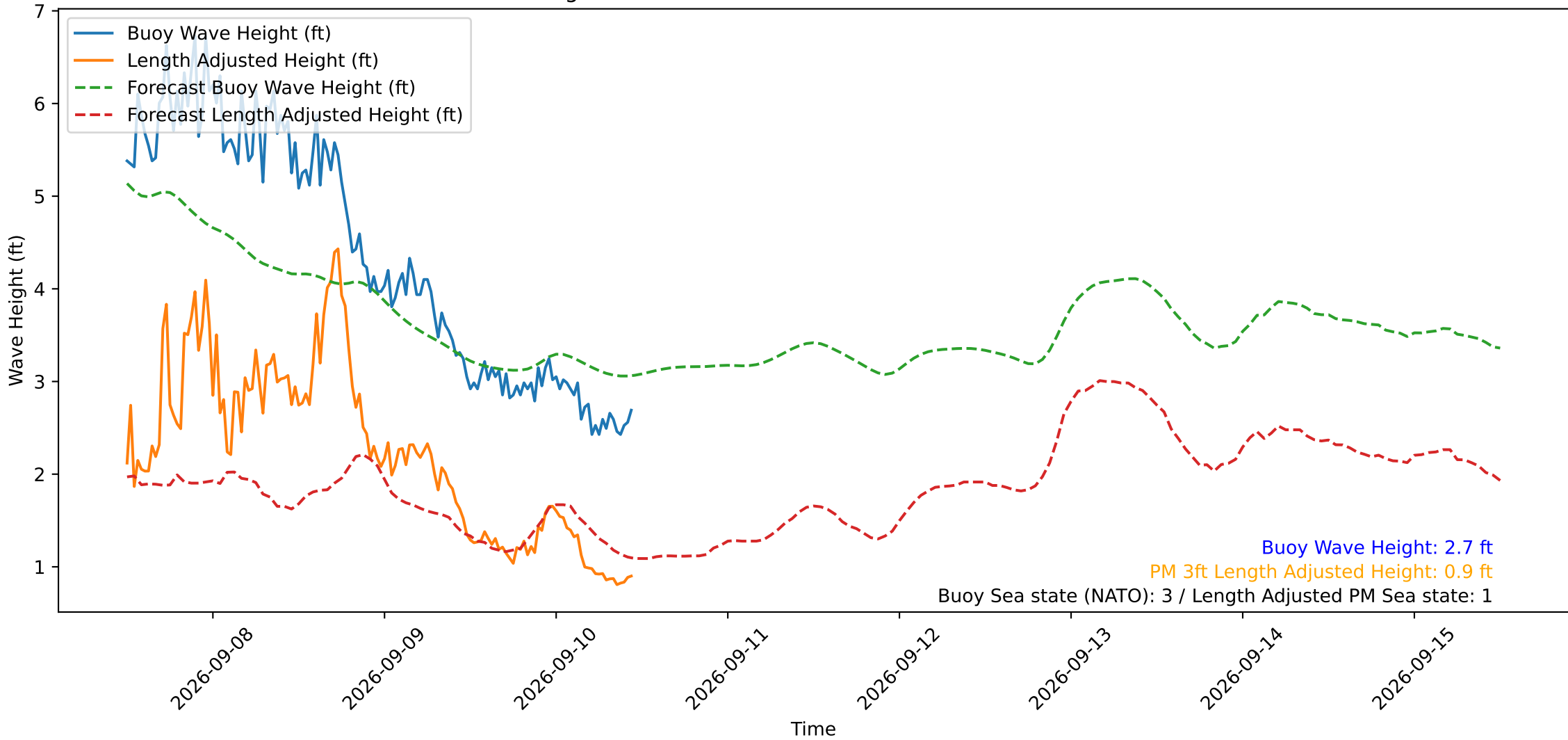
Wave Heights over Time for Red Beach at 2026-09-10 11:30:49
