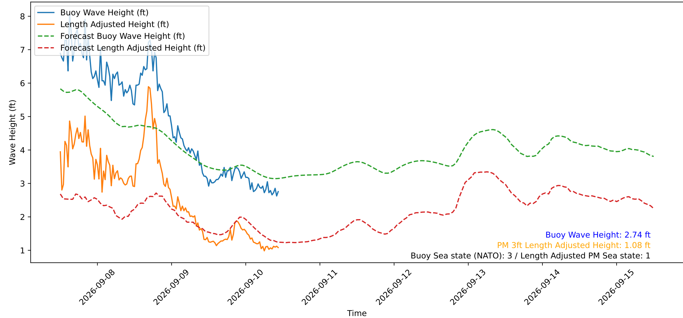
Wave Heights over Time for Green Beach at 2026-09-10 11:31:12
