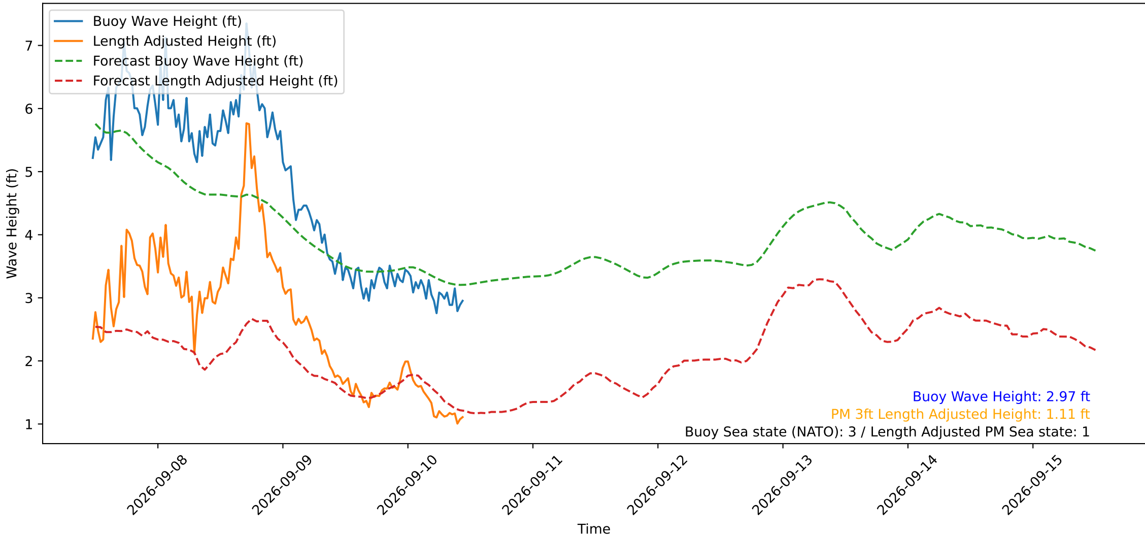
Wave Heights over Time for Oceanside Harbor at 2026-09-10 11:30:29
